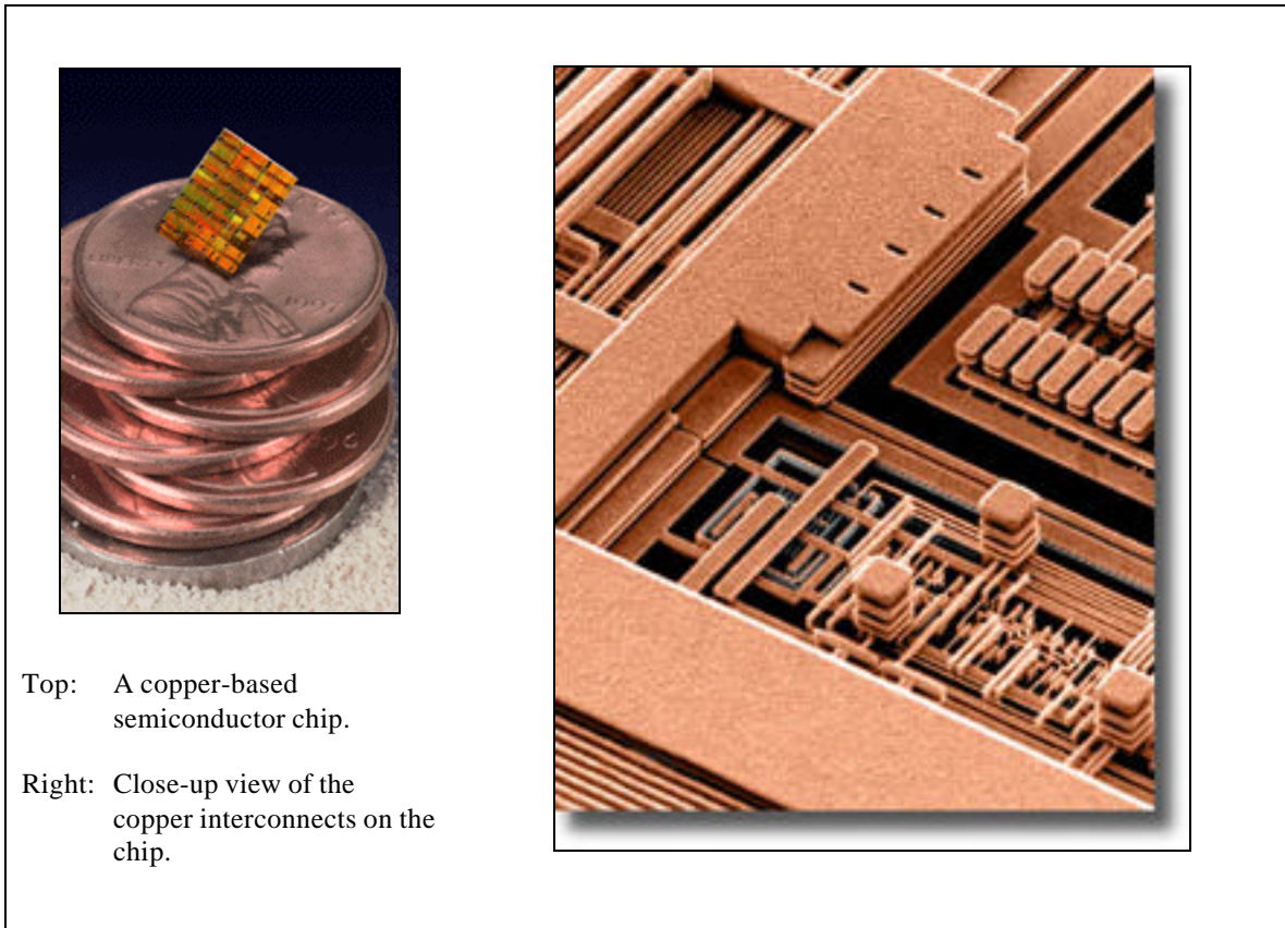
Figure 2-1: Semiconductor Chip with Copper Interconnects.
