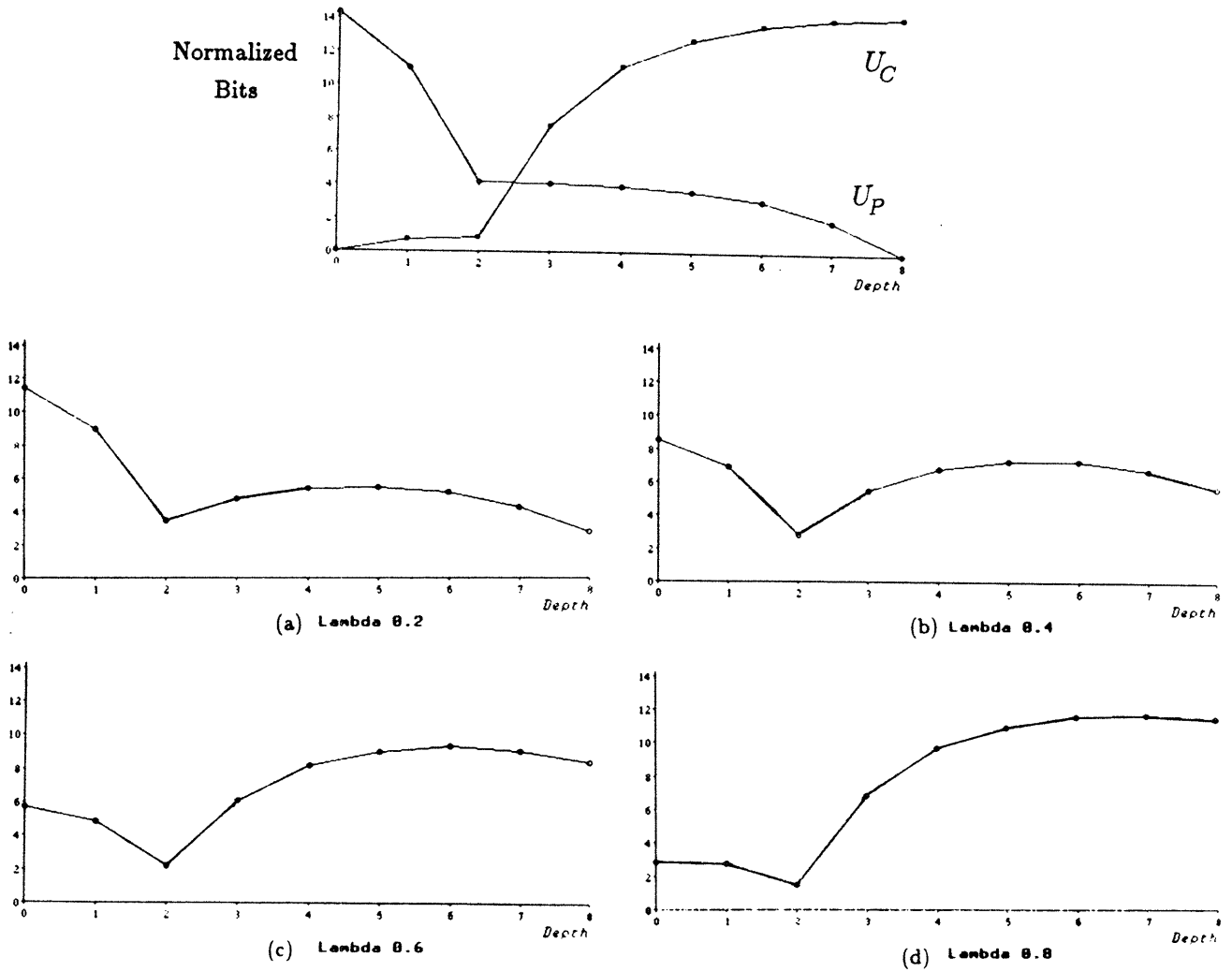
Figure 4.18: Graphs of U = (1 - \lambda) U_P + \lambda \eta U_C for the ordered taxonomy. Top plot is original values of U_P and normalized U_C . The four panels a-d are for \lambda of .2, .4, .6, and .8 respectively.
