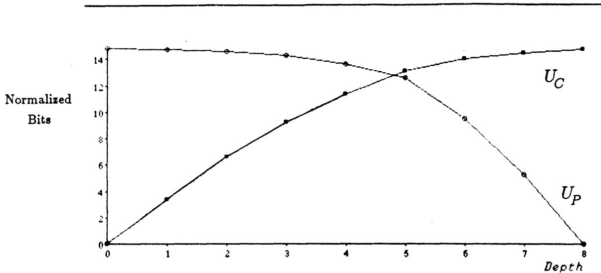
Figure 4.13: The evaluation curves for the jumbled taxonomy. Plotted are U_P and the normalized U_C as a function depth. The normalization factor causes the scales of the two graphs to be the same. Both curves change smoothly, indicating no special level within the taxonomy.
