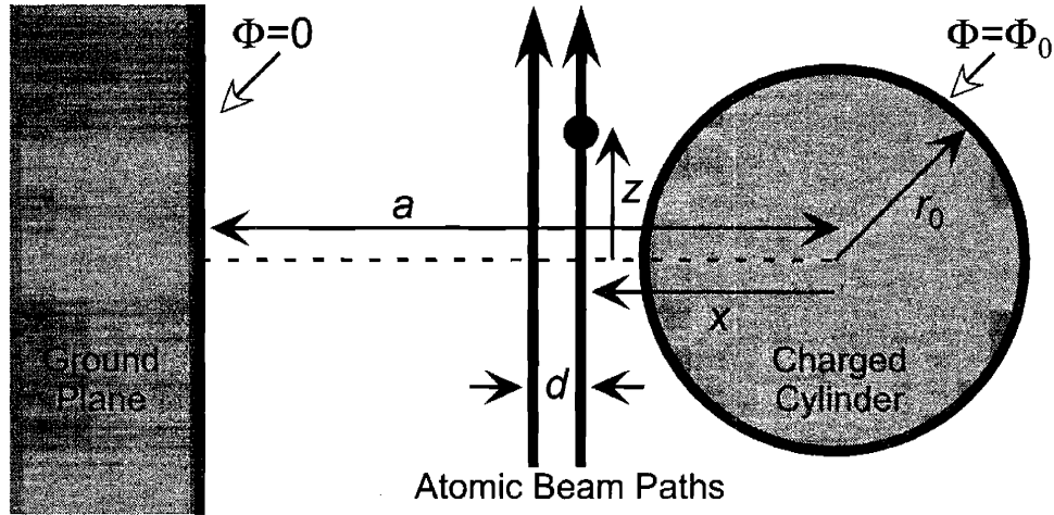
Figure 3-3: A charged cylinder is used to apply a differential phase shift to the separated paths of the wavefunction inside the interferometer.
