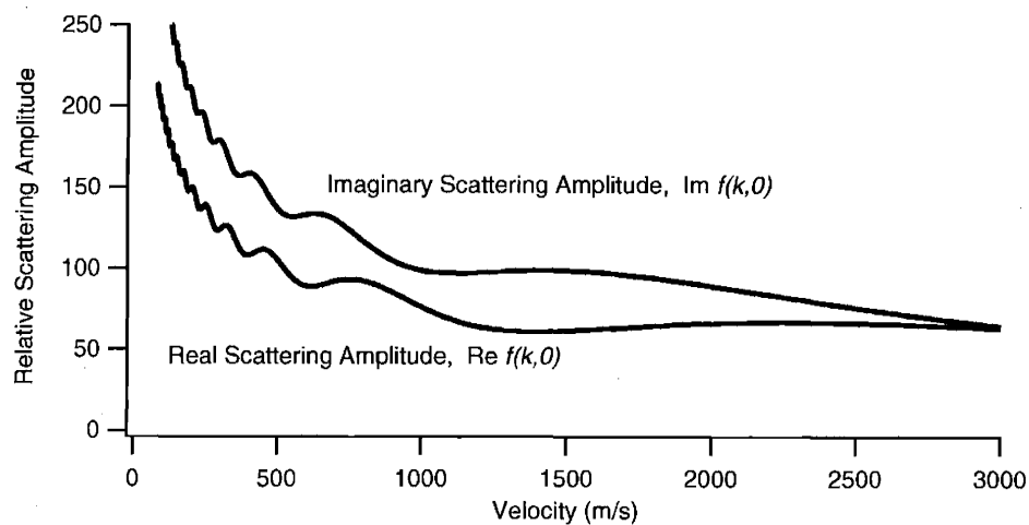
Figure 2-3: \text{Re}f(k) and \text{Im}f(k) for a sodium-argon Lennard-Jones potential, plotted vs the velocity, v = \hbar k/m .
