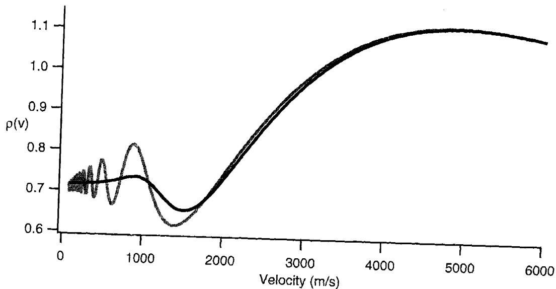
Figure 2-5: A comparison of thermally averaged ratio \rho(v) = \text{Re}[n(v) - 1]/\text{Im}[n(v)] for a sodium-argon 6-12 potential at T = 0^\circ\text{K} (grey), and at T = 300^\circ\text{K} (black). In the limit of zero temperature, \rho is equivalent to \text{Re}f/\text{Im}f .
