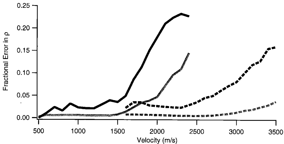
Figure 2-22: The fractional systematic error in the measurement of \rho due to wrong interfering orders, as a function of velocity for the 200 nm (—) and 100 nm (- - -) interferometers. Although the attenuated orders (black) are larger than the unattenuated ones (grey) to start with (see Fig. 2-21), they influence the measurement of \rho less because during the measurement they are greatly attenuated.
