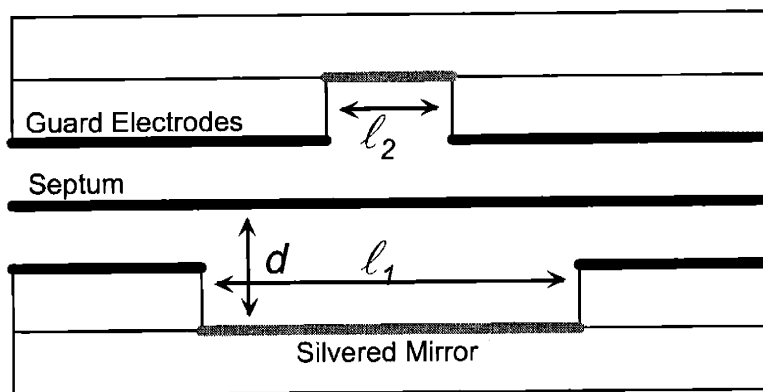
Figure 3-16: Schematic showing the new features of an improved interaction region. Black surfaces are at ground and grey surfaces are at high voltage. The septum has been made much longer than \ell and the guard electrodes have been extended. The high voltage plane consists of a charged, partially-silvered surface that can transmit light for an interferometric measurement of d . The ground side of the interaction region has a small length that is at high voltage to cancel out the hard-to-model end effects. (The schematic exaggerates the vertical dimensions; in reality d \ll \ell .)
