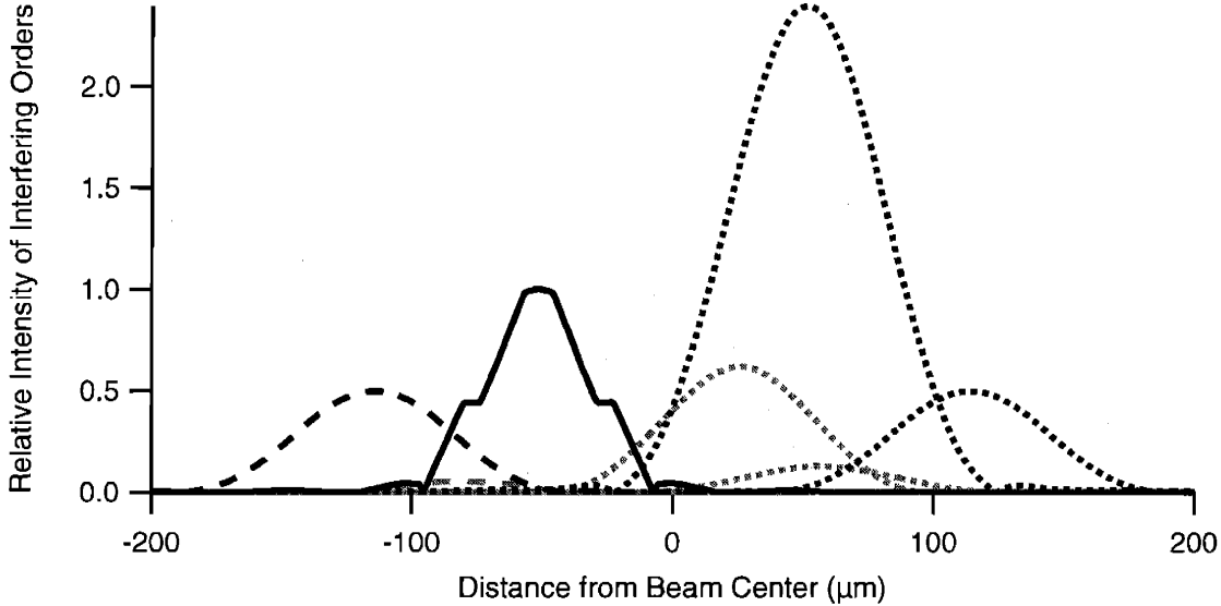
Figure 2-20: Intensities of “wrong” interfering orders ( \cdots ), ( - - - ) compared to the “normal” order ( --- ), this time including the effects of clipping by the septum (molecule orders are in grey). This example models the worst case of contamination experienced during our measurements: v = 1 km/s, 200 nm gratings. The “normal” intensity is greatly reduced due to clipping by the septum.
