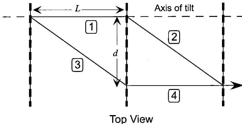
Figure 1-7: An interferometer tilted with respect to gravity experiences a phase shift. The maximum separation between the interferometer paths is d = \frac{hL}{mv\lambda_g}
