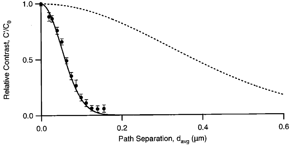
Figure B-4: A comparison of the length scales for decoherence by photon scatter and a fixed momentum kick. The data show the contrast dependence when scattering multiple photons. The dashed line shows contrast for the first order of the diffraction grating from the fit of the data in Fig. B-3.
