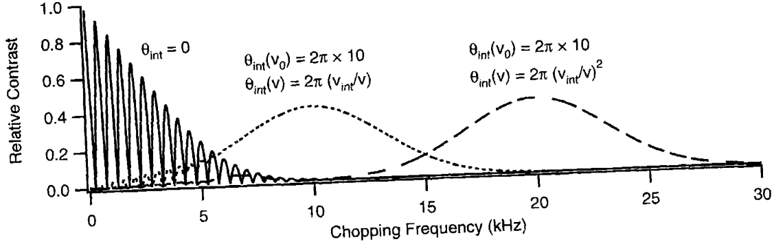
Figure 3-6: The contrast (from Eq. 3.35) vs the chopping frequency f \equiv \omega/2\pi assuming v_0 = 1 km/s, L = 1 m, and \sigma/v_0 = 5\% . Three cases are shown: no interaction phase (—); a 1/v -dependent interaction phase like that produced by a high voltage septum ( \cdots ); and a 1/v^2 -dependent interaction phase like an electric field gradient (---). Note that the mean phase applied is the same for both interactions ( 2\pi \times 10 radians), but the revivals occur at different frequencies. For the larger frequency revival, higher order revivals can be seen (though barely) at multiples \frac{1}{3}, \frac{1}{5}, \dots of the rephasing frequency.
