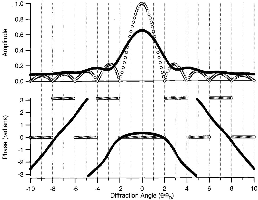
Figure C-4: Diffraction of sodium atoms from a 50 nm wide slit, in the presence of the Van der Waals potential (●) and without (○). The single slit diffraction is the envelope of the grating diffraction pattern, consisting of peaks spaced \theta_D apart. A transit time in the slit of 10 ns and a grating period of 100 nm is assumed.
