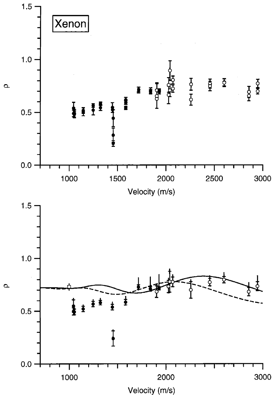
Figure 2-9: The ratio of real to imaginary index of refraction, \rho , for sodium atoms with velocity v in Xe. Top: Each measurement is taken at a different pressure and velocity ( \bullet using 200 nm gratings, \circ 100 nm). Bottom: All measurements at a single velocity are averaged and systematic error bars are included. A comparison is made with theoretical predictions, [6](—), [31](---), [13](···), and an older measurement [83](□).
