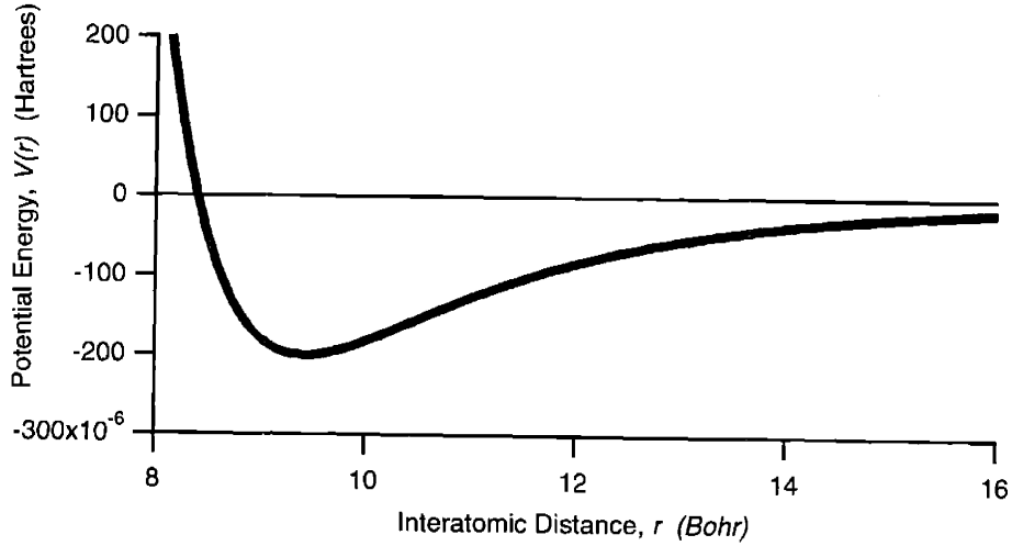
Figure 2-2: The Lennard-Jones 6-12 potential is the simplest model for the interatomic potential between sodium and argon. The depth of the potential is D_e = 2.0 \times 10^{-4} \text{ H} = 5.4 \times 10^{-3} \text{ eV} . The minimum occurs at r_e = 9.4 a_0 = 5.0 \text{ \AA} [17].
