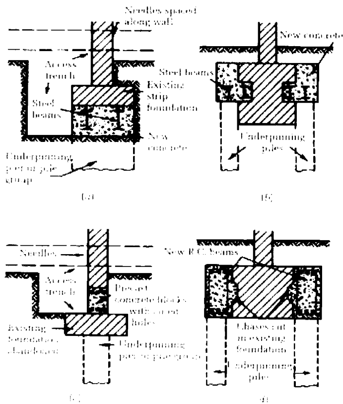
Figure 12 Methods of Underpinning Wall Foundations Using Beams Spanning Between Piles [10]
