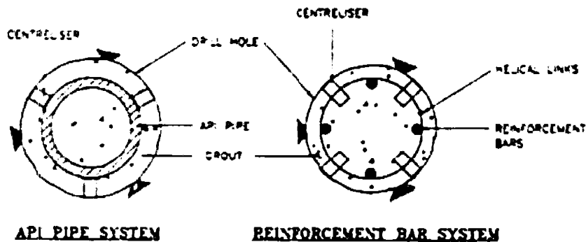
Figure 13 Typical Cross Sections of Two Common Micropile System [5]
