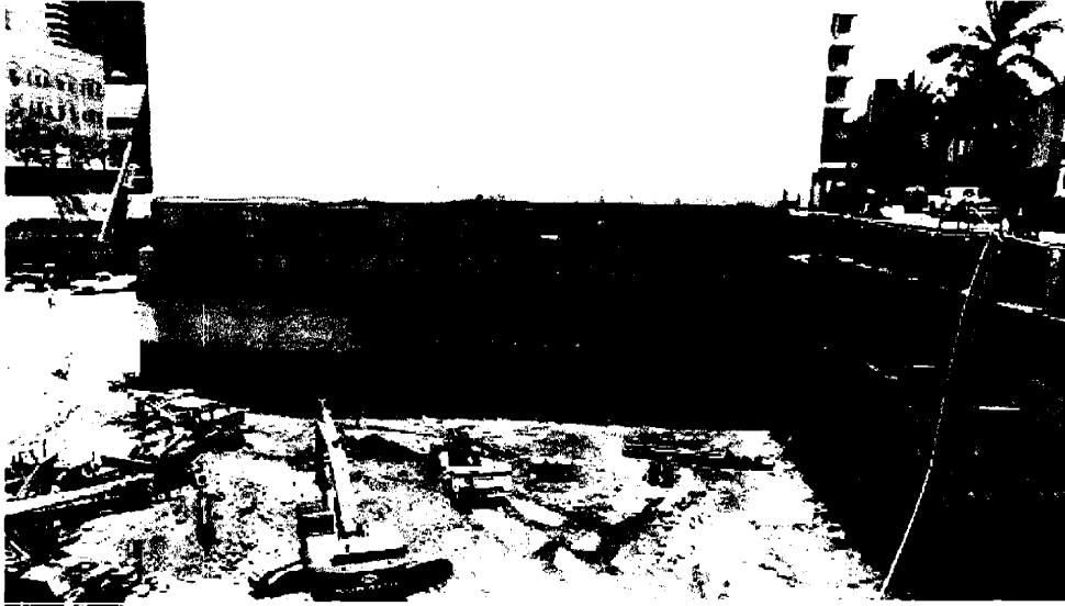
Figure 18 General View of Excavation Works, Honolulu [15]
