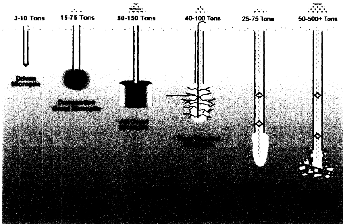
Figure 9 General Types of Micropiles [4]
