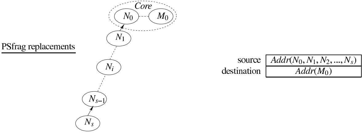
Figure 5-21: A hill route segment without a downhill portion and its representation.
