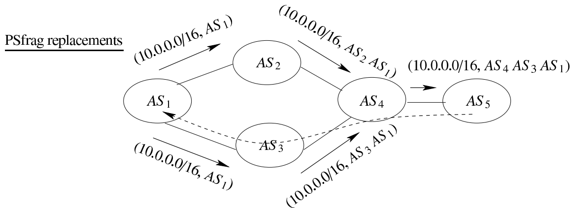
Figure 2-1: This figure illustrates how BGP works. A domain AS_1 announces (10.0.0.0/16, AS_1) to its neighbors AS_2 and AS_3 , telling them that it can reach the address prefix 10.0.0.0/16 . AS_2 and AS_3 propagate this reachability information by announcing (10.0.0.0/16, AS_2 AS_1) and (10.0.0.0/16, AS_3 AS_1) respectively to their neighbor AS_4 . From these announcements, AS_4 learns that it has two paths AS_4 \rightarrow AS_3 \rightarrow AS_1 and AS_4 \rightarrow AS_2 \rightarrow AS_1 to reach the address prefix 10.0.0.0/16 . Based on its policies, AS_4 selects the path AS_4 \rightarrow AS_3 \rightarrow AS_1 and announces (10.0.0.0/16, AS_4 AS_3 AS_1) to AS_5 . Packets sent from AS_5 to the address range 10.0.0.0/16 will then follow the path AS_5 \rightarrow AS_4 \rightarrow AS_3 \rightarrow AS_1 .
