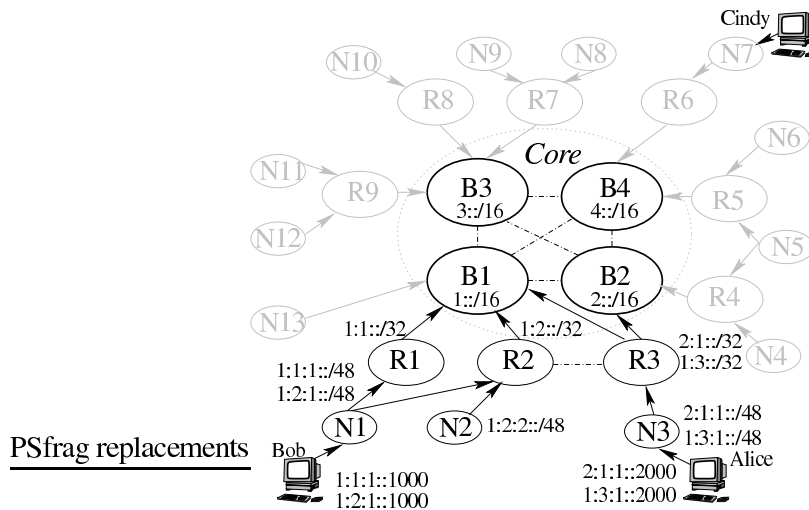
Figure 4-3: An example of strict provider-rooted hierarchical addressing. For clarity, we only shown address allocation for the dark region of the figure.
