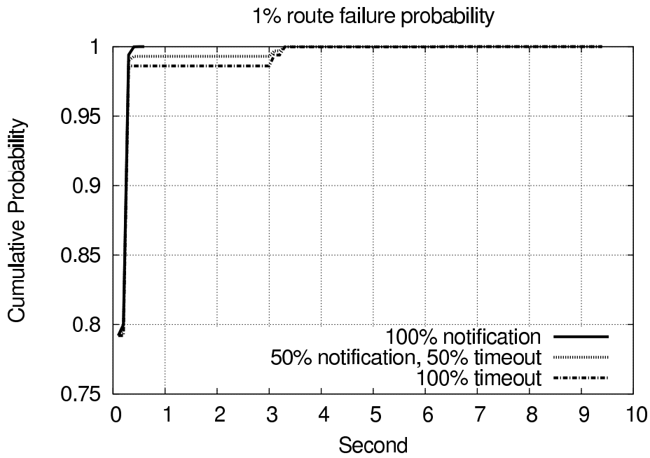
Figure 7-12: The cumulative distribution of the connection setup latency with 1% route failure probability. Other parameter values: 80% NURLS cache hit probability, 3-level of name hierarchy, 100ms round trip time, 3-second timeout value for route failure detection.
