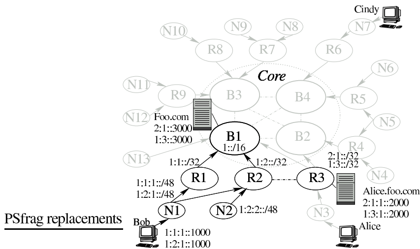
Figure 4-8: When Bob wants to communicate with Alice, Bob will query the Name-to-Route Lookup Service to retrieve Alice's addresses, 2:1:1::2000 and 1:3:1::2000.
