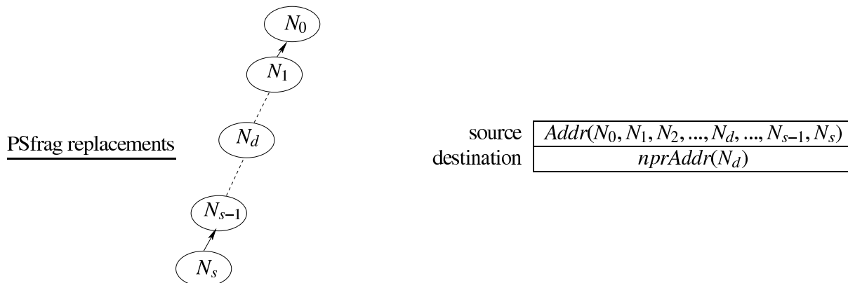
Figure 5-16: This figure shows an uphill route segment and its representation.
