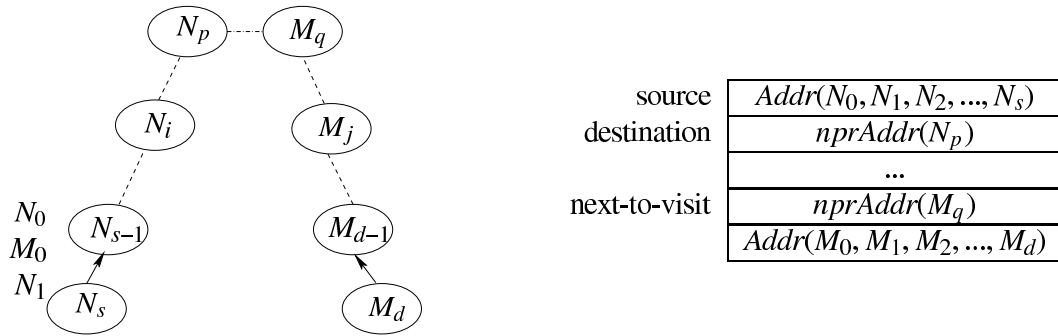
Figure 5-22: This figure shows an arbitrary route segment and its representation.
