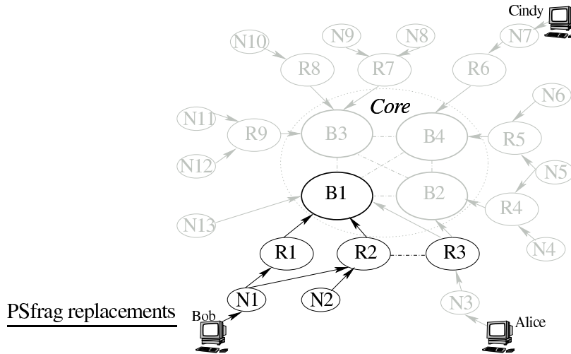
Figure 3-2: User Bob's up-graph is drawn with dark lines.
