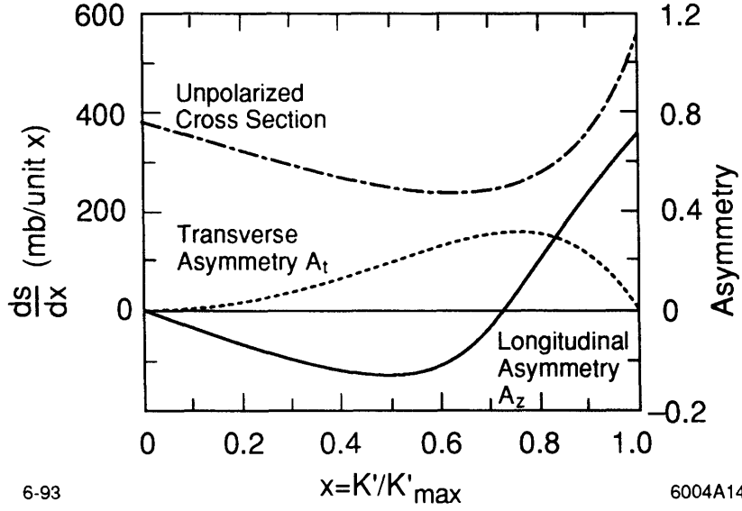
Figure 4-2: The transverse and longitudinal asymmetries for Compton scattering as a function of the kinematical variable x . x = 1 for the case of complete backscattering (kinematic edge).
