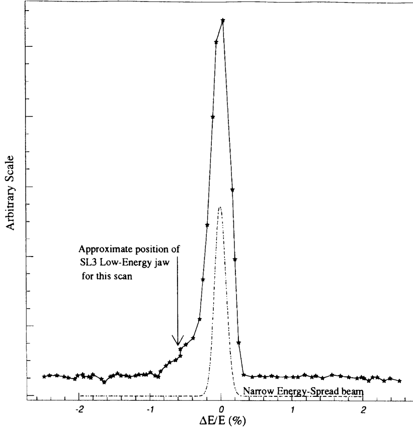
Figure 7-3: Final Focus wirescan data, showing \mathcal{N}(E) (stars), and the position of the SL3 Low-Energy collimator jaw for this scan (arrow); as well as the narrow-energy spread test beam ( < 0.1\% ) distribution, (dashes).
