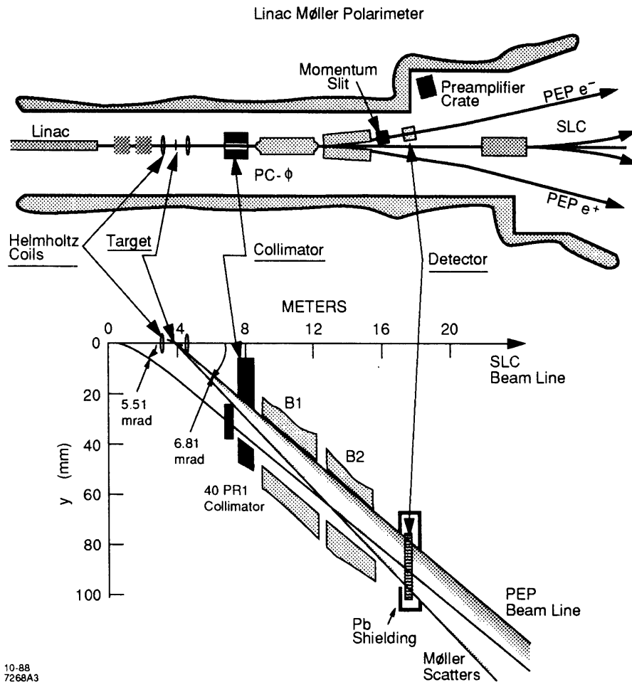
Figure B-1: Schematic of the Linac Møller Polarimeter.
