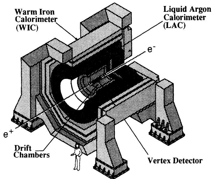
Figure 3-1: A perspective, cutaway diagram of the SLD detector at the SLC.
