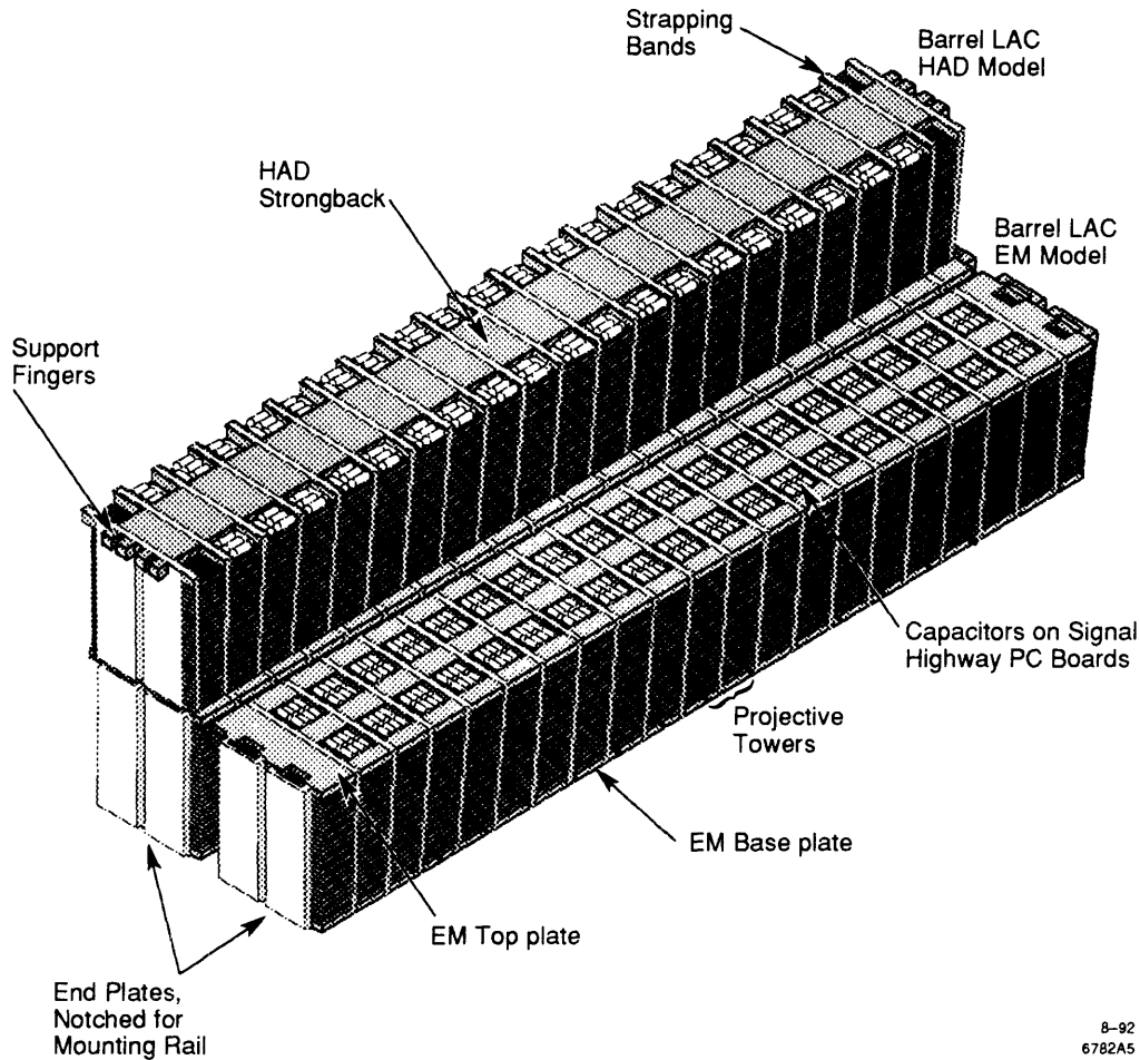
Figure 3-3: Schematic diagram of a LAC module. The inner EM sections and the outer HAD sections are shown.
