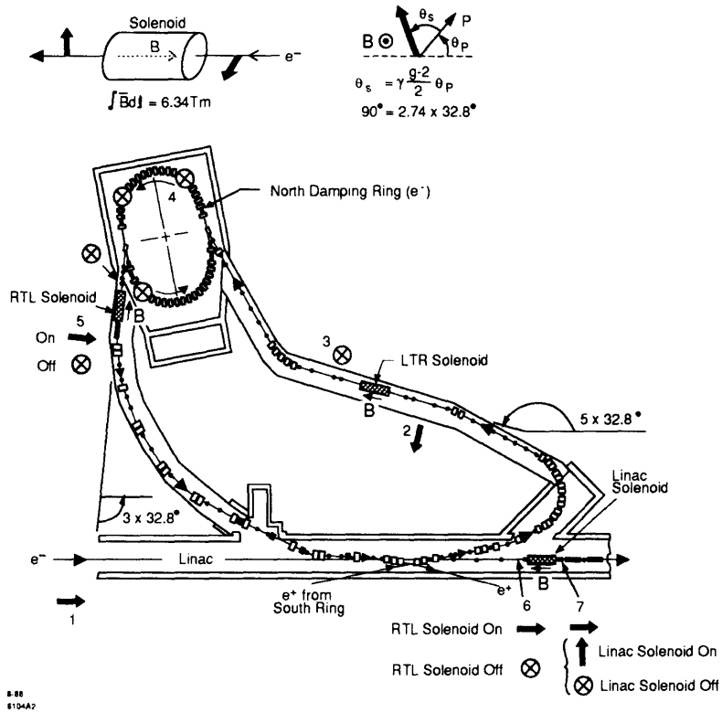
Figure 2-5: The North Damping Ring. The orientation of the electron spin vector is indicated throughout.
