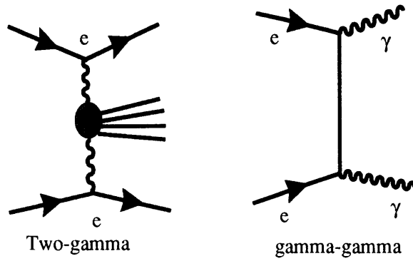
Figure 8-15: Feynman diagrams for 2- \gamma and \gamma\gamma backgrounds.
