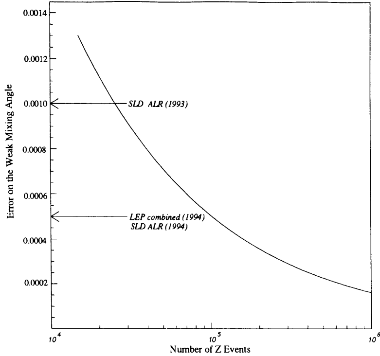
Figure 10-1: Error on \sin^2 \theta_W^{\text{eff}} versus number of Z events at 80% e^- beam polarization, and \delta\mathcal{P}/\mathcal{P} = 1\% .
