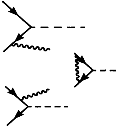
Figure 1-2: Feynman diagrams for first-order initial state radiation correction terms for the interaction e^+e^- - Z .
