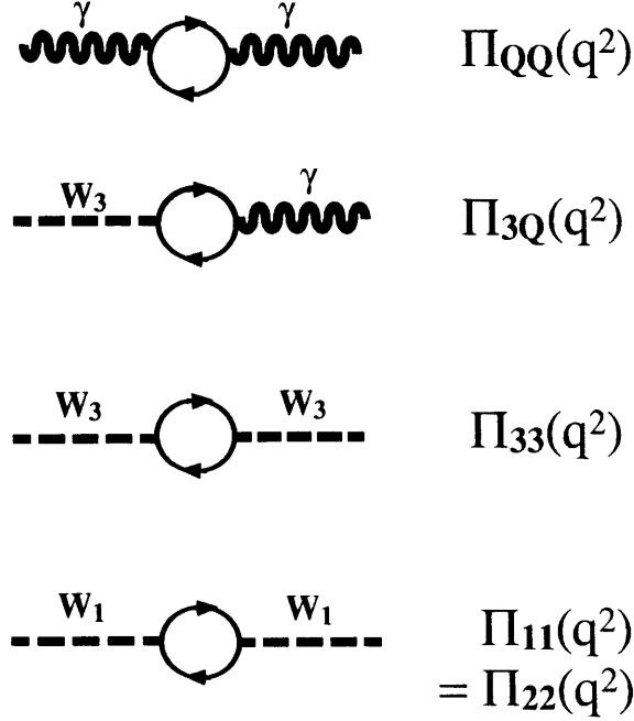
Figure A-1: Oblique corrections and their dependence on the \Pi functions.
