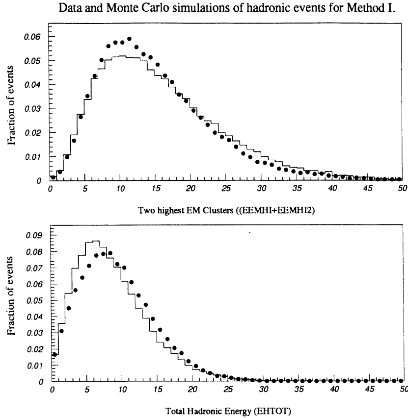
Figure 8-9: Comparison of the Method I variables EEMHI1+EEMHI2 and EHTOT for the Pass 2 hadronic sample data (dots) and hadronic event simulation (line).
