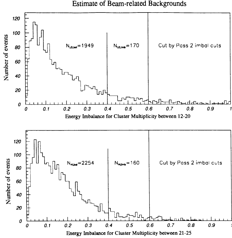
Figure 8-13: Histograms of energy imbalance for the low and high cluster multiplicity data sets.
