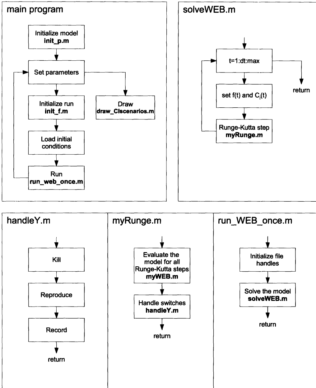
Figure 3-2: Flowchart of the main steps in the simulations.
