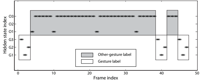
Figure 2. This figure shows max-margin assignment of hidden states given by the LDCRF model for a sample sequence from the synthetic data set. As we can see the model has used the hidden states to learn the internal sub-structure of the gesture class.
