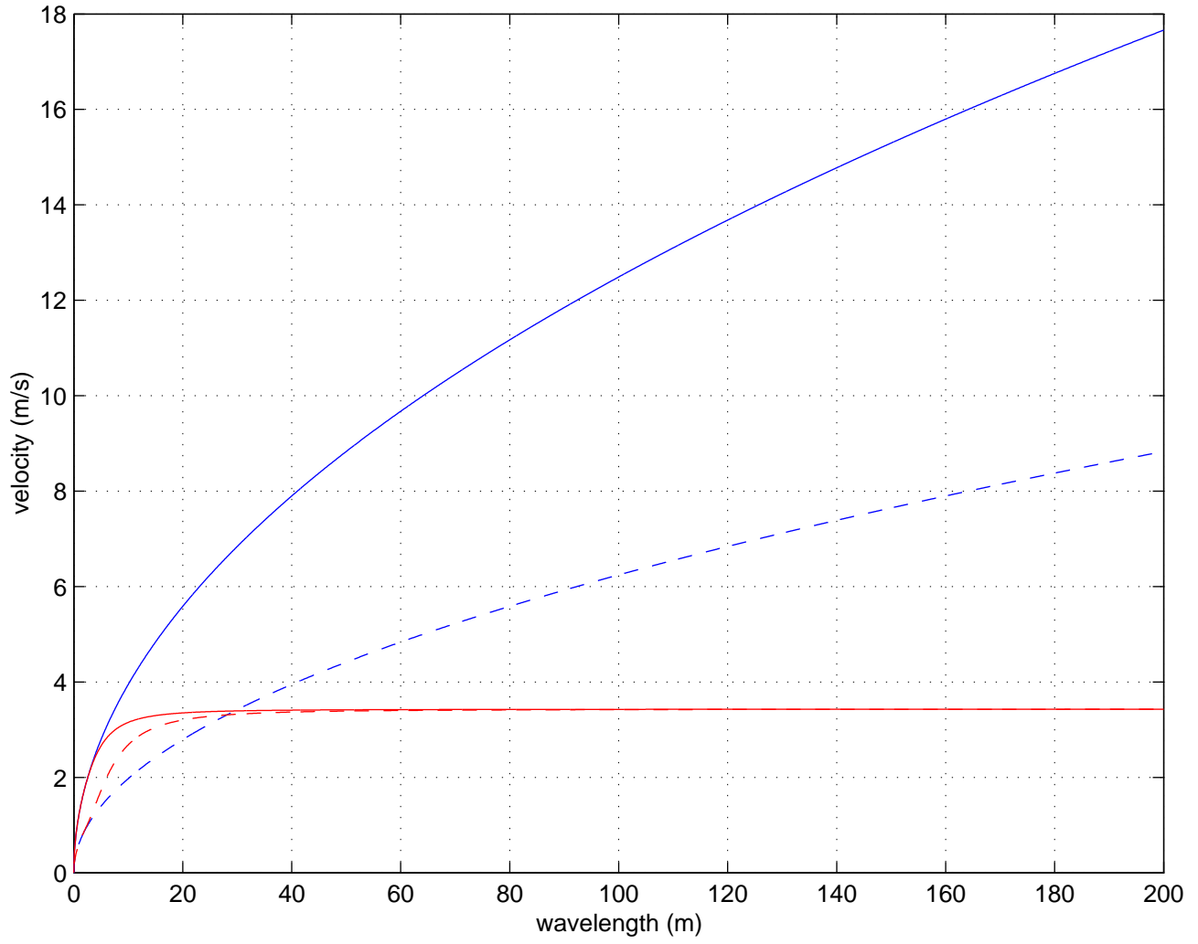
velocity vs. wavelength for inf. water depth and for h=1.2 meters
