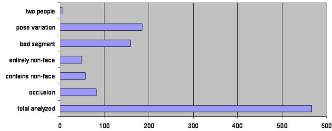
Figure 4-23: Analysis of errors and variations in the face sequence training data that the robot automatically collected during the experiment
