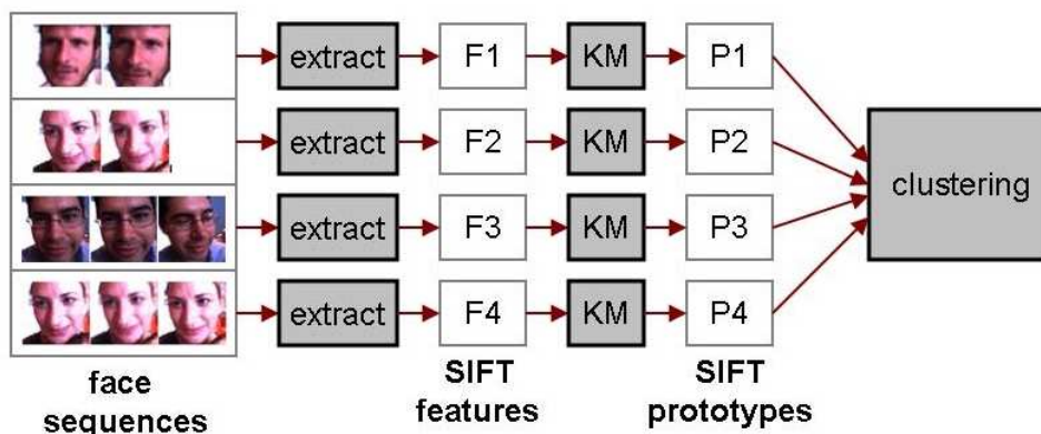
Figure 5-2: The Unsupervised Face Sequence Clustering Procedure. The input is a data set containing an arbitrary number of face sequences. Each face sequence is processed for feature extraction. Extracted features are then passed to the clustering system.
