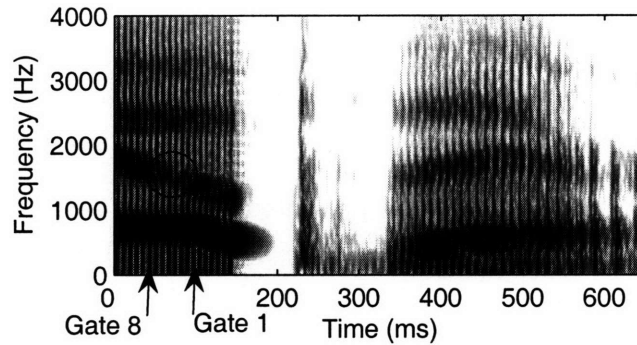
Figure 5-3: The structure of the stimuli (for the non-word ‘ap there’). The initial vowel was synthetic, but the rest of the stimulus was naturally produced speech. The circle indicates the location of the visible effect of the zero on F2. The arrows indicate the locations of the first and eighth gates.
