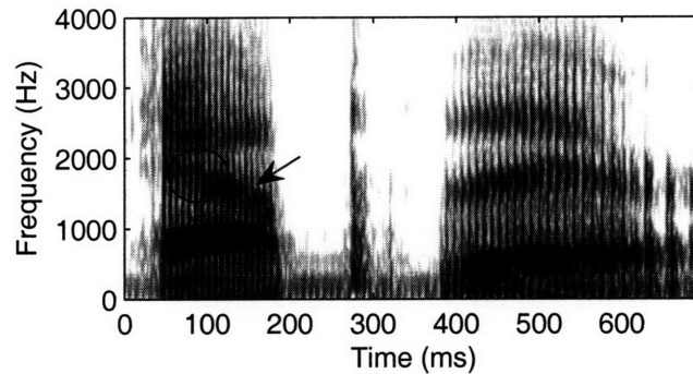
Figure 5-1: Spectrogram of the naturally produced vowel [æ] in the word ‘apter’. The arrow indicates the interaction of the formant with the lower airway zero, and the oval marks the region of interaction between the formant and the lower airway pole.
