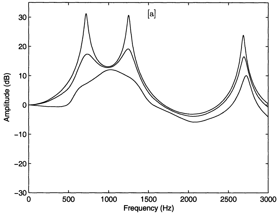
Figure 3-3: Three spectra of [a] as the glottal impedance Z_g decreases. The three Z_g conditions correspond to glottal widths of d = 0.6\text{mm} , 1.2\text{mm} , and 1.8\text{mm} .
