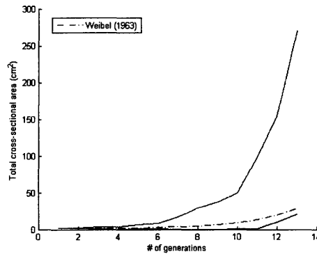
Figure 2-4: Total cross-sectional area of the lower airway as more generations are added.
