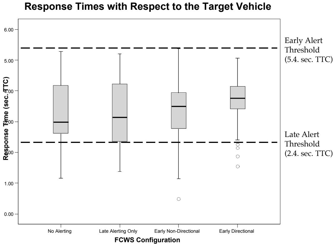
Figure 4-4: Response times with respect to the target vehicle.
