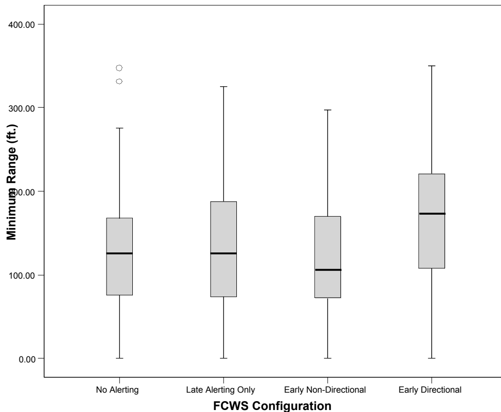
Figure 4-3: Minimum range with respect to the target vehicle.
