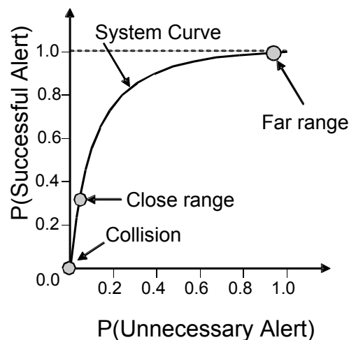
Figure 2-12: An example SOC curve.
