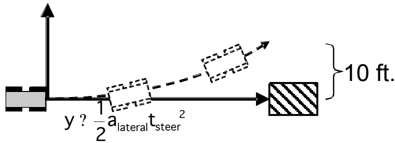
Figure 2-7: A simplified representation of an example steering response.
