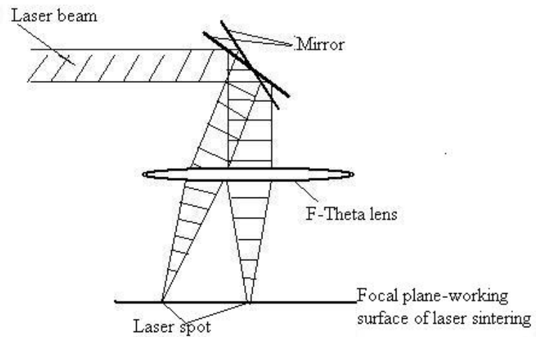
Fig. 2 Focal plane obtained through F-Theta lens
