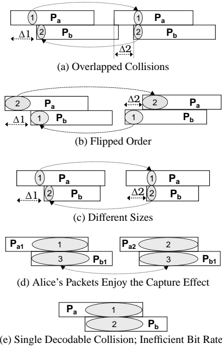
Figure 4—ZigZag applies to various collision patterns. The figure shows a variety of collision patterns that ZigZag resolves. The top three patterns are decoded chunk-by-chunk. The fourth pattern refers to a capture effect which occurs because Alice’s power at the AP is significantly higher than Bob’s. The last pattern occurs when Alice’s power is significantly higher than Bob’s, but Bob’s power is also significantly higher than necessary for his bit rate.
