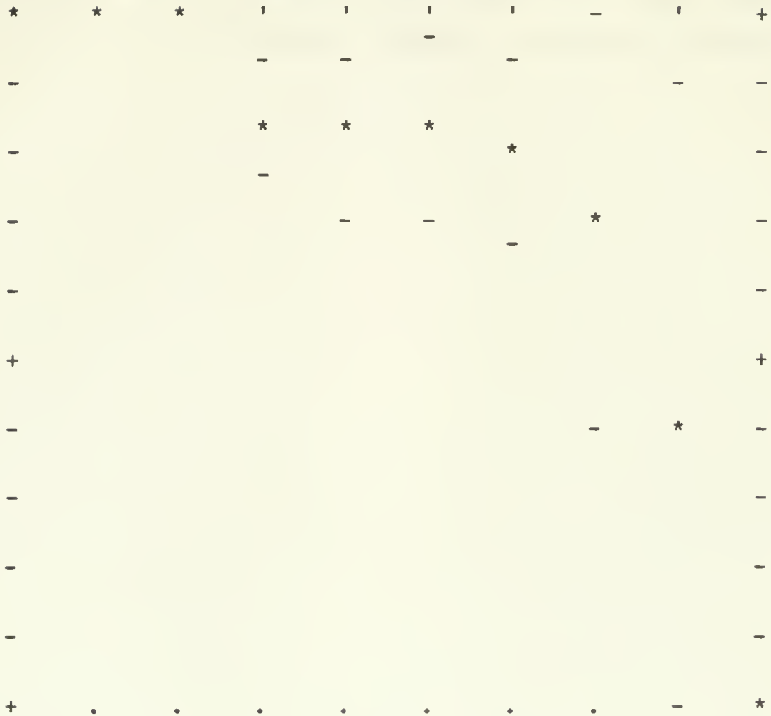
Figure 3.1.1.2: Plot of Bk versus k Set A1, Complete Linkage
