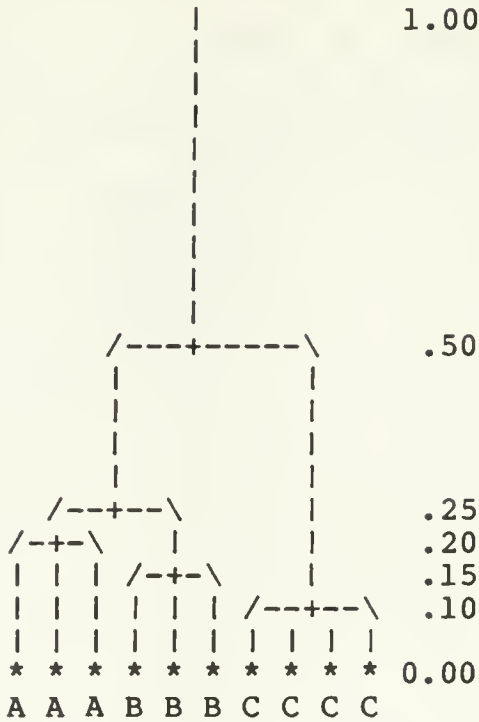
Figure 3.1.5.2: Tree for Data Set A2
