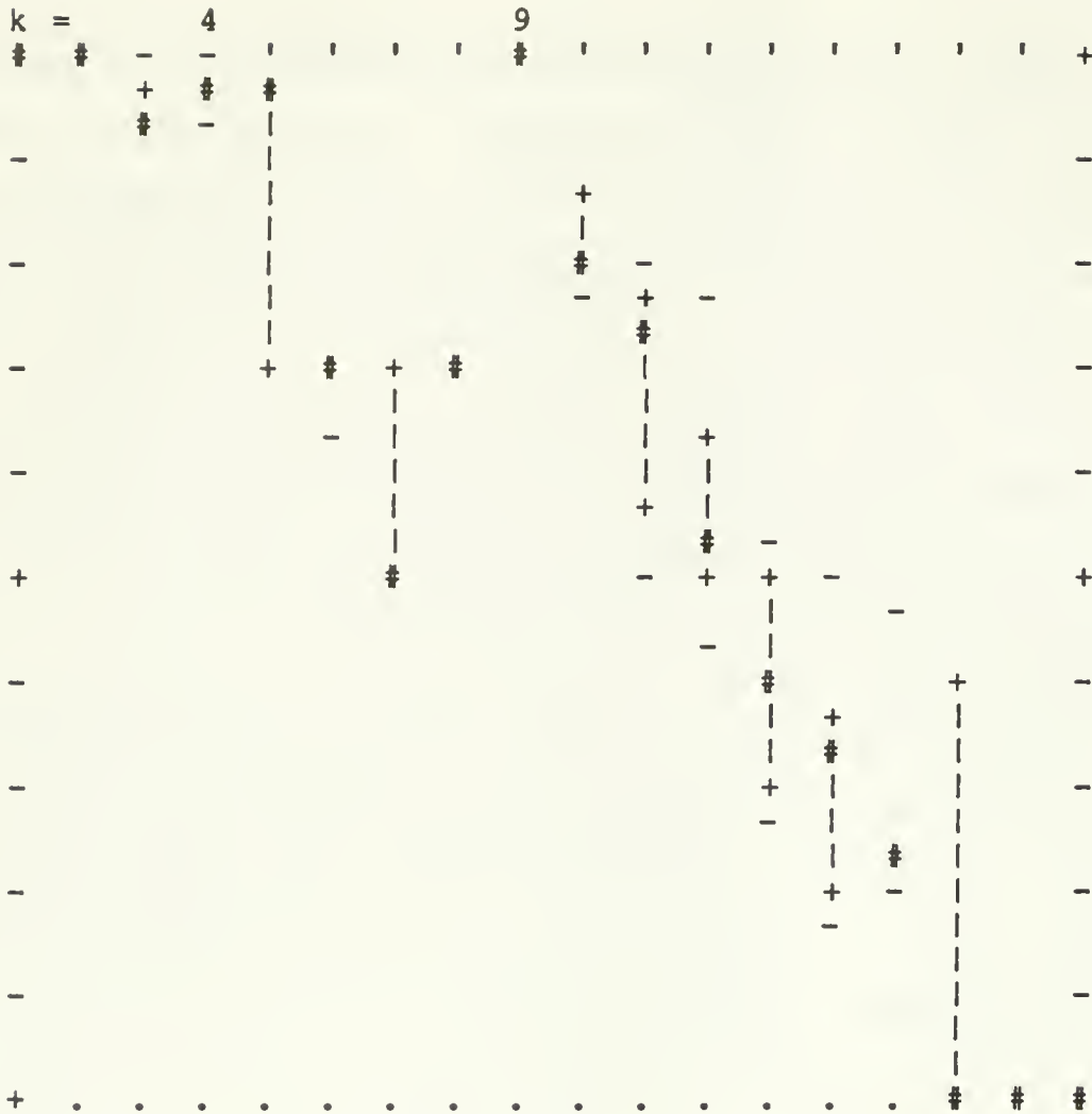
Figure 3.2.2: Plot of B_k versus k Set B1, Average Linkage, 50 Samples
