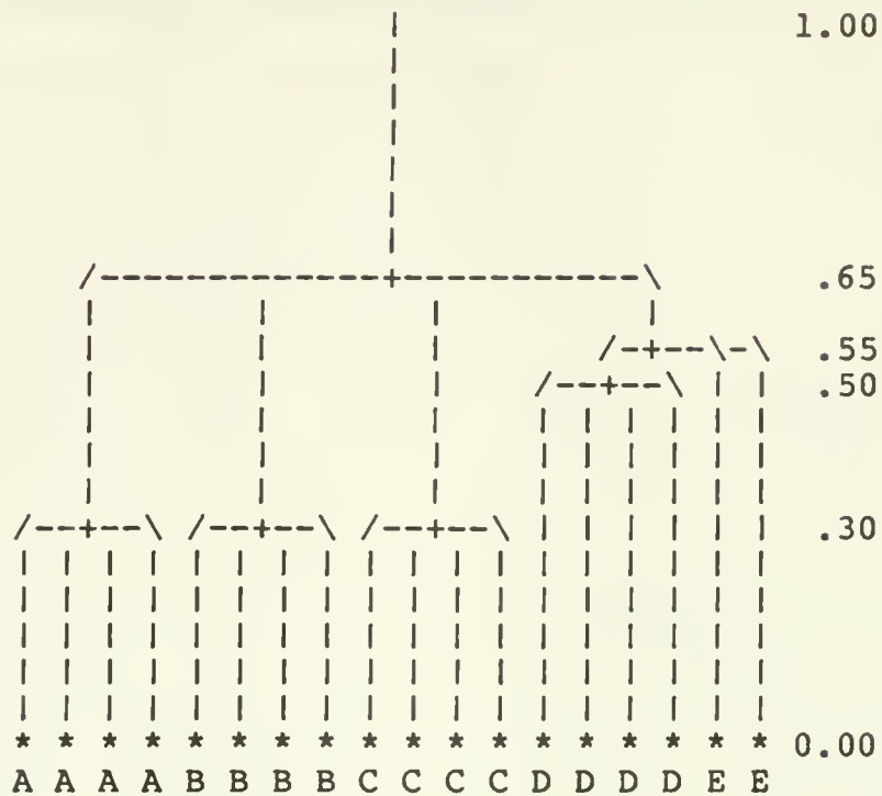
Figure 3.1.2.1: Tree for Data Set B1
