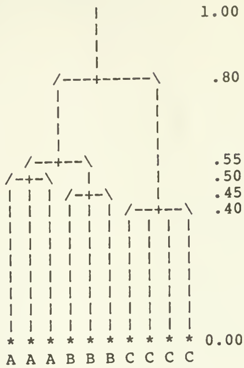
Figure 3.1.5.4: Tree for Data Set A3
