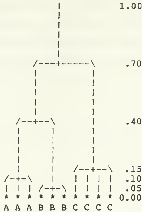
Figure 2.4.2: Tree for Data Set A1
