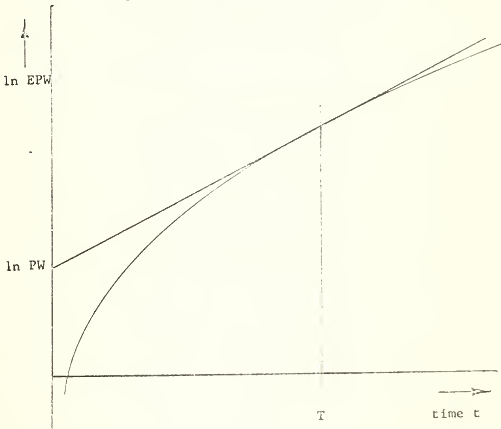
Expected Value and Investor Horizon
