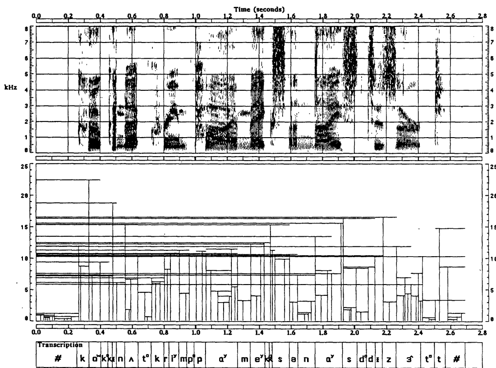
Figure 3.5: A non-monotonically increasing dendrogram.
