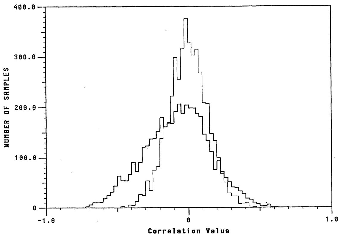
Figure 5.16: Off-diagonal Correlations
