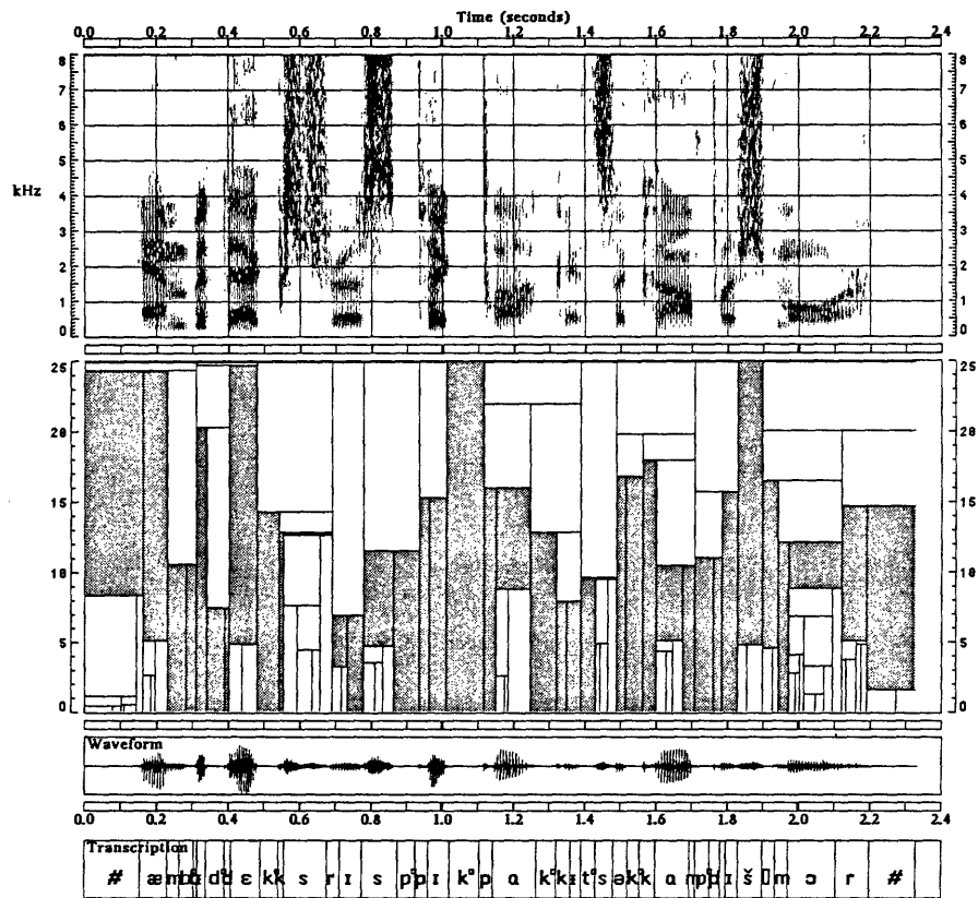
Figure A.7: Dendrogram of 'Ambidextrous pickpockets accomplish more.'
