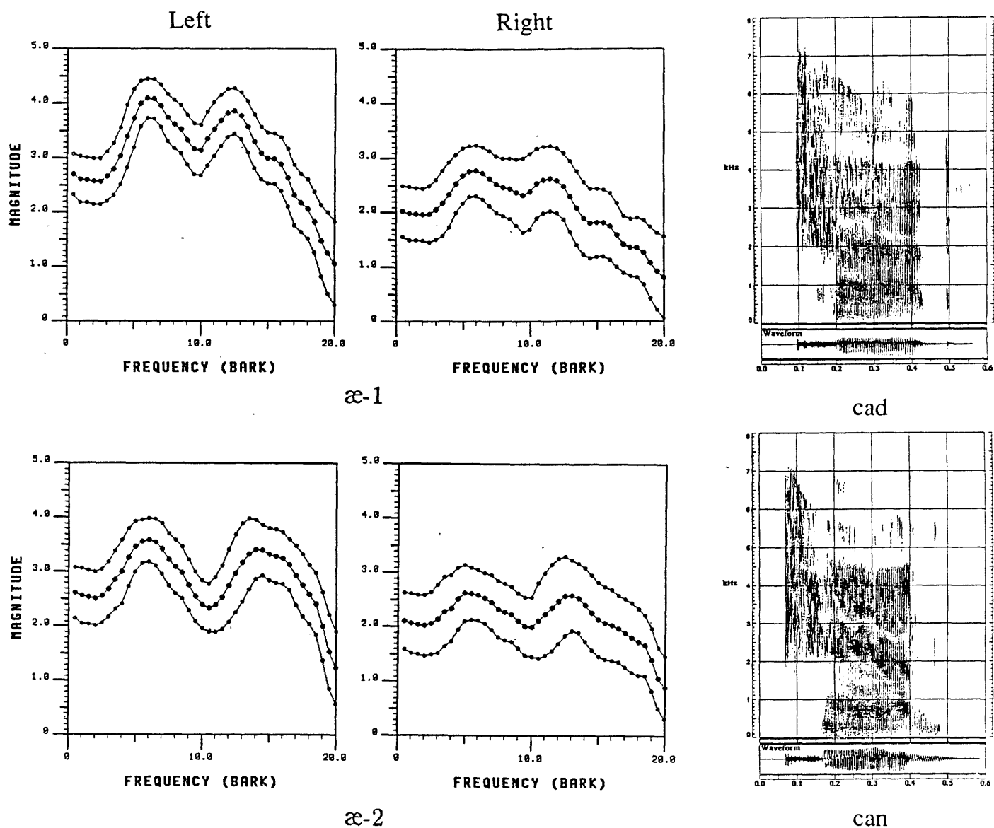
Figure 4.11: Spectra of /æ/ clusters.
