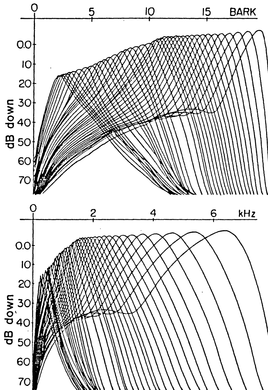
Figure 2.2: Critical-band filter frequency response (after Seneff).
