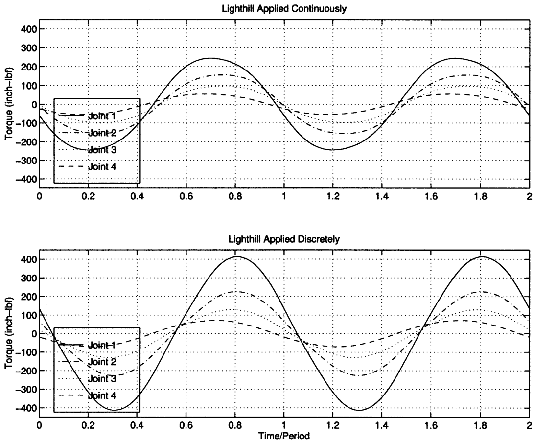
Figure 2-17: Torque Outputs From the Lighthill Continuous EBT Model (“C” in Figure 2-3), Top and From the Lighthill Discrete EBT Model (“D” in Figure 2-3), Bottom
