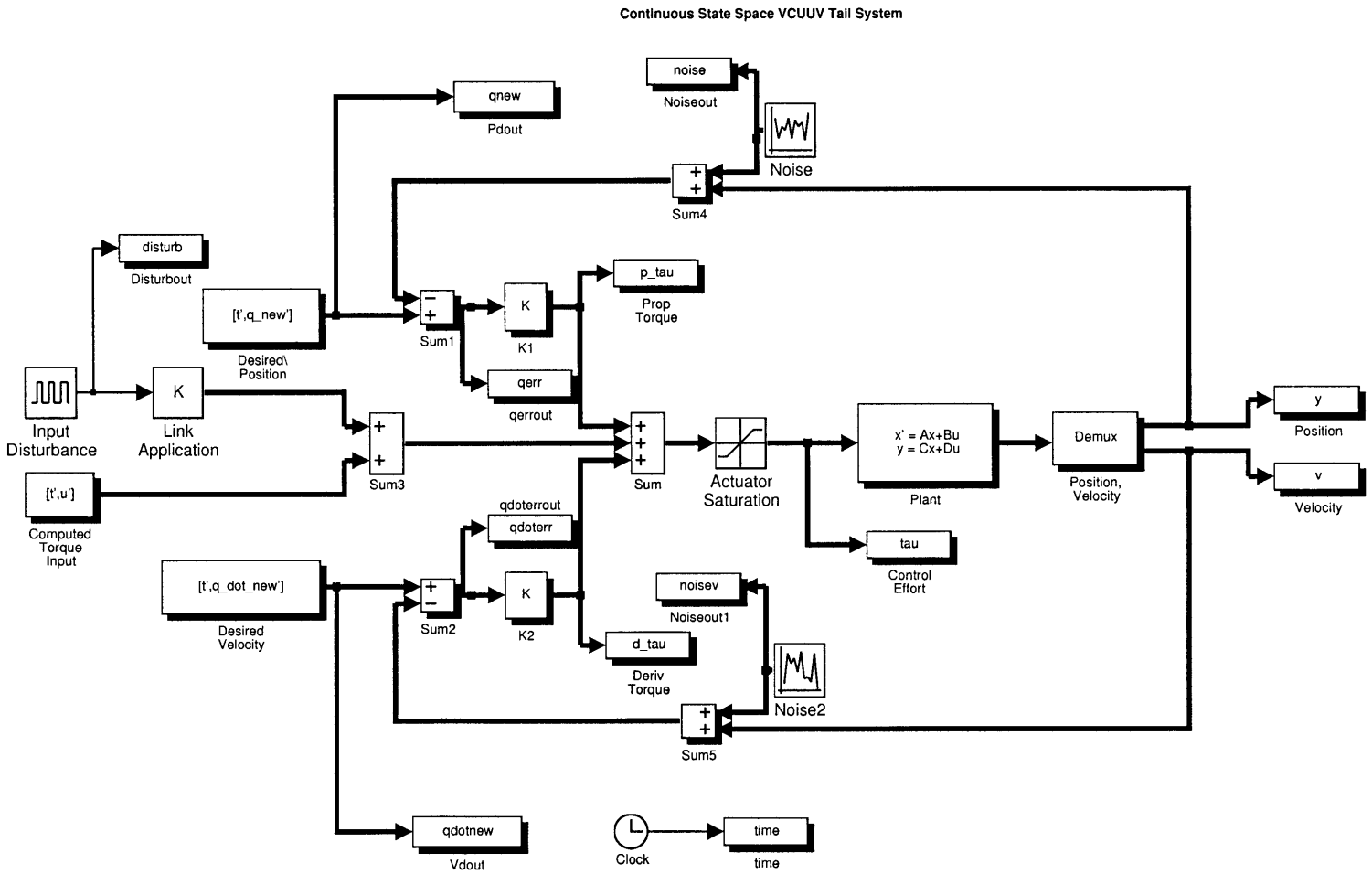
Figure 3-7: Computed Torque Controller Design
