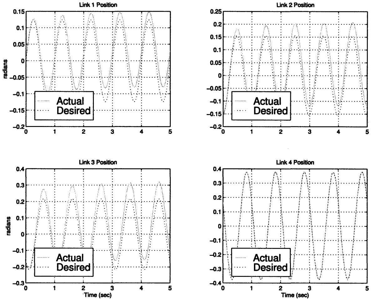
Figure 3-20: Desired and Actual Positions of Links in the Presence of Increased Noise
