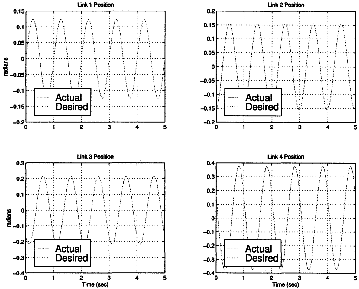
Figure 3-8: Desired and Actual Positions of Links 1-4 for Computed Torque Controller
