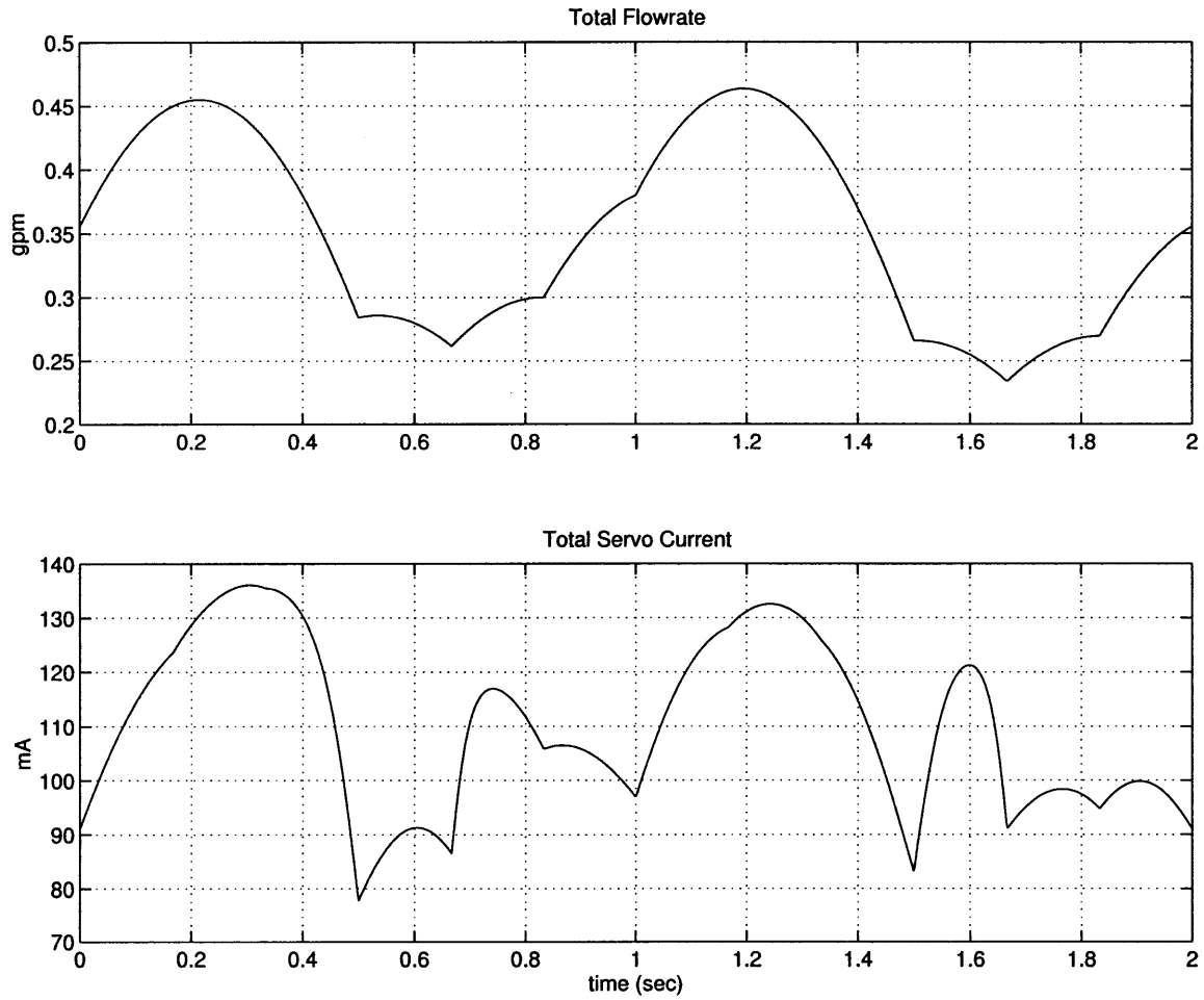
Figure C-6: Total Flowrate and Total Servo Current
