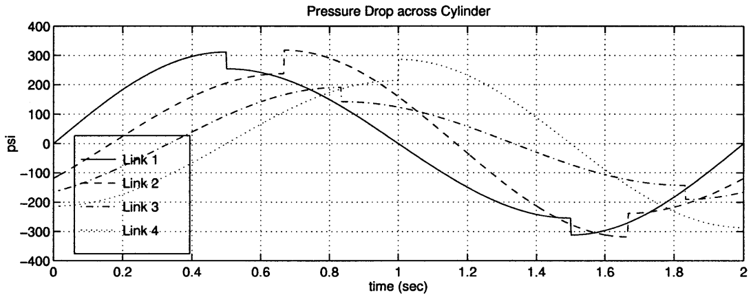
Figure C-2: Pressure Drop Across ServoValve and Piston
