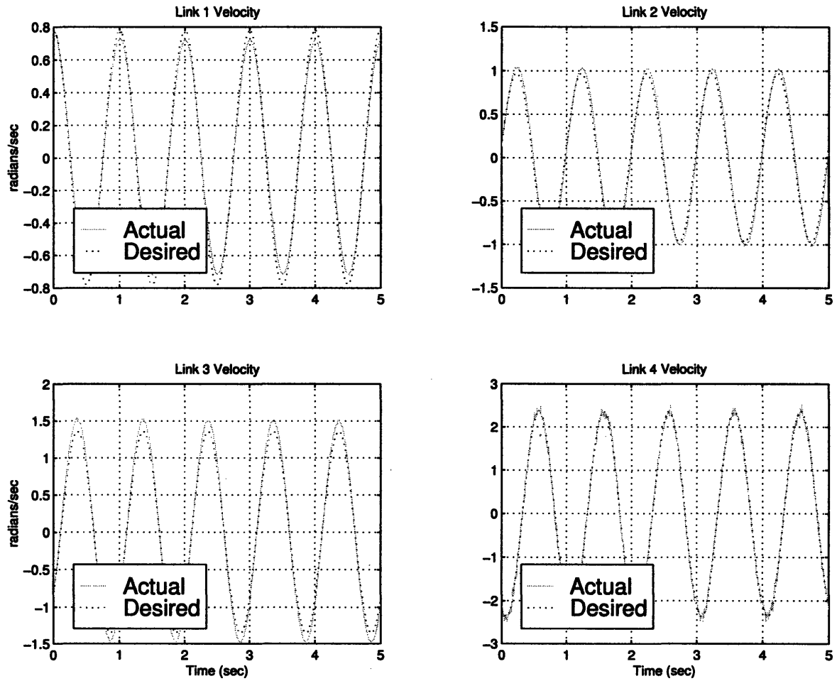
Figure 3-21: Desired and Actual Velocities of Links in the Presence of Increased Noise
