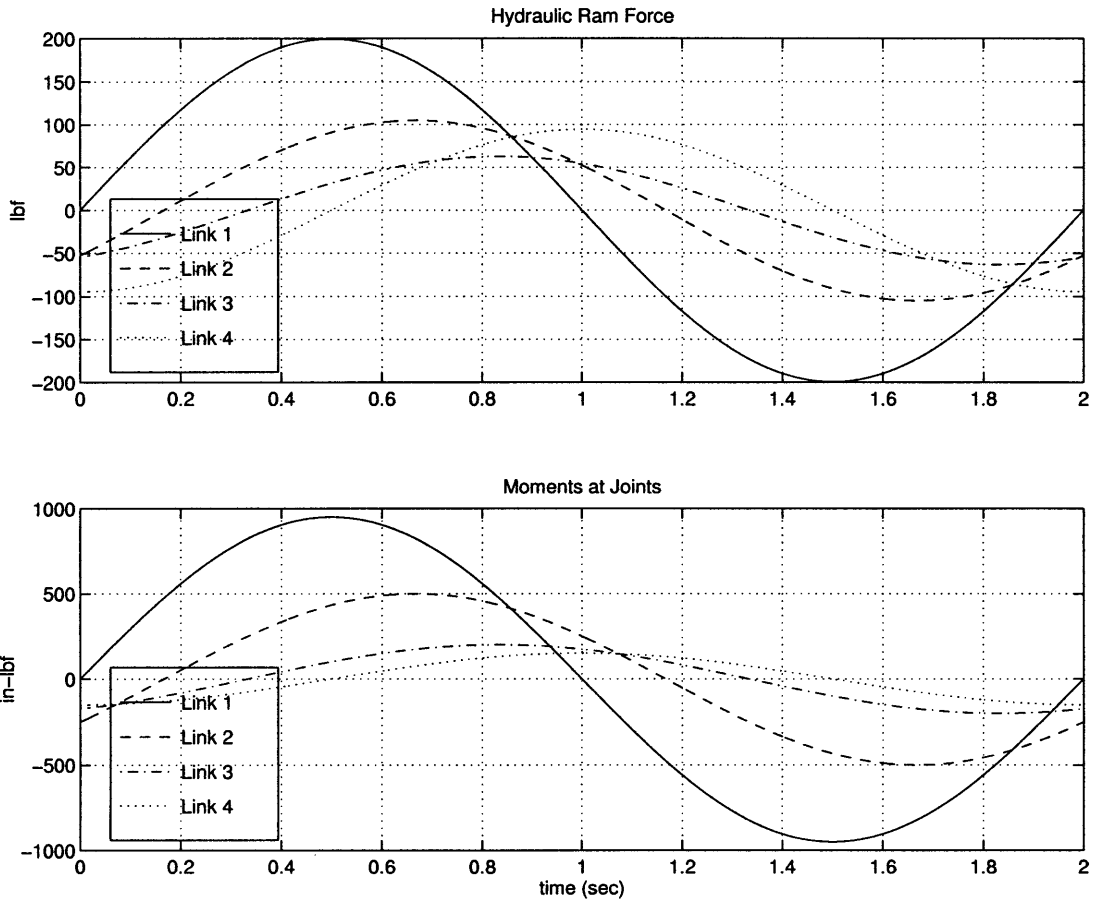
Figure C-4: Piston Force And Joint Moment
