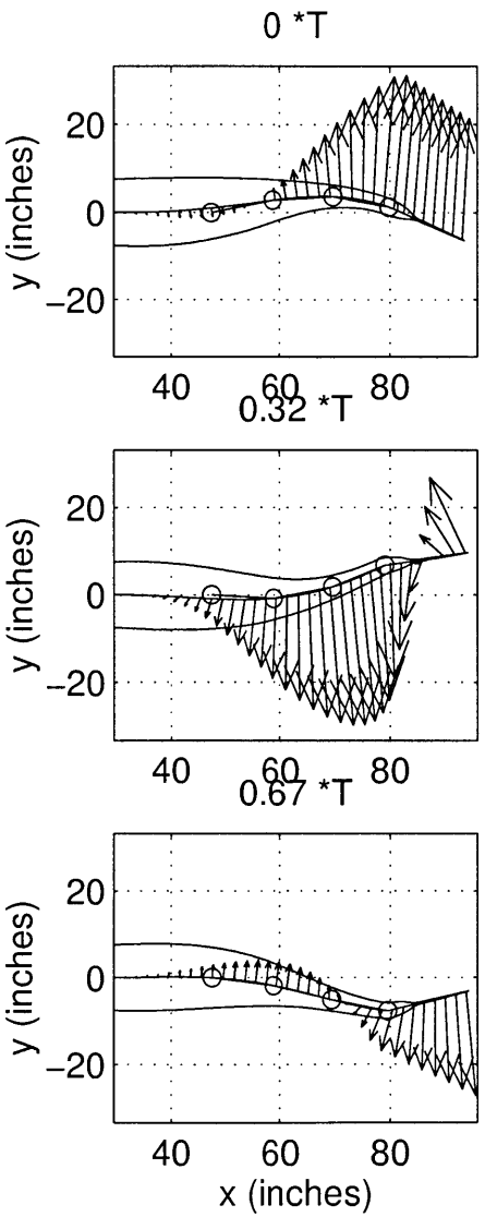
Figure 2-2: Motion of Tail Over One Period, T (Vectors Represent Instantaneous Velocity). Parameters used from Table 2.1
