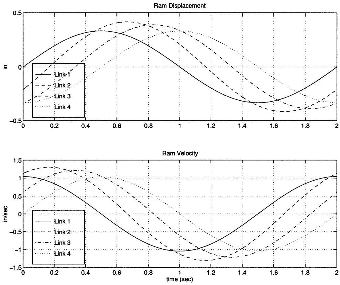
Figure C-1: Piston Displacement And Velocity
