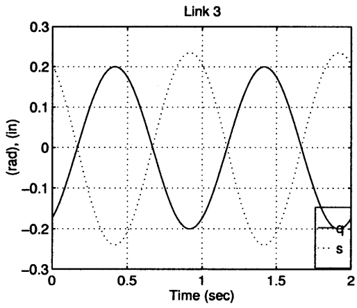
Figure 2-11: Piston Linear, s , and Link Angular, q , Position
