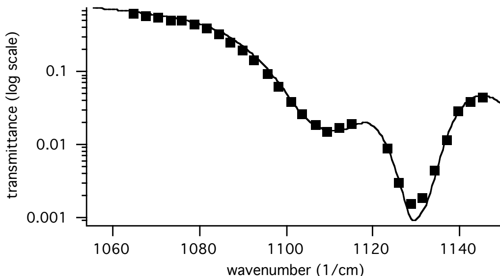
Figure 6. Absorption spectrum of isopropanol measured using the WBC DFB-QCL array at a distance of 6 m (squares). Fourier-transform infrared-spectrometer measurement of the same sample using a Bruker Vertex 80v FTIR instrument (solid line).
