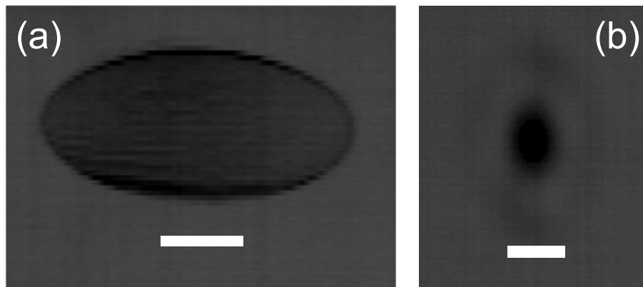
Figure 3. (a) Image of the beam of a representative laser, just after it has been reflected from the grating. The white bar is 1 cm. (b) Image of the far-field spot of a representative laser. The white bar is 1 milliradian.
