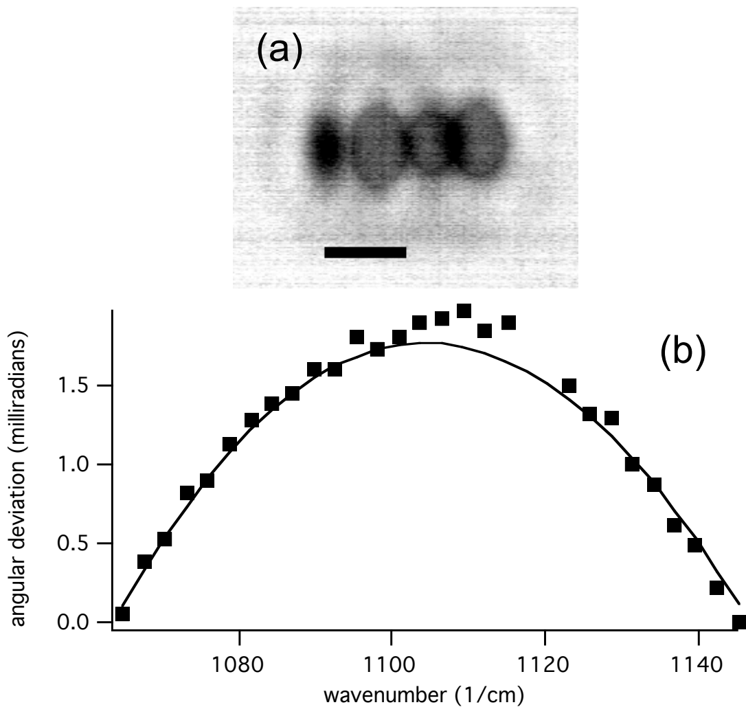
Figure 4. (a) Image of several lasers showing the extent of the residual pointing error of the beams. From the left, we have laser elements #18, 24, 28, and 31 in the array. Lasers 18 and 31 have the largest relative pointing error in the entire array. The bar is 1 milliradian. (b) A plot of the angular deviation of the laser beams, as a function of the laser frequency. Squares represent the pointing of laser beams from the entire array as measured relative to the pointing of laser 31 (rightmost point in the plot). The line is a calculation of the beam pointing using the grating equation (Eq. 1) given the wavelengths of the DFB-QCL array and a grating angle of 54.65 degrees.
