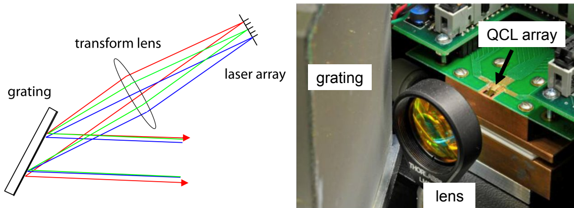
Figure 1. (a) Schematic diagram of wavelength beam combining with an array of distributed-feedback quantum cascade lasers (DFB-QCLs). The emission wavelengths of the lasers are selected by the individual DFBs on each laser ridge in the array. Beam combining is accomplished by a suitably placed grating and transform lens that overlap the beams from each laser in both the near-field and far-field. (b) Photograph of the actual wavelength beam combining setup with the DFB-QCL array.
