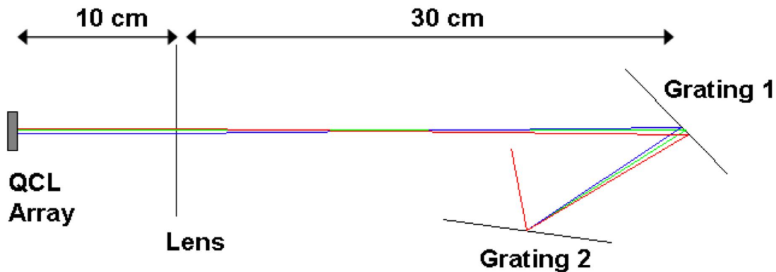
Figure 5. Setup with two gratings to reduce the beam pointing error due to the non-linear grating dispersion. The second grating provides a dispersion of the opposite sign to optimally overlap all the laser beams.
