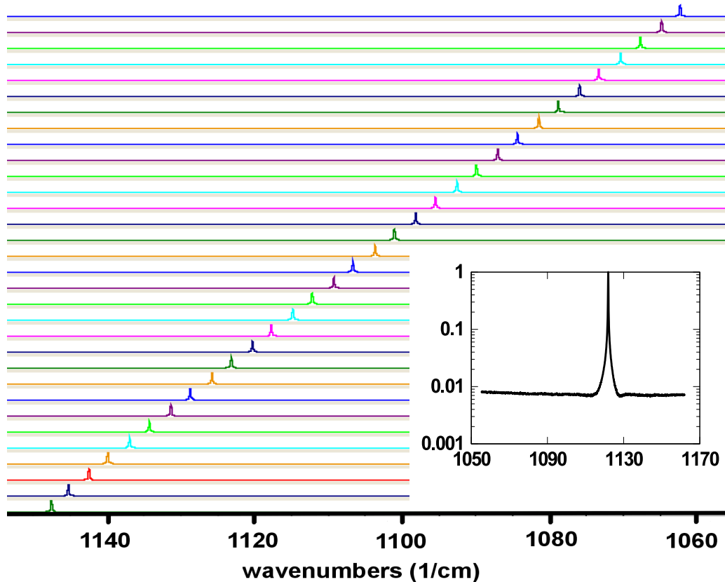
Figure 2. Spectra from the 32 lasers of a DFB-QCL array operating from 1061 to 1148 \text{cm}^{-1} where adjacent lasers have emission frequencies separated by \sim 2.74 \text{ cm}^{-1} . (Inset) Representative spectrum of a single laser, plotted on a log scale to show side-mode suppression of >20 \text{ dB} .
