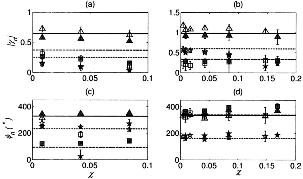
Figure 3-9: Variation of the modal decomposition results with \chi for (a,c) \varepsilon = 0.70 \pm 0.04 and (b,d) \varepsilon = 1.73 \pm 0.05 . Data point markers are as follows: |\gamma_1| , triangles; |\gamma_2| , squares; and |\gamma_3| , stars. Open and closed data points show experimental and numerical results, respectively. Horizontal lines show linear theoretical estimates for modes 1 (solid), 2 (dashed) and 3 (dotted).
