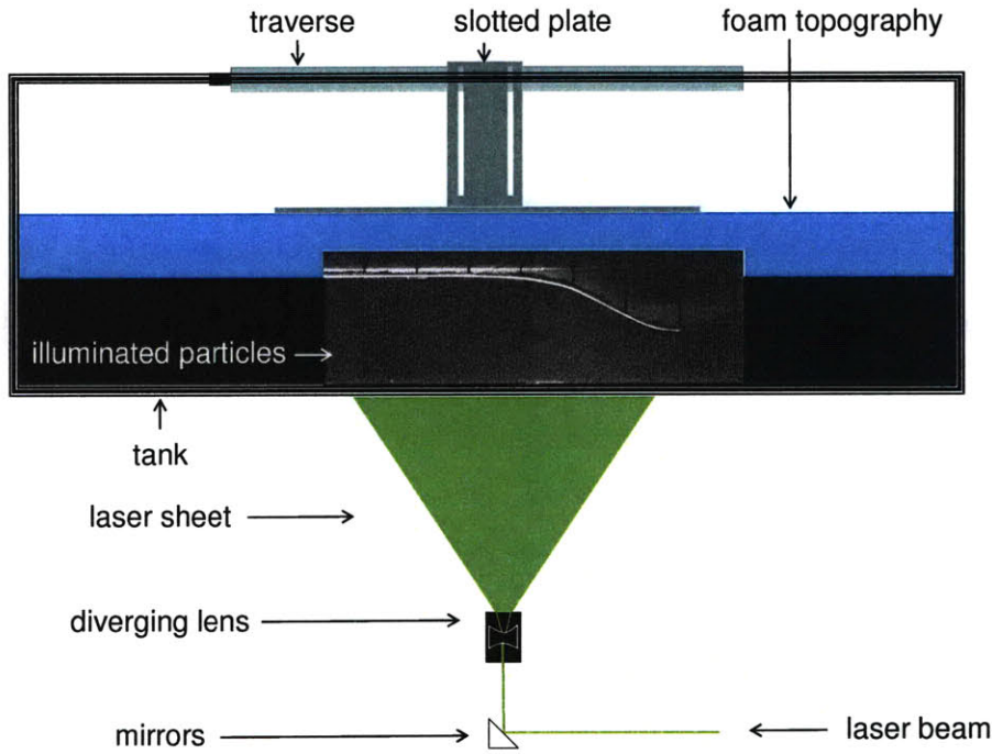
Figure 2-6: Schematic of the PIV set-up showing the laser beam passing through a cylindrical lens to form a laser sheet. A PIV image of the illuminated particles where the surface of the topography is visible is super-imposed. The foam block is on an adjustable mount that connects to the traverse, which is attached to the top of the tank.
