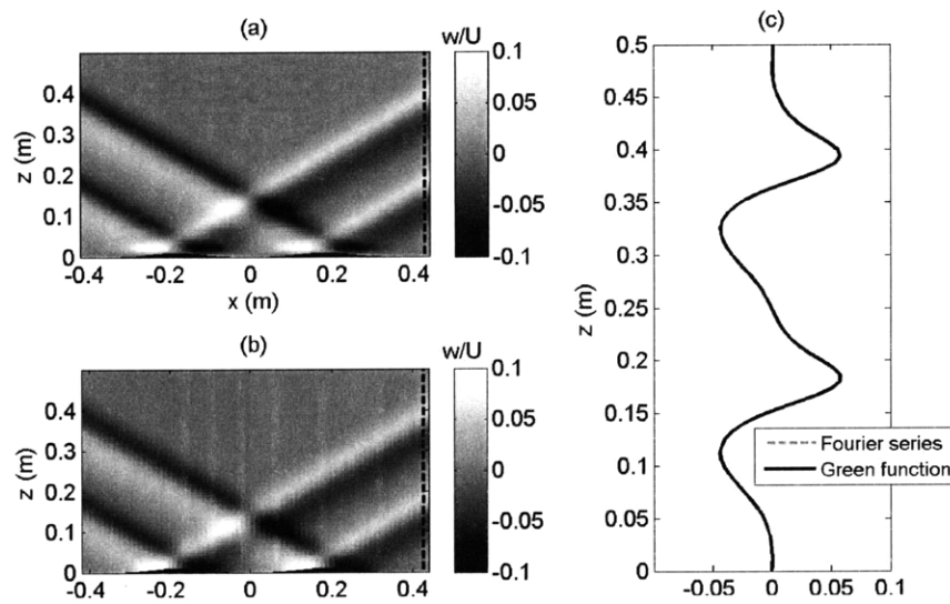
Figure 4-2: Comparisons of w/U for internal tides generated by two identical subcritical double Gaussian ridges using the internal tide solution presented in section 4.1 (using a Green function) and the solution of Balmforth et al. [6] (using a Fourier series). The ridges are L = 6\sigma apart and have criticalities \varepsilon = 0.17 . Snapshots at \Phi = 0 using (a) the Green function solution and (b) a Fourier series solution, and (c) comparison of the respective vertical profiles at x = 7\sigma .
