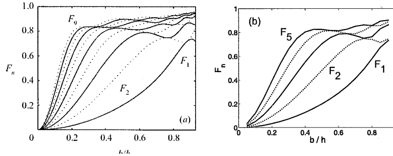
Figure 4-3: Comparisons of F_p for a knife-edge topography in an exponential stratification fit to WOD data obtained using (a) the solution of [55] (panel (a) is reproduced from figure 7 in the cited paper) and (b) the internal tide solution presented in section 4.1. The nomenclature is from [55]: b/h is the depth ratio. The lines represent increasing values of p .
