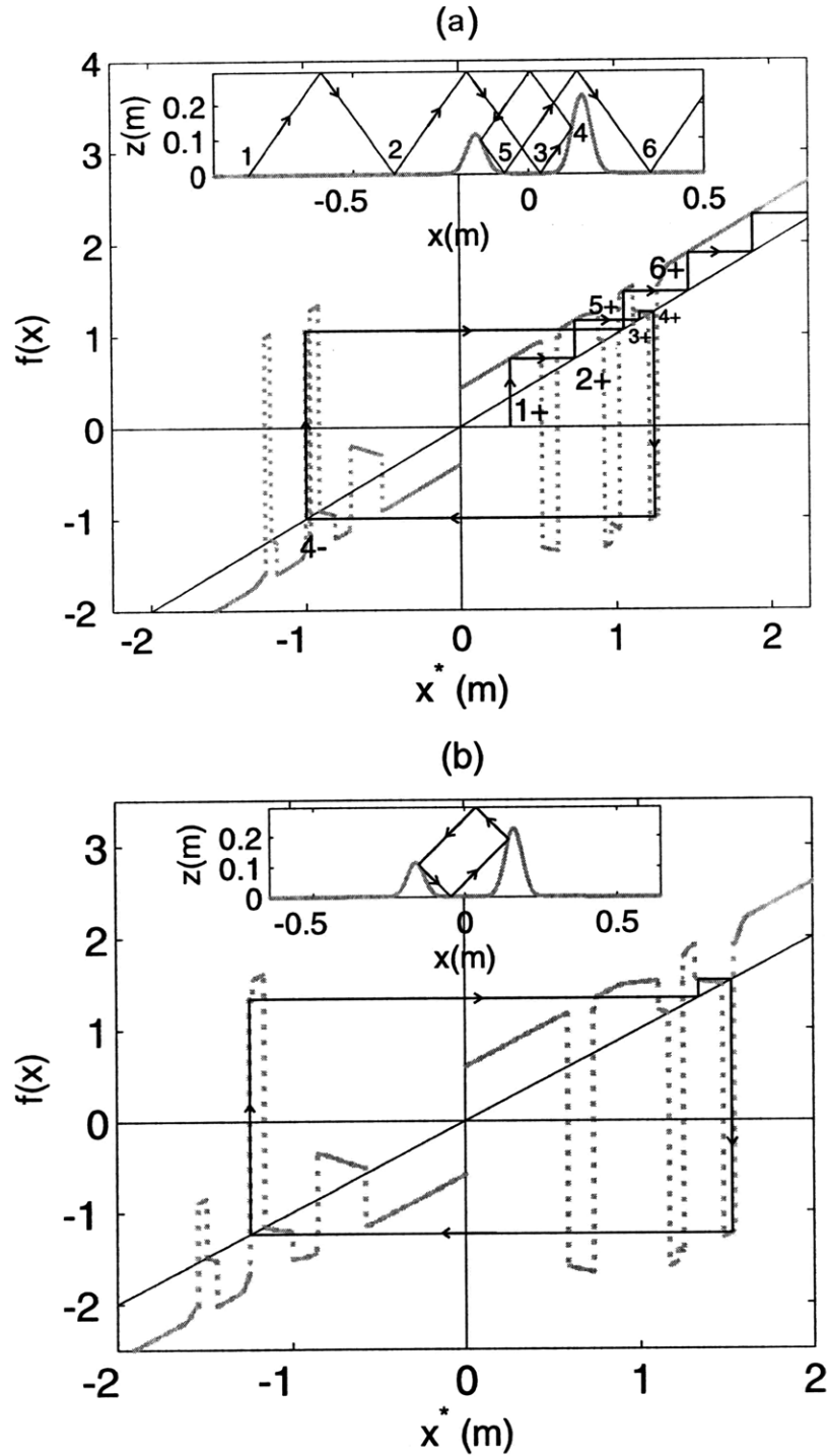
Figure 5-2: A 1-D map of upward reflections of internal wave rays from a double Gaussian ridge. An example ray path is indicated by the solid black line in each 1-D map and, within the inset, the ray path in the physical (x, z) -plane is presented. The coordinate x^* = x \pm l . (a) Configuration with \theta = 54.9^\circ in which internal wave rays escape, with l = 1.12 m. Upward reflections on the topography occur at the points labeled 1 through 6. (b) Configuration with \theta = 47.1^\circ in which an internal wave attractor exists, with l = 1.30 m.
