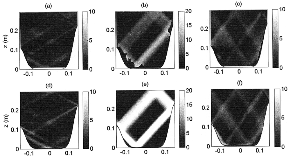
Figure 5-7: Experimental and theoretical snapshots of the velocity magnitude between the ridges. (a)-(c) present experimental results for \theta = 29.4^\circ, 47.1^\circ, 54.9^\circ respectively, and (d)-(f) are the corresponding viscous theoretical results.
