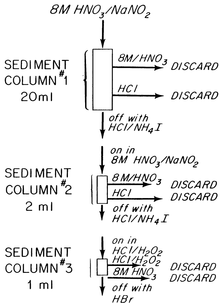
Fig. 3.2a: Summary of the ion exchange procedures for sediment samples.
