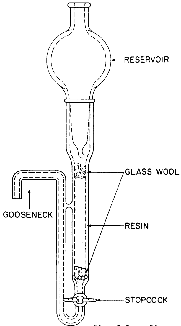
Fig. 3.1a: "Goose neck" ion exchange column.
