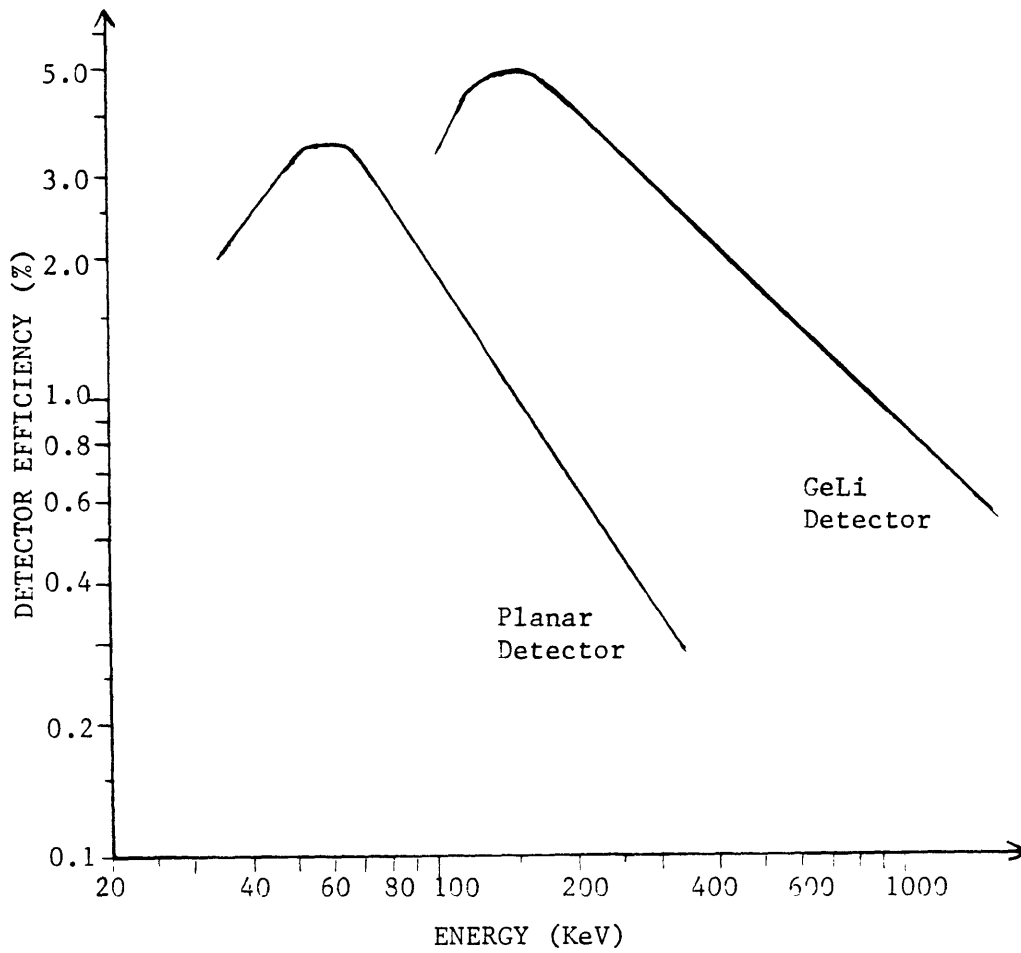
Fig. 2.1: Efficiency vs. Energy plot for a 50gm standard sediment sample in a 4oz. counting jar. -note log-log scale
