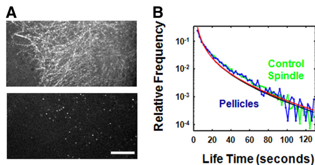
Figure 6. (A) Microtubules growing off of pellicles in X. laevis egg extracts. (A, top) Heavy labeling with Alexa-488 tubulin allows all microtubules to be visualized, but individual filaments cannot be resolved. (A, bottom) The same region as in A with single molecule level Alexa-647 tubulin. Bar, 10 \mu\text{m} . (B) Distributions of tubulin lifetimes from pellicles (pellicles, blue) and unperturbed spindles (control spindles, green) are very similar. Best fits to Equation 1 are displayed for pellicles (red, \tau = 71 \pm 9 s) and spindles (black, \tau = 64 \pm 6 s).
