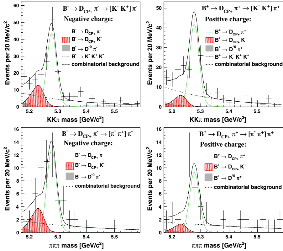
FIG. 3 (color online). Invariant mass distributions of B^- \rightarrow D_{CP^+} \pi^- candidates for each reconstructed decay mode. The pion mass is assigned to the prompt track from the B decay. A requirement on the PID variable was applied to suppress the D\pi component and favor the DK component. The projections of the likelihood fit for each mode are overlaid. The p value for agreement of data with the fit is 0.95
