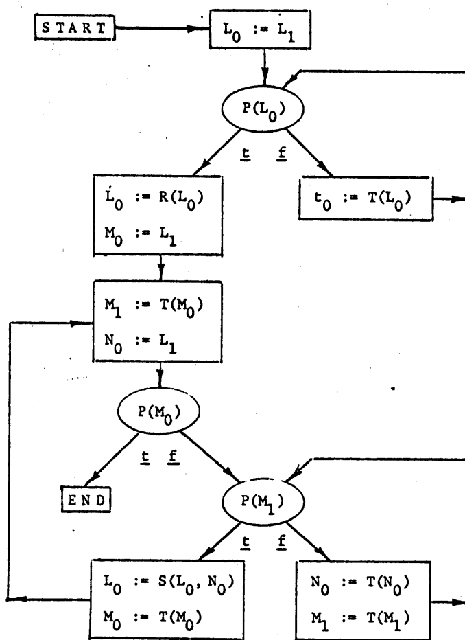
Fig. 3. Program schema equivalent to a linear schema.
