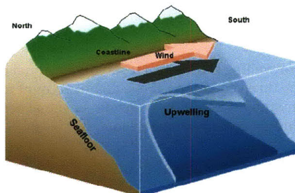
Figure 2-1: Schematic of Coastal Upwelling. ( http://www.greenseaupwelling.com/_images/upwellPic.png )
