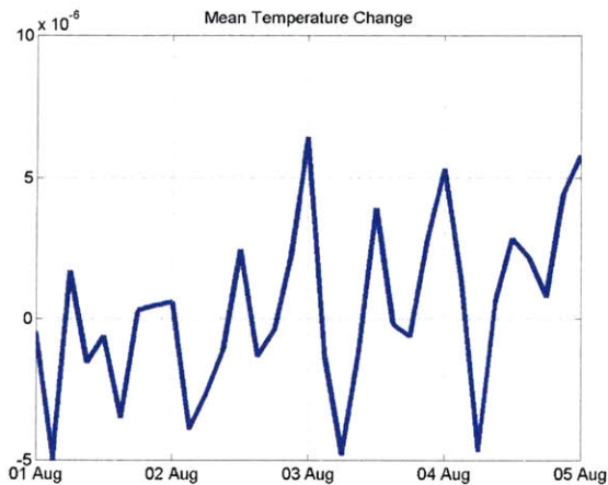
Figure 4-16: Volume-averaged time rate of change of temperature (K /s) for Run 2.
