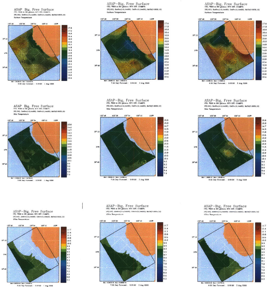
Figure 3-1: Temperature at 0, 30, and 150 meters deep on August 1 00Z, August 3 00Z, and August 5 00Z, 2006 for a baseline MSEAS primitive-equations simulation.
