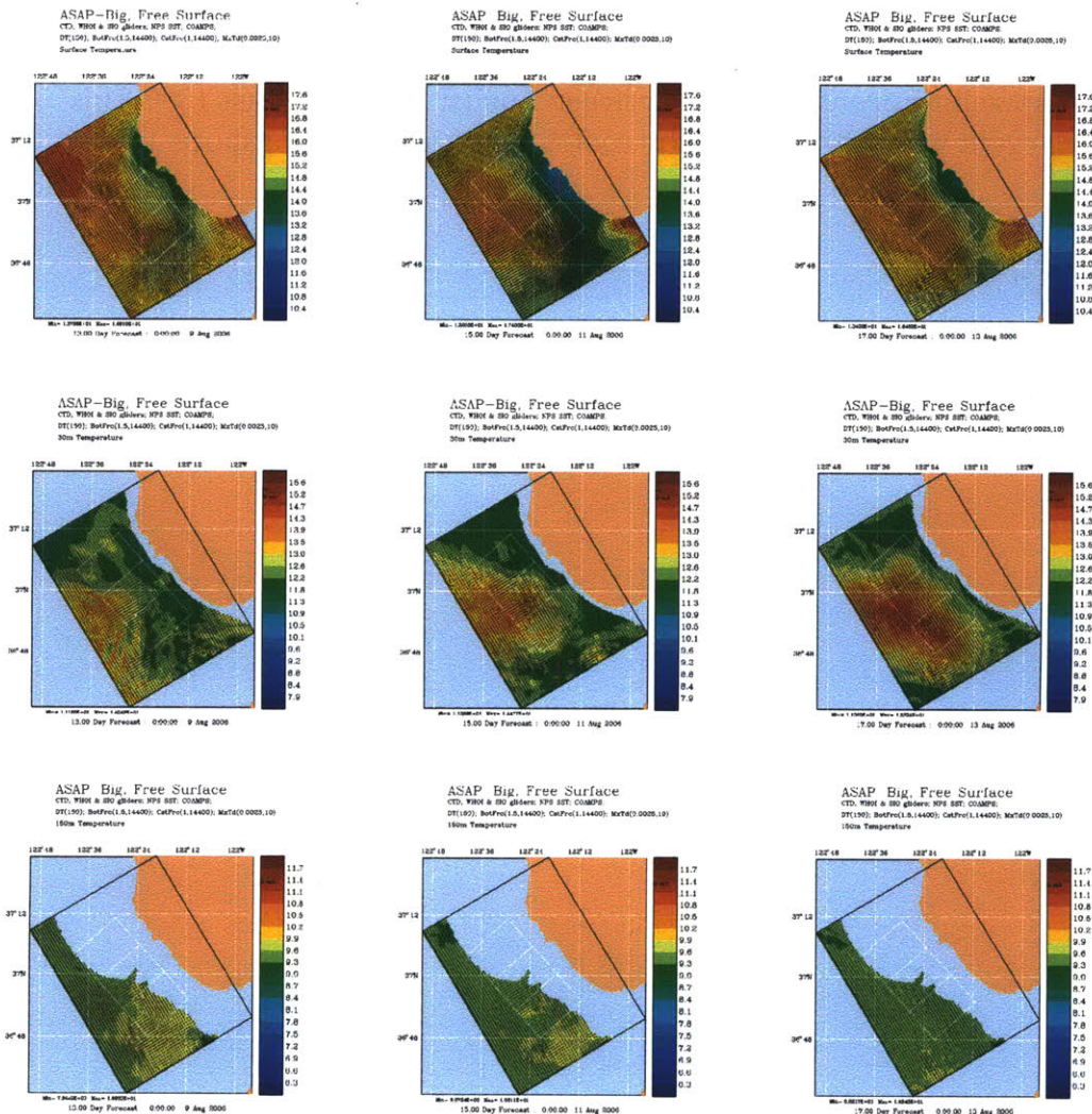
Figure 3-6: Temperature at 0, 30, and 150 meters deep on August 9, August 11, and August 13, 2006 for a baseline MSEAS primitive-equation simulation.
