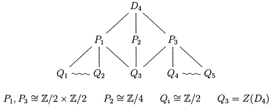
Figure 2-1: Subgroup-conjugacy lattice of D_4
