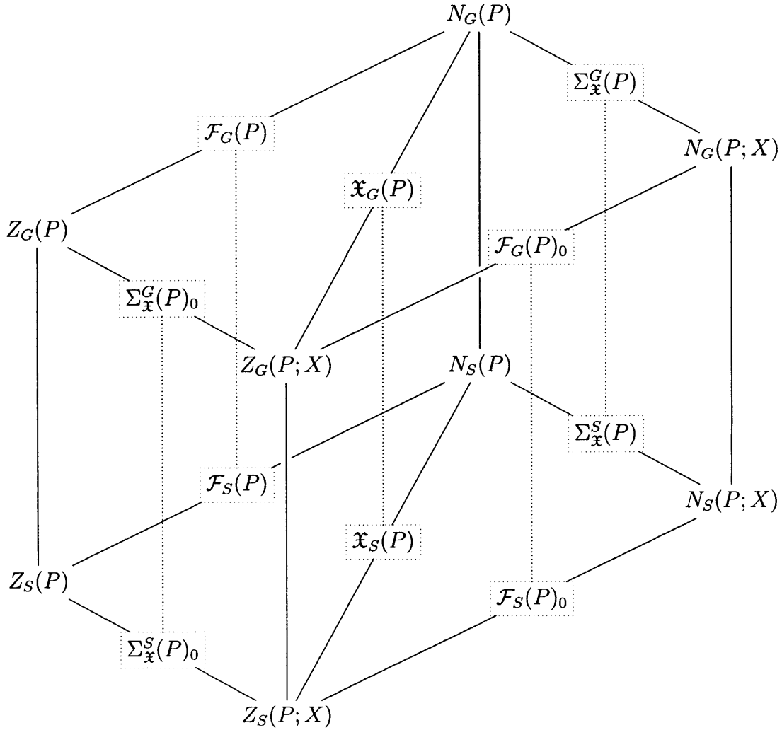
Figure 4-2: Comparing S -automizers to G -automizers
