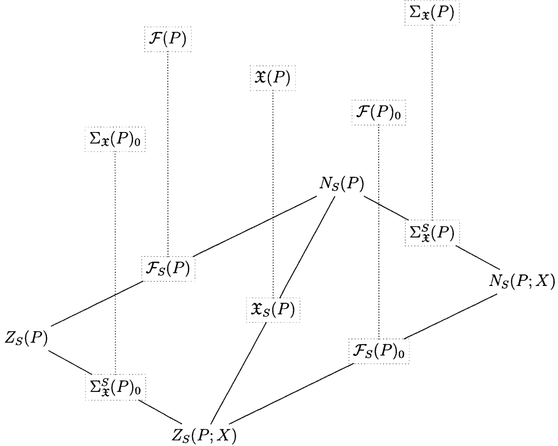
Figure 4-3: Comparing S -automorphisms to \mathfrak{X} -automorphisms
