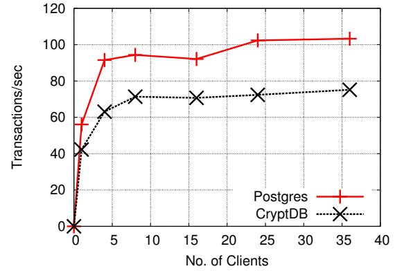
Figure 6: Throughput of TPC-C transactions as a function of the number of concurrent clients.
