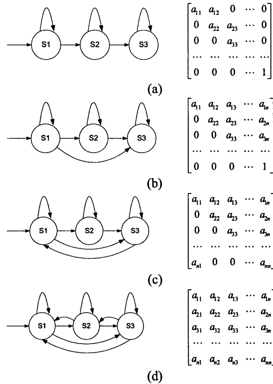
Figure 3-2: HMMs used in the experiment (a) A strict left-right model, each state can transfer to itself and the next one state. (b) A left-right model, each state can transfer to itself and any state to the right of it. (c) A variation of the left-right model, additional to (b), the last state can transfer to the first state. (d) A fully connected model.
