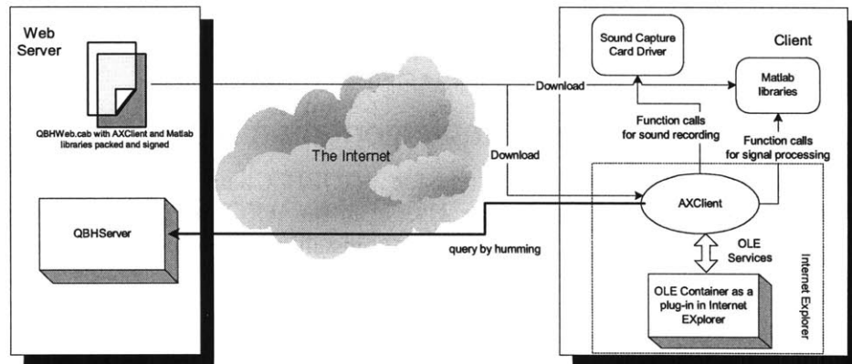
Figure 6-6: Structure of QBH AXClient.
