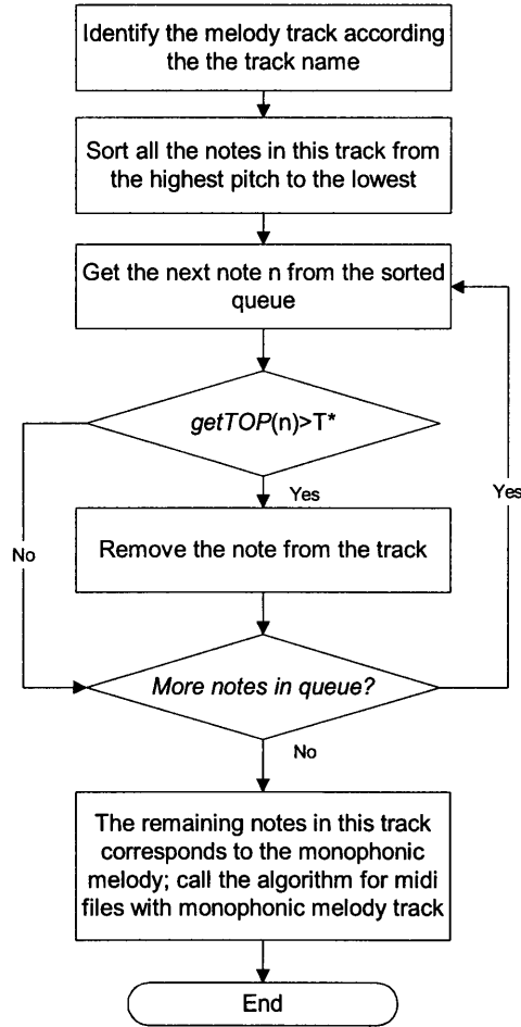
Figure 5-11: The revised skyline algorithm for extracting melody from MIDI files with polyphonic melody track.
