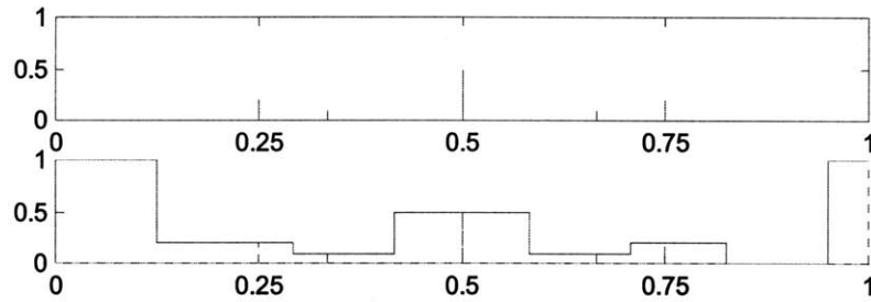
Figure 5-22: Onset likelihoods within one beat. Above: L_d(t) Below: L_c(t)
