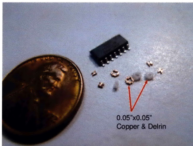
Figure 4.2c 50 mil conductor and insulator parts
