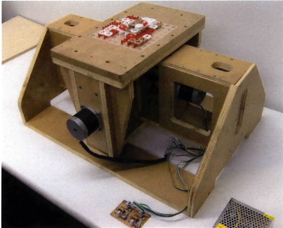
Figure 5.1b Bench-level prototype of a 2axis machine bed
