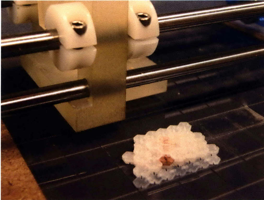
Figure 5.2h assembler head prototype and assembly of plastic and copper parts
