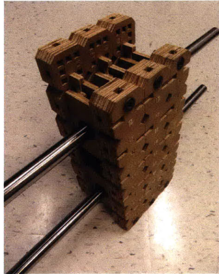
Figure 6b bench-level prototype of a press fit assembly with linear bearings and shafts this is a prototype for a linear machine component
