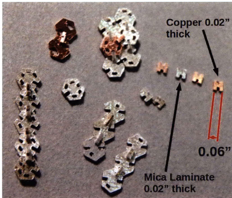
Figure 4.2f Mica laminate and copper parts machined on a CNC mill with 1/64" carbide endmill
