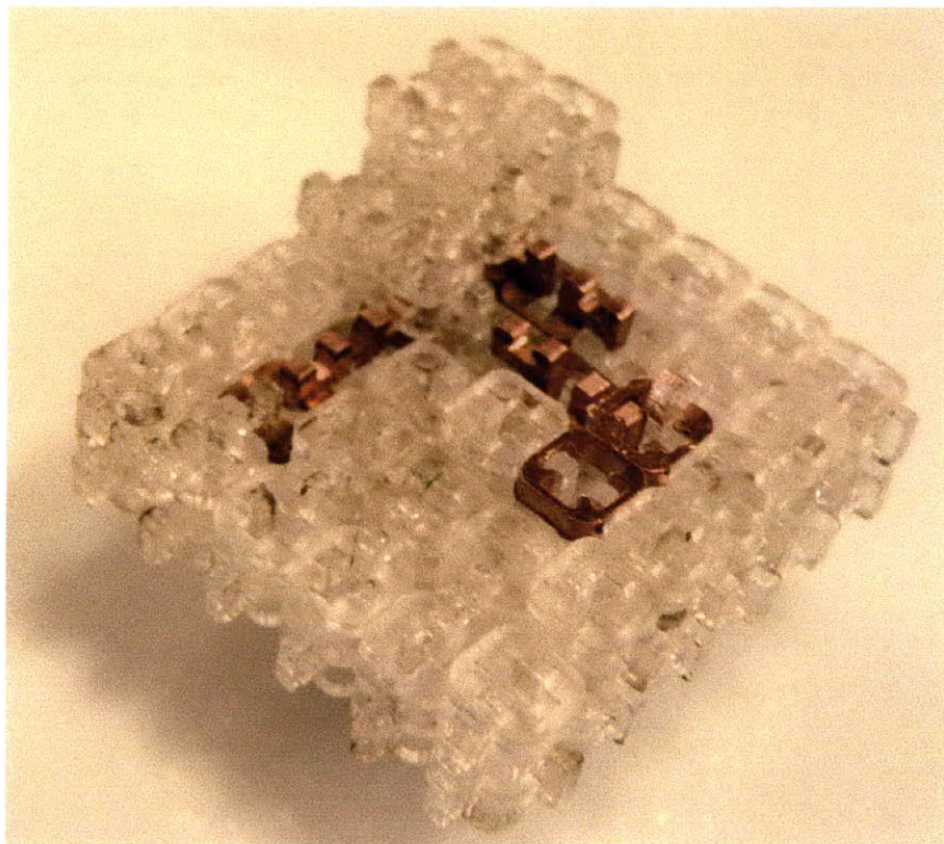
Figure 4.5c Digital assembly of acrylic and copper parts
