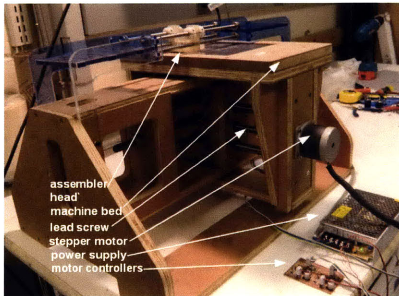
Figure 5.2d bench-level prototype of CNC machine bed and hand actuated assembler head
