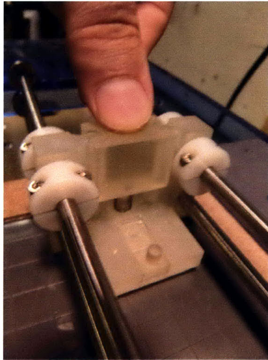
Figure 5.2f part pushing mechanism being actuated by hand
