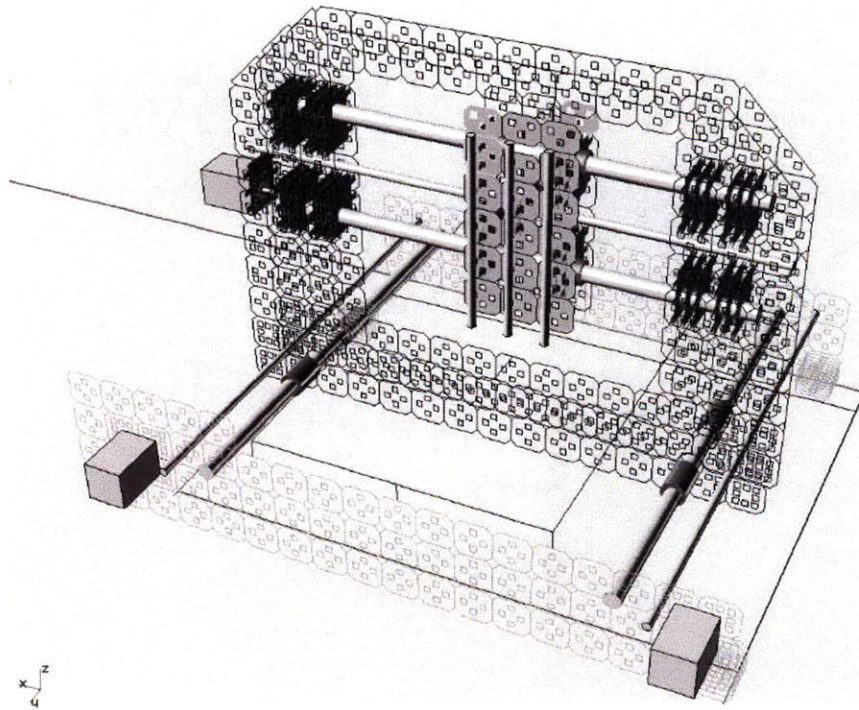
Figure 6a Schematic diagram of 3Axis CNC machine made of press-fit parts
