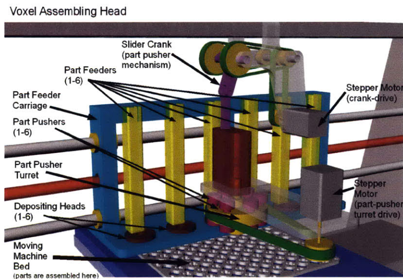
Figure 5.2c detail of print head concept, showing multiple part feeders, tool changing turret, and part pushing mechanisms
