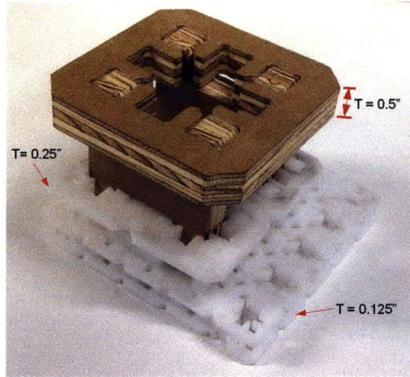
Figure 4.3a self-similar parts constructed and assembled showing hierarchy
