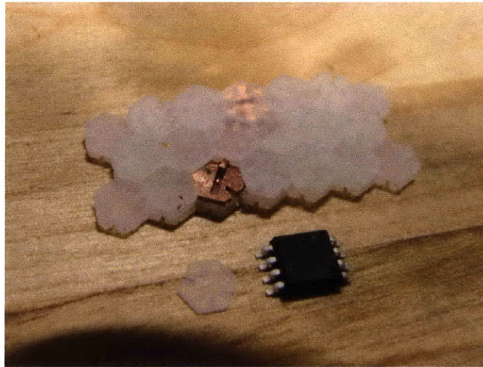
Figure 4.5h Press fit assembly of ABS plastic and copper parts
