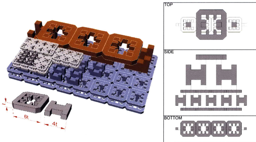
Figure 4.3b Diagram of hierarchical parts showing scalability and vertical interconnect between self-similar parts
