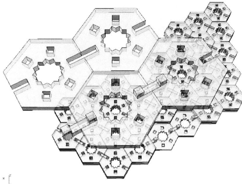
Figure 4.3d 3D model of hierarchical hexagonal press-fit structure
