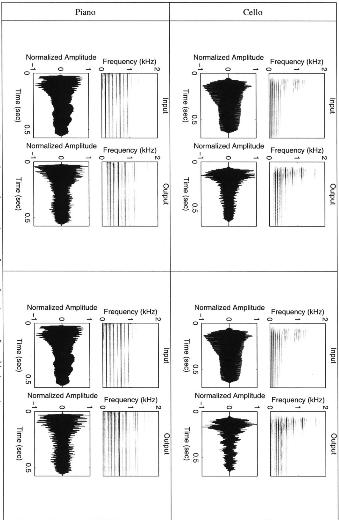
Figure 8: Input and output time waveforms and spectrograms for real instruments
