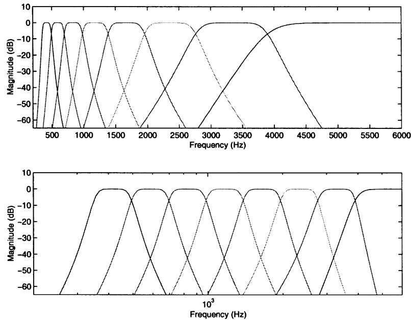
Figure 6: Frequency response of bandpass filters, shown on linear (top) and logarithmic (bottom) frequency scales
