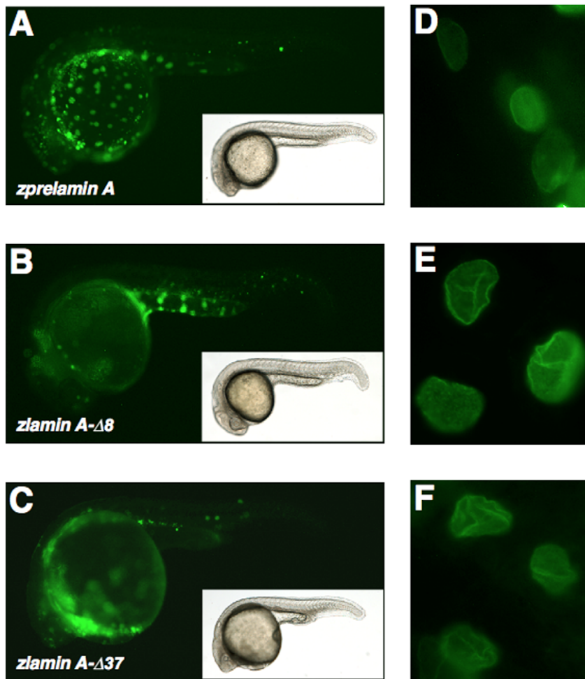
Figure 3. Expression of EGFP-tagged zprelamin A, zlamn A- \Delta 8, and zlamn A- \Delta 37/zProgerin in zebrafish embryos and the nuclear morphologies in the expressing cells. (A) EGFP-zprelamin A expression in zebrafish embryos. (B) EGFP-zlamn A- \Delta 8 expression in zebrafish embryos. (C) EGFP-zlamn A- \Delta 37/zProgerin expression in embryos. (D) The nuclear localization of EGFP-zprelamin A and the nuclear morphology in the expressing cells within the embryo. (E) The nuclear localization of EGFP-zlamn A- \Delta 8 and the nuclear morphology in the expressing cells within the embryo. (F) The nuclear localization of EGFP-zlamn A- \Delta 37/zProgerin and nuclear morphology in the expressing cells within the embryo. doi:10.1371/journal.pone.0017688.g003
