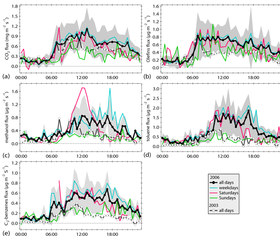
Fig. 3. Average diurnal patterns of the flux of (a) \text{CO}_2 , (b) mix of olefinic VOCs as propylene detected by the FOS, (c) methanol, (d) toluene, and (e) \text{C}_2 -benzenes for the entire study, weekdays, Saturdays and Sundays. The fluxes measured in 2003 at the CENICA site are included as reference. The grey shadows represent \pm 1 standard deviation from the total 2006 averages, and give an indication of the day-to-day variability in each phase of the daily cycle. The time scale corresponds to the local standard time.
