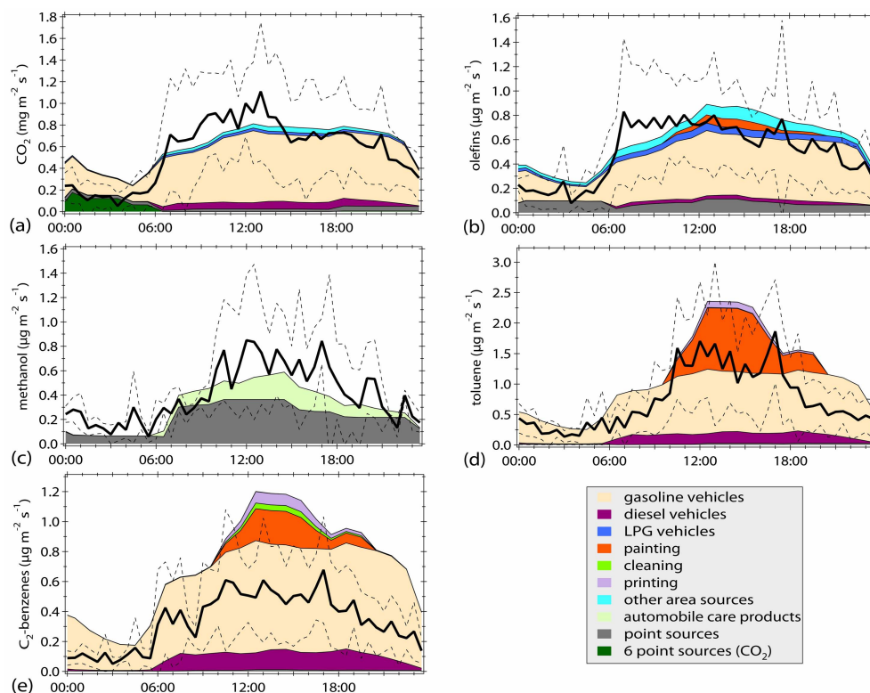
Fig. 9. Diurnal emission profiles distributed by source types for CO 2 (a), olefins (b), methanol (c), toluene (d), and C 2 -benzenes (e). The emissions of CO 2 , olefins, toluene and C 2 -benzenes were extracted from the grid cells coinciding with the 6-h footprints obtained for different periods of the diurnal course, while the methanol emissions represent the 63 surrounding cells. The black lines correspond to the average fluxes measured during the entire field campaign, while the dashed lines indicate \pm 1 standard deviation of the measured fluxes.
