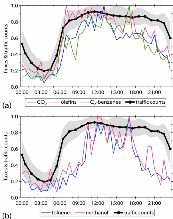
Fig. 7. Diurnal profiles of normalized traffic counts and fluxes of CO 2 , olefins, and C 2 -benzenes (a), and toluene and methanol (b). The traffic counts represent the average traffic from 11 roadways in a 10 km radius from the flux tower site. The gray shadow indicates \pm 1 standard deviation from the traffic counts. The time scale corresponds to the local standard time.
