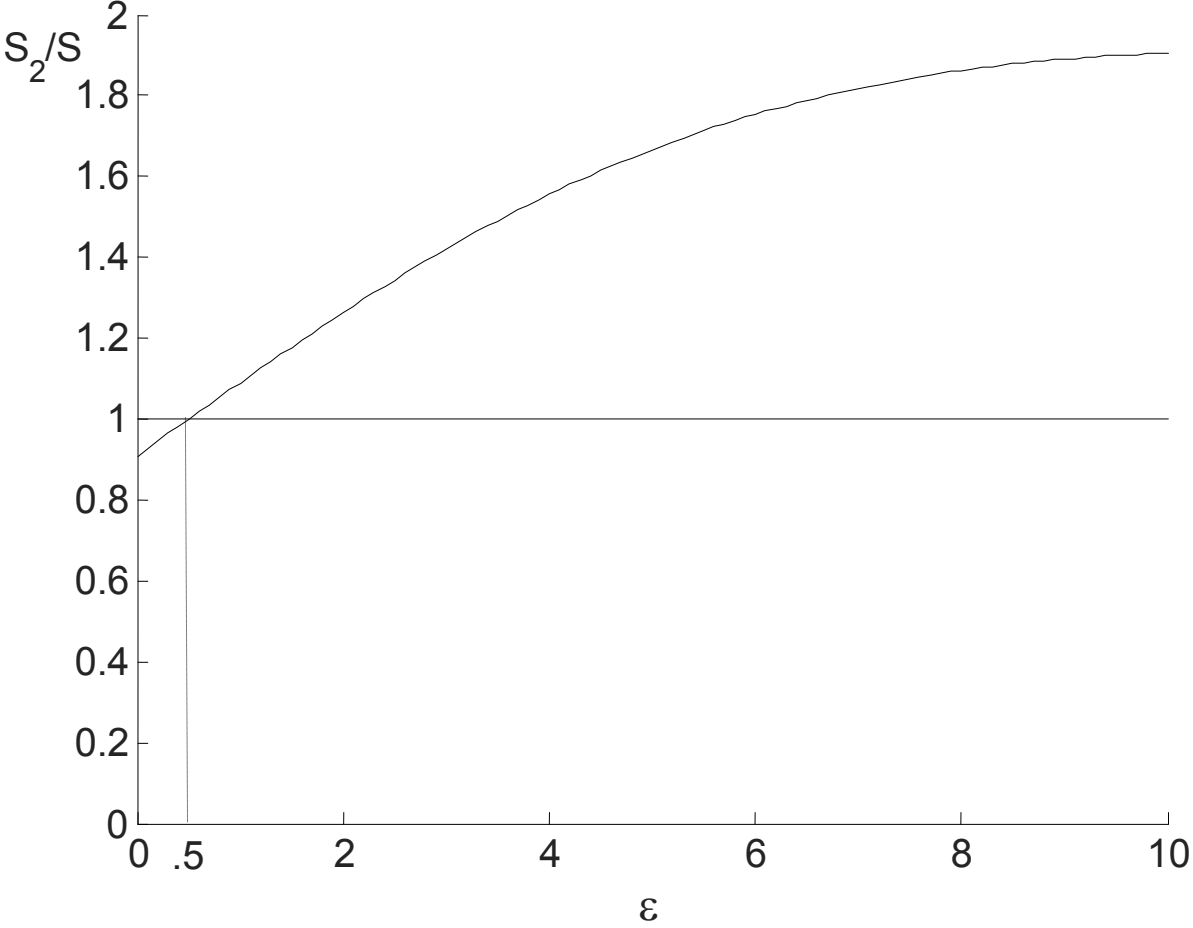
Figure 1: Increase in Sunk Cost, S_2/S
