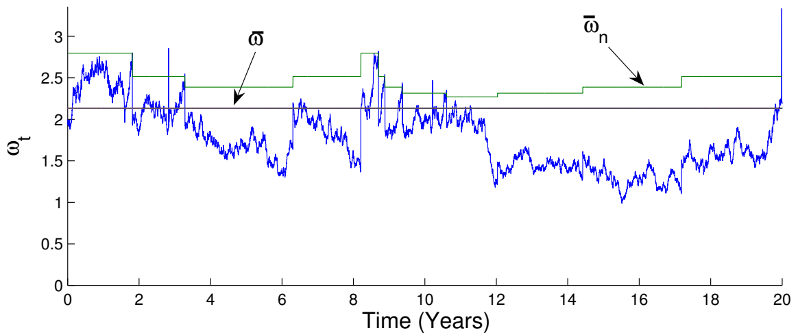
Figure 4: Sample Path: \lambda = 0.1
