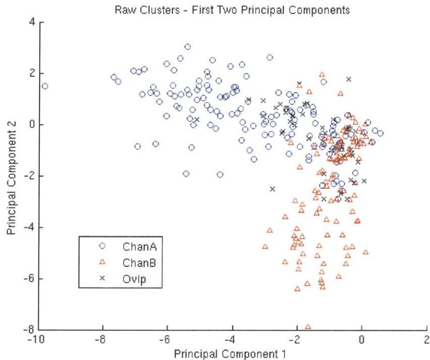
Figure 4-9: Plot of the first two dimensions (principal components) of rotation-only PCA-projected speaker i -vectors. The triangles in red represent i -vectors of a male speaker, while the blue circles represent i -vectors of a female speaker in the same conversation. The black x 's correspond to i -vectors representing overlapped speech.
