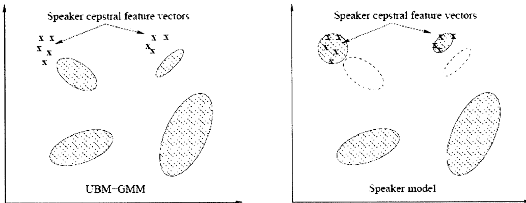
Figure 3-1: Depiction of maximum a posteriori (MAP) adaptation, taken from [2, 3].
