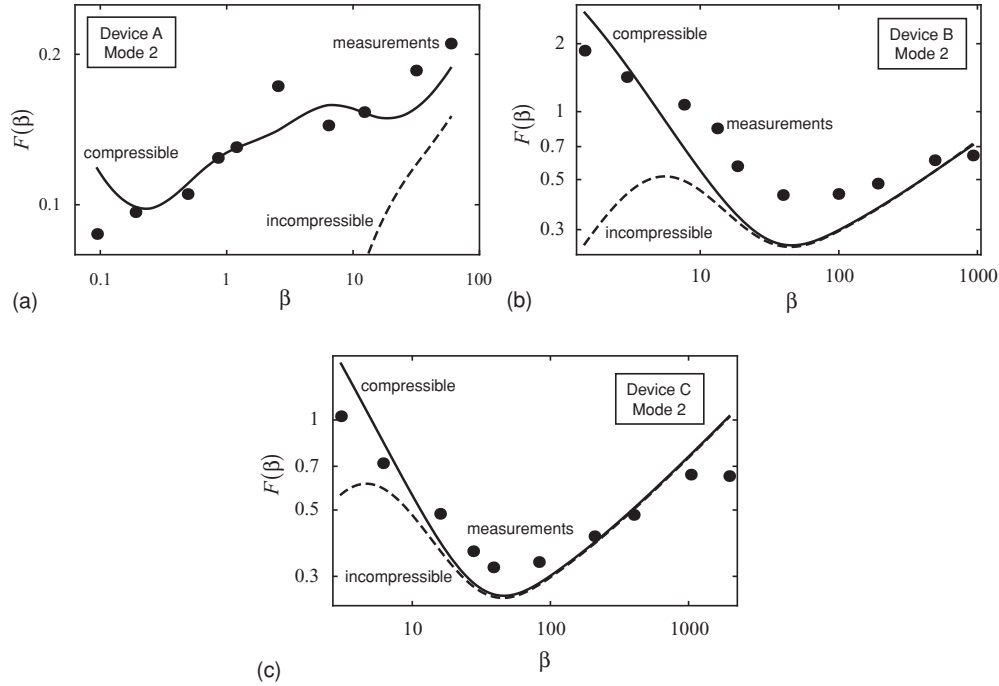
FIG. 13. Second mode (mode 2). Comparison of theoretical model (lines) to measurements (solid circles) for devices A, B, and C. The off-axis placement for each device: A ( \bar{Z}_0 = 0.5 ); B ( \bar{Z}_0 = 0.1 ); C ( \bar{Z}_0 = 0.09 ). Solid line (compressible fluid–finite speed of sound). Dashed line (incompressible fluid–infinite speed of sound).
