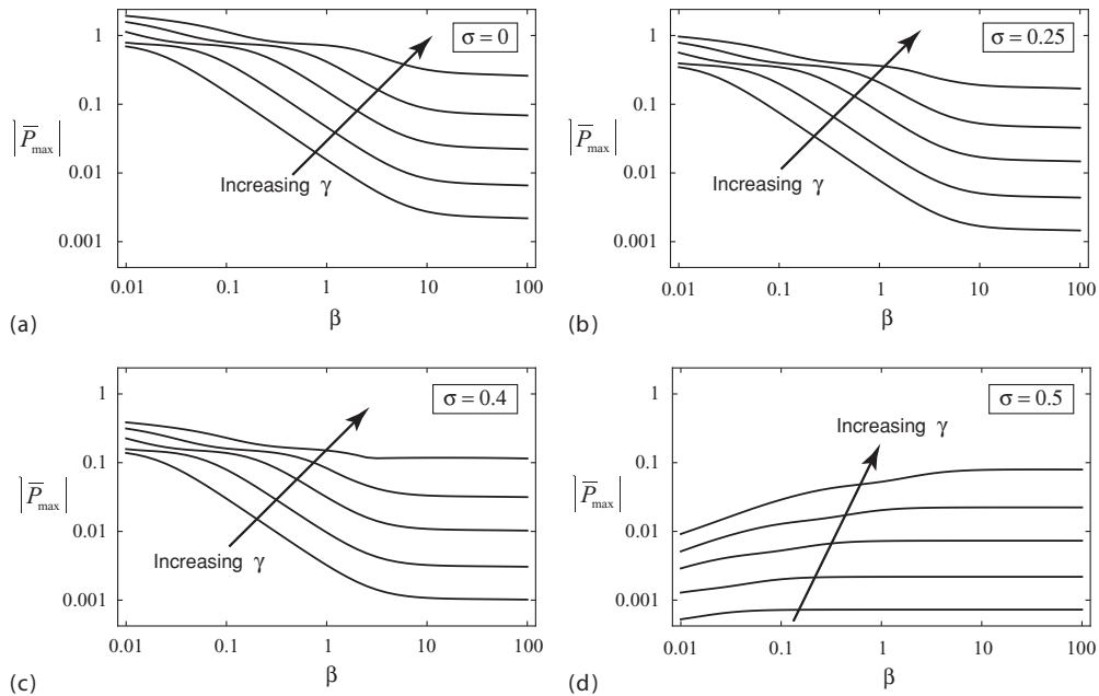
FIG. 11. Magnitude of normalized maximum pressure |\bar{P}_{\max}| within the rigid channel-cantilever system for various normalized acoustic numbers \gamma = 0.001, 0.003, 0.01, 0.03, 0.1 and Poisson's ratios: (a) \sigma = 0 , (b) \sigma = 0.25 , (c) \sigma = 0.4 , and (d) \sigma = 0.5 . The pressure scale is P_s = \rho_0 c^2 u_s / (\omega L) and is appropriate for the low inertia compressible limit, i.e., \beta \ll 1 and \alpha \gg 1 [21]. The length of the rigid lead channel equals the cantilever length, i.e., L_c = L . Identical axis scales have been used in each figure to assist comparison.
