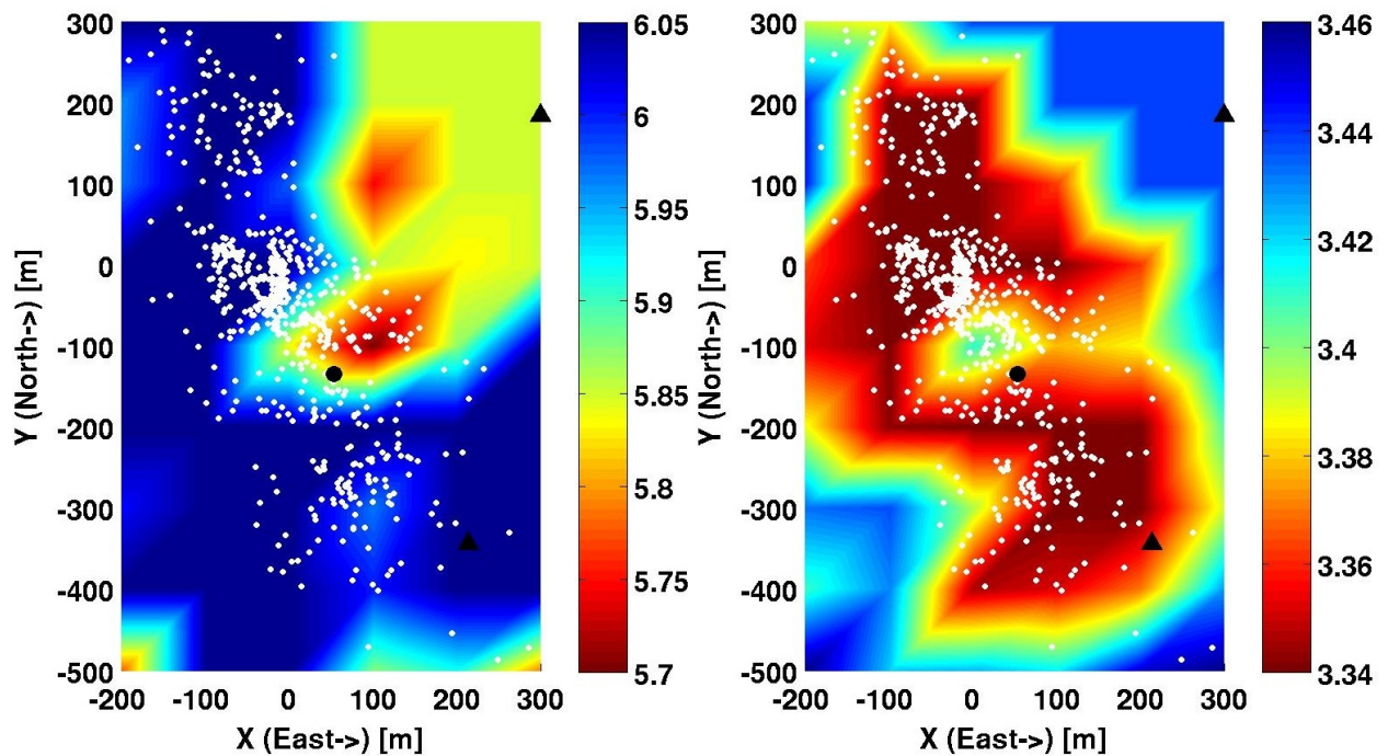
Figure A.21: Horizontal velocity model slices for P and S wave velocities at 3200 meters depth in km/sec. Black circle denotes the position of the injection well GPK1. Black triangles show the locations of station 4550 (upper right) and hyd1 (lower right). White dots denote final earthquake locations within fifty meters depth.
