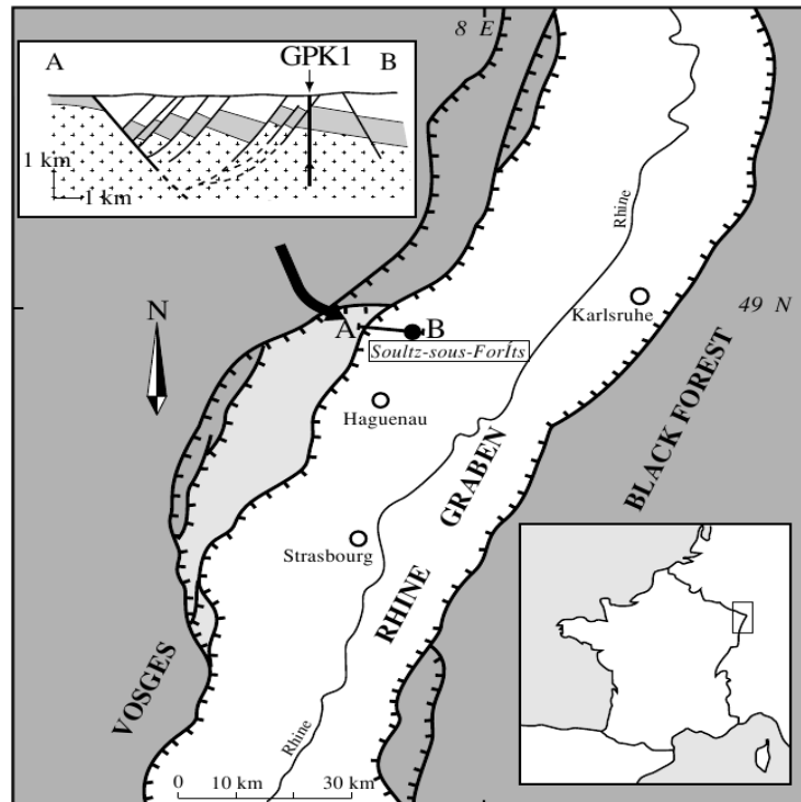
Figure 1.3: Regional overview of location of Soutz EGS reservoir from Evans et al. (2005). Upper left inset shows a cross-sectional view from A-B with GPK1 and the main geologic sections (granite denoted by crosses, Mesozoic sediments in light gray, and Oligocene and Miocene sediments in white). Lower right inset shows the location of the expanded view relative to France.
