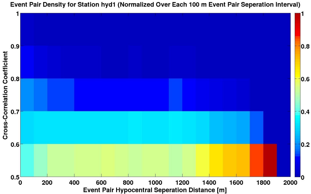
Figure 2.22: Density of event pairs based on their relationship between event pair hypocentral separation distance and cross-correlation coefficient for station hyd1. Note that each cell represents the percentage of event pairs within the range of CC coefficients at the given 100 m interval in hypocentral separation distance.
