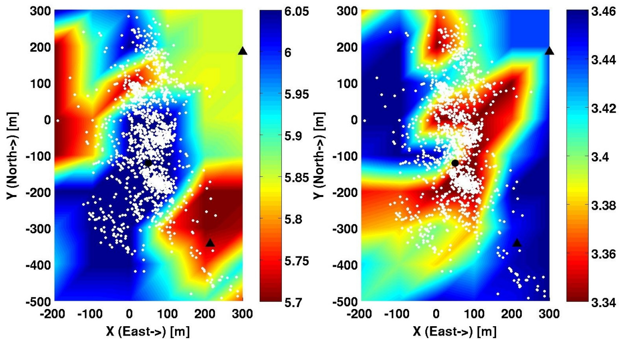
Figure A.31: Horizontal velocity model slices for P and S wave velocities at 2900 meters depth in km/sec. Black circle denotes the position of the injection well GPK1. Black triangles show the locations of station 4550 (upper right) and hyd1 (lower right). White dots denote final earthquake locations within fifty meters depth.
