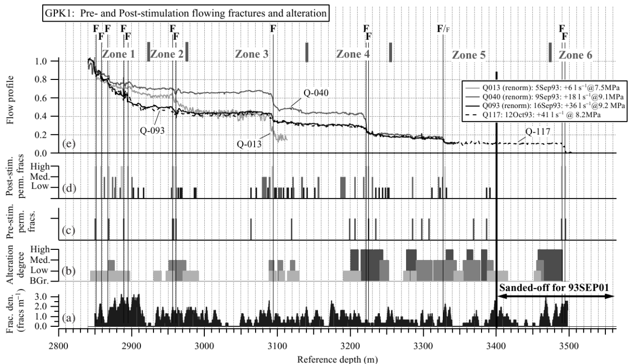
Figure 1.1: Flow profile (from spinner logs), pre and post-stimulation fractures, alteration degree, and fracture density plotted from 2800 to 3600 meters depth for the September 1993 Soutiz EGS hydraulic stimulation, from Evans et al. (2005).
