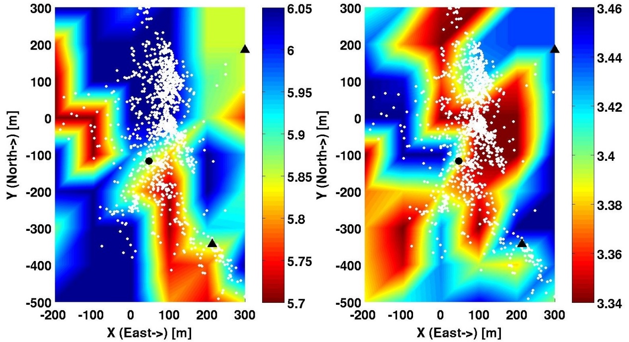
Figure A.30: Horizontal velocity model slices for P and S wave velocities at 2800 meters depth in km/sec. Black circle denotes the position of the injection well GPK1. Black triangles show the locations of station 4550 (upper right) and hyd1 (lower right). White dots denote final earthquake locations within fifty meters depth.
