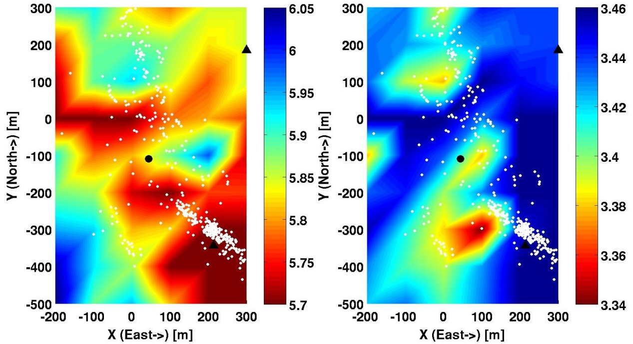
Figure A.41: Horizontal velocity model slices for P and S wave velocities at 2600 meters depth in km/sec. Black circle denotes the position of the injection well GPK1. Black triangles show the locations of station 4550 (upper right) and hyd1 (lower right). White dots denote final earthquake locations within fifty meters depth.
