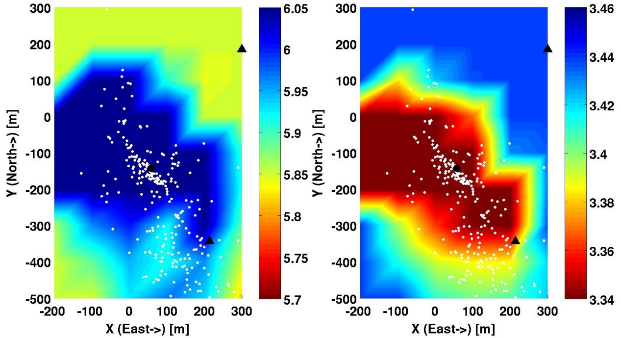
Figure A.49: Horizontal velocity model slices for P and S wave velocities at 3400 meters depth in km/sec. Black circle denotes the position of the injection well GPK1. Black triangles show the locations of station 4550 (upper right) and hyd1 (lower right). White dots denote final earthquake locations within fifty meters depth.
