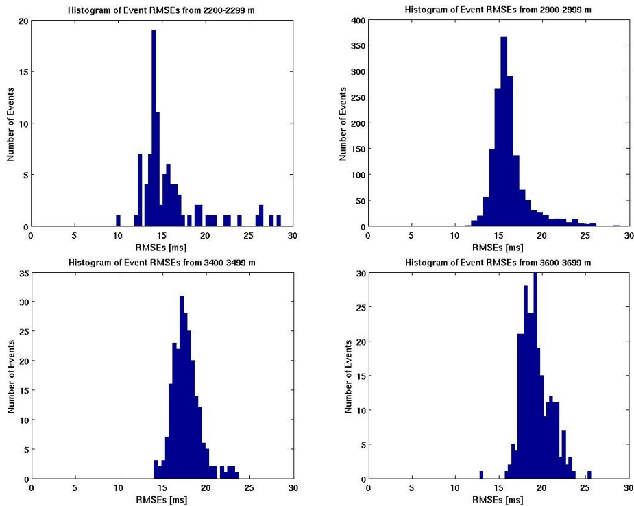
Figure 2.7. Histograms of event RMSE for different depth intervals. Note how the center of the main event distribution shifts towards higher RMSE with increasing depth.
