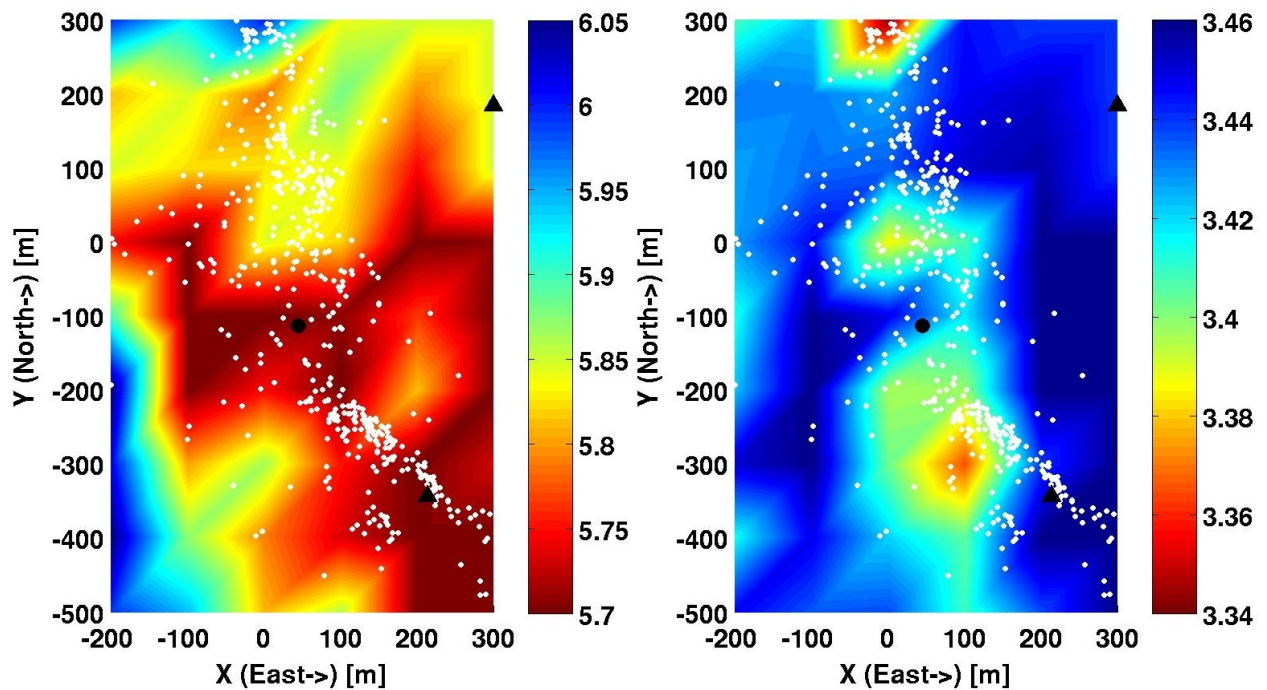
Figure A.42: Horizontal velocity model slices for P and S wave velocities at 2700 meters depth in km/sec. Black circle denotes the position of the injection well GPK1. Black triangles show the locations of station 4550 (upper right) and hyd1 (lower right). White dots denote final earthquake locations within fifty meters depth.
