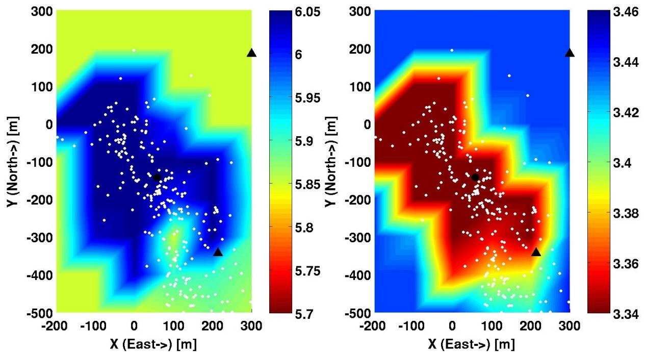
Figure A.50: Horizontal velocity model slices for P and S wave velocities at 3500 meters depth in km/sec. Black circle denotes the position of the injection well GPK1. Black triangles show the locations of station 4550 (upper right) and hyd1 (lower right). White dots denote final earthquake locations within fifty meters depth.
