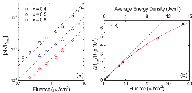
FIG. 4. (Color online) (a) |\Delta R/R|_{\text{max}} plotted as a function of \Phi at T = 7 \text{ K} for the x = 0.4 - 0.6 samples, each offset for clarity. Dashed lines show a slope of 1. Linear behavior in the low-fluence regime is an indication that the optically accessed excitations are fully gapped, as described in the text. (b) The absolute value of the maximum change in reflectivity versus both \Phi and the average energy absorbed within a penetration depth for the x = 0.4 sample. The red curve is a fit to a simple saturation model yielding \Phi_{\text{sat}} = 25 \text{ μJ/cm}^2 at an initial temperature of 7 K.
