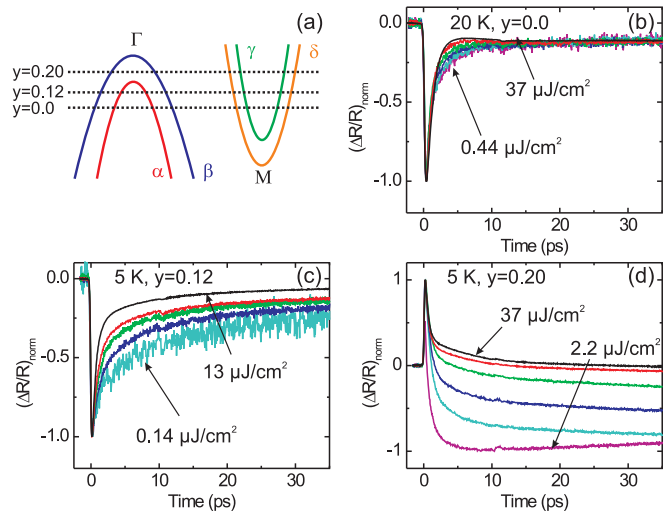
FIG. 11. (Color online) (a) Schematic representation of the band structure of the Ba-122 pnictides. Although this is somewhat of a simplification that ignores the change in k_z dependence with doping, 47 the predominant effect is a shift of the Fermi level up with the addition of electrons: 45 in the parent compound, \alpha and \gamma, \delta nest, leading to SDW behavior. In the underdoped regime ( y = 0.12 ), \alpha does not nest appreciably with \gamma, \delta . With the addition of more holes, the \alpha band is submerged below the Fermi level when the doping reaches y = 0.15 , as measured by Sekiba et al. 46 (b) Raw (\Delta R/R)_{\text{norm}} traces for the parent compound at 20 K. The moderate amount of intensity dependence in these traces at short times is due to acoustic suppression from the diminished thermal expansion parameter at lower temperatures/fluences. (c) Reflectivity transients in the underdoped sample ( y = 0.12 , T_c = 12 K) show a mild amount of intensity dependence of the faster relaxation with increasing fluence, similar to that seen in the hole-doped samples. (d) Fluence dependence of the optimally doped sample ( y = 0.2 , T_c = 22.5 K) indicates entirely different relaxation dynamics with fluence. While there appears to be intensity dependence present here, the slope of the initial transient \gamma_0 is identical for all fluences. The differences between the various fluences and the origin of this nonuniformity of the relaxation dynamics are due to a temperature effect, as described in the text.
