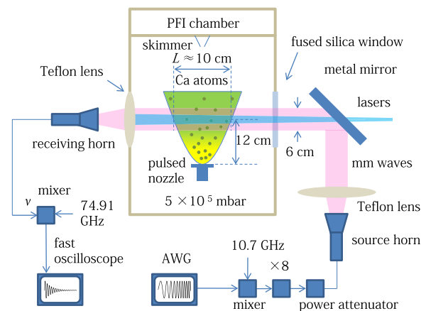
FIG. 1 (color online). Rydberg CPmmW experimental setup. Ca atoms are produced by laser ablation and supersonically co-expanded with He gas into vacuum [19]. The diverging laser beams, delivered through a 12 mm aperture in the metal mirror, excite Ca atoms to a selected Rydberg state. The chirped mm-wave pulses are broadcast from the source horn, and the FID is collected by the receiving horn. The pulsed lasers and gas nozzle operate at a 20 Hz repetition rate, and are synchronized with the mm-wave pulses.
