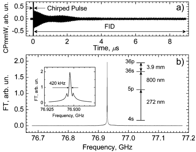
FIG. 2. CPmmW spectrum of Ca atoms. (a) The 10 ns duration, 3.9 V/m ( \approx 1.4 \times 10^{-5} W), 0.5 GHz bandwidth chirped pulse centered around the \nu = 76.9293 GHz 36p - 36s transition [21], is followed by FID. Fine modulation is due to the 10 MHz frequency standard [16]. (b) The spectrum is a (rectangular window) magnitude Fourier transform of the FID. The inserts show an up-close view of the line, which is split into the three Zeeman components with \Delta\nu_{\text{FWHM}} = 420 kHz of the central peak, and the level diagram of Ca atoms.
