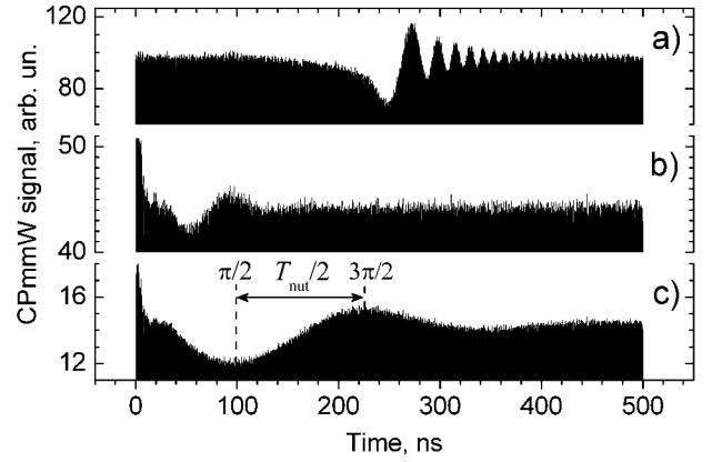
FIG. 3. Millimeter-wave transient nutations (only the top portion is shown). (a) The FID is initiated when the frequency of the chirped excitation pulse (500 ns duration) tunes through the Rydberg-Rydberg resonance. The frequency of the chirp is swept linearly in time away from resonance while that of the FID is constant; hence the frequency of the beat increases. (b), (c) Single frequency excitation pulse. (b) \mathcal{E}_0 = 0.69 V/m is determined by measuring T_{\text{nut}} = 84 ns; (c) \mathcal{E}_0 = 0.23 V/m, T_{\text{nut}} = 250 ns. When deducing \mathcal{E}_{\text{FID}} we took into account that approximately 60% of the detected signal comes from the mm waves that pass outside of the interaction volume.
