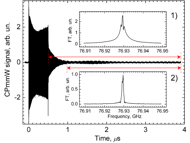
FIG. 4 (color online). Evidence of superradiant decay. The excitation pulse (0–0.5 \mu\text{s} ) followed by FID (superradiance) (0.5–3.9 \mu\text{s} ) is a continuation of the Figs. 3(b) and 3(c) series with \mathcal{E}_0 = 0.039 V/m ( \approx 1.4 \times 10^{-9} W), as determined by the tunable power attenuator. The line splitting in (1) is due to Zeeman effect. The observed (1/e) decay time of 190 ns is close to the predicted T_{\text{sr}} = 350 ns. The inserts show Fourier transforms of different time intervals of the time-domain signal. (1) 0.5–3.9 \mu\text{s} : broader, Lorentzian-type line shape; (2) 1.0–3.9 \mu\text{s} : narrower, Gaussian-type line shape. This measurement is consistent with fast initial superradiant decay followed by slower, Doppler dephasing.
