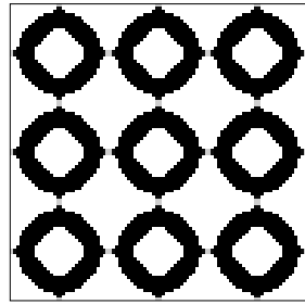
(a) Optimized crystal structure
