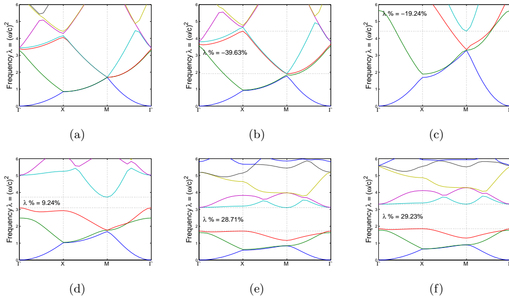
Figure 18: The corresponding band structure (of Figure 17)) and the gap-midgap ratio between \lambda_{TE}^3 and \lambda_{TE}^4 in the square lattice.
