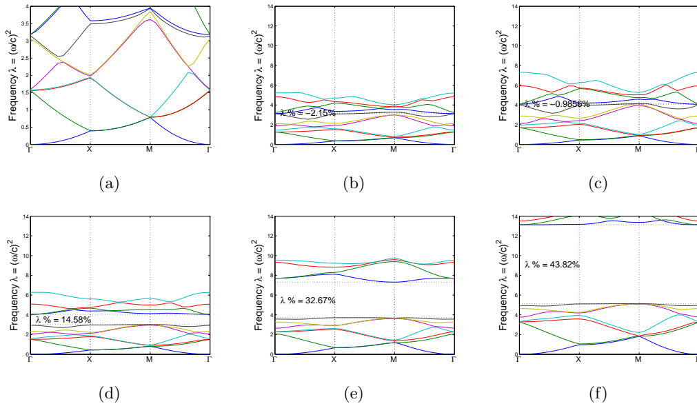
Figure 16: The corresponding band structure (of Figure 15)) and the gap-midgap ratio between \lambda_{\text{TM}}^7 and \lambda_{\text{TM}}^8 in the square lattice.
