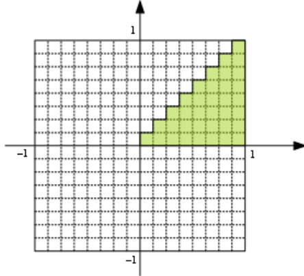
Figure 2: An illustration of a coarse mesh ( 16 \times 16 ) and dielectric function for the square lattice. The shaded cells indicate the decision variables relating the dielectric material ( \varepsilon_i, i = 1, 2, \dots, n_\varepsilon ). Note that the actual computational mesh ( 64 \times 64 ) is finer than this one.
