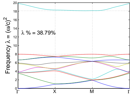
(b) Optimal band structure
