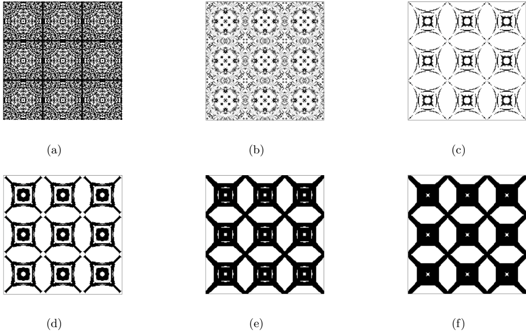
Figure 17: The evolution of the square lattice crystal structure for optimizing the gap-midgap ratio between \lambda_{TE}^3 and \lambda_{TE}^4 .
