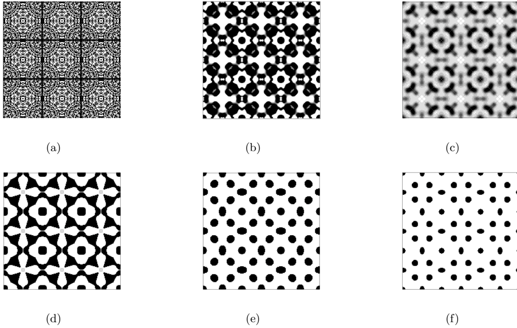
Figure 15: The evolution of the square lattice crystal structure for optimizing the gap-midgap ratio between \lambda_{\text{TM}}^7 and \lambda_{\text{TM}}^8 .
