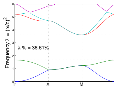
(b) Optimized band structure
