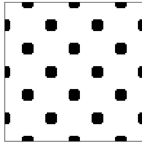
(a) Optimized crystal structure
