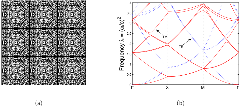
Figure 14: (a) Random starting structure with translation, rotation, and reflection symmetry, 3 \times 3 unit cells in square lattice. (b) Band structure before optimization.
