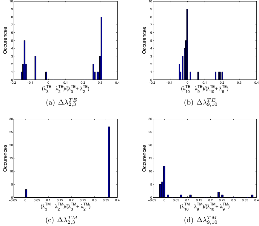
Figure 5: Histograms of gap-midgap ratios for 30 runs with random initial configurations, for the second and ninth bands.
