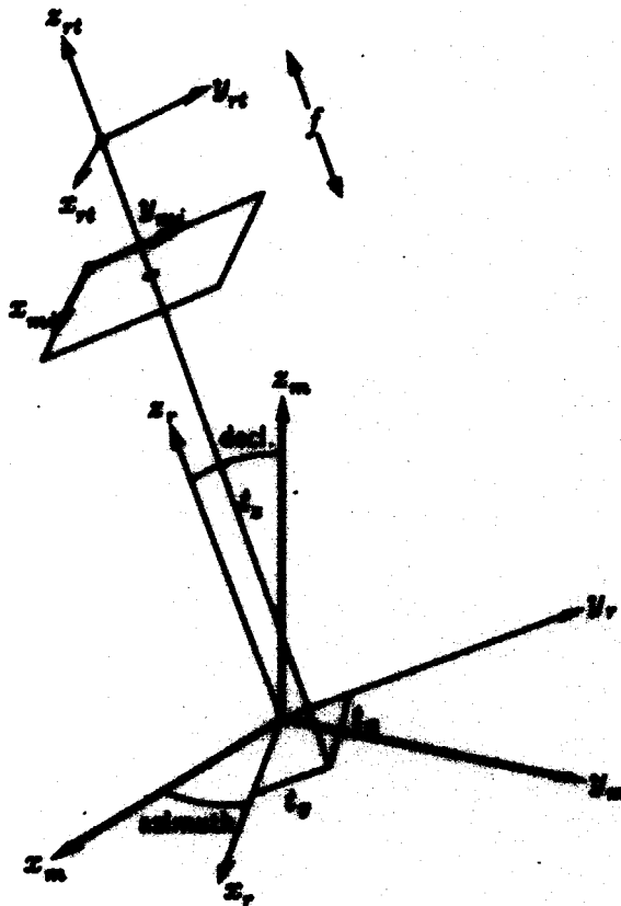
Figure 5.6: The coordinate frames used for rotating, translating, and projecting a model point into the image.
