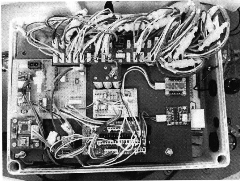
Figure 2-12: Photograph of kayak electrical system. The enclosure contains the batteries, battery and power distribution boards, Arduino microcontroller, sensor board, and XBee radios.
