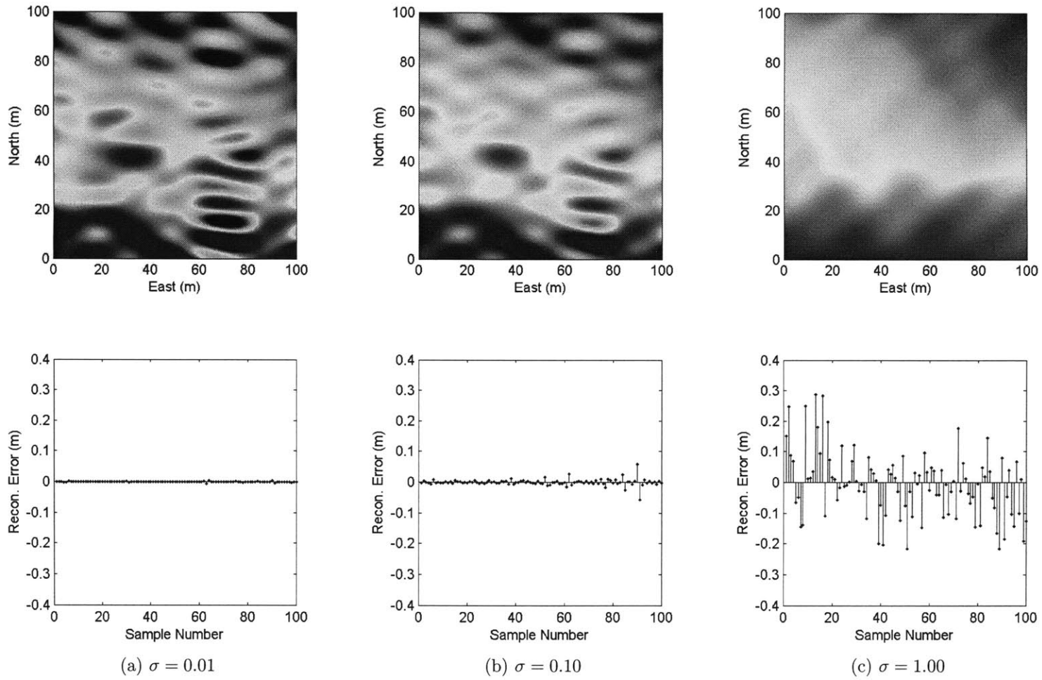
Figure 4-13: CS reconstruction error. These reconstructions correspond to the second row in Fig. 4-12, with the number of basis coefficients equal to 450. Here, the top row shows the reconstructed field, and the bottom row shows the difference between the measurements and the reconstructed field at the measurement locations. Columns (a), (b), and (c) give the reconstruction results for measurement errors ( \sigma ) equal to 0.01, 0.10, and 1.00, respectively.
