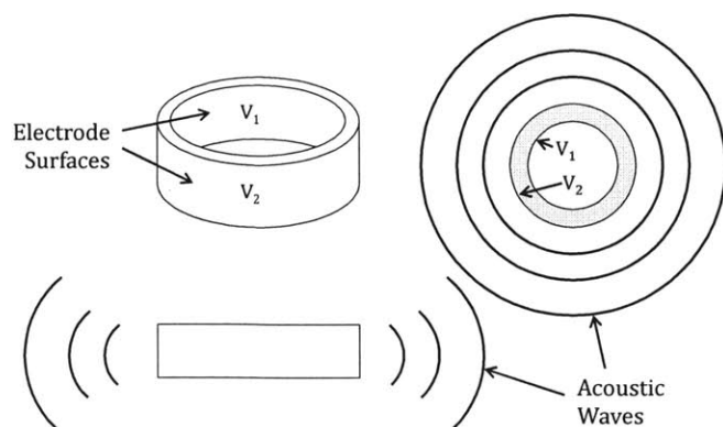
Figure 3-3: Illustration of radially-expanding piezoelectric ceramic ring transducer. An electric signal is across the electrodes on the inner and outer surface of the cylinder, causing a radial deformation that produces acoustic waves. The waves are omnidirectional in the horizontal plane.
