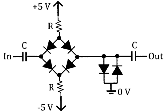
Figure 3-12: Schematic of transmit/receive switch. The AC-coupled diode bridge is connected to each of the transducer inputs on the receiver. The switch protects the receive circuitry from the transmission-level voltages would cause damage. The diodes do not block low voltages such as those present when receiving an acoustic signal.
