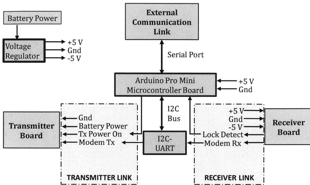
(a) Interface Board Schematic
