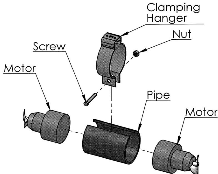
Figure 2-5: Motor-propeller assembly. The propeller is attached to the motor with a custom coupling. The quantity of the coupling required per raft (8) motivated design for minimum machining steps. The part requires one cutoff operation, two drilling operations, and two tapping operations. Its production was outsourced for the price of three dollars per part for 34 pieces.
