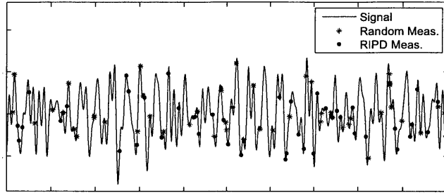
Figure 4-7: A representative signal of measurement point selection in the 1D case with discrete cosine transform. Fifty points are selected randomly, or designed according to the RIP, with one-hundred candidates considered for each addition.
