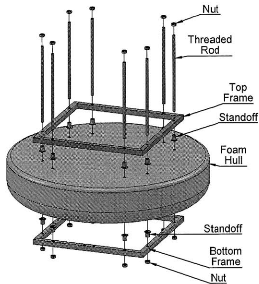
(a) CAD view of raft frame
