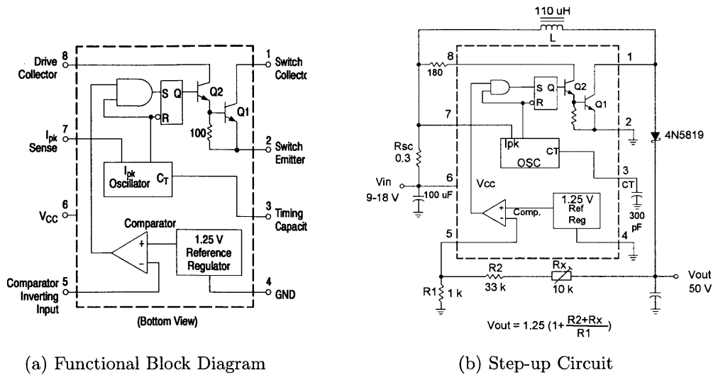
Figure 3-9: Voltage regulator circuit. The voltage regulator boosts the battery voltage to 50 volts to amplify the transmission signal. The regulator is built using an MC34063 Buck Boost Inverting Switching Regulator IC from ON Semiconductor. The values of the discrete components are calculated using design equations included in the data sheet for the chip. The potentiometer, R_X , is used for fine-scale adjustment of the output voltage. Schematic from MX34063 datasheet.
