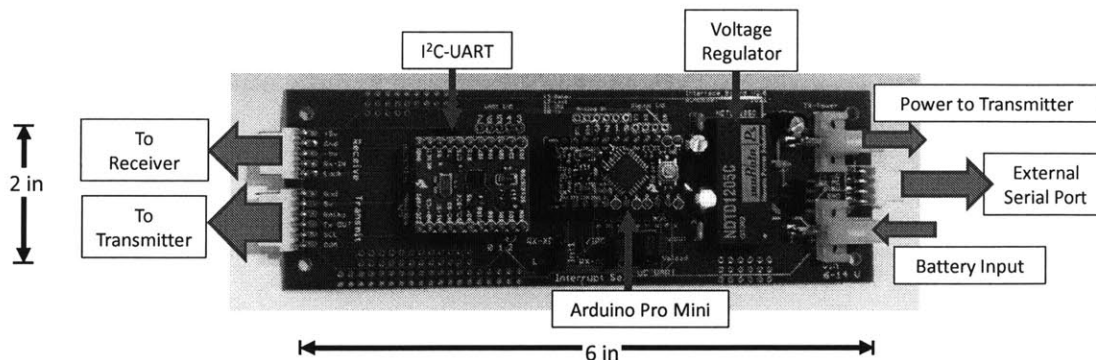
(b) Interface Board PCB
