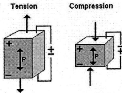
Figure 3-1: Illustration of the piezoelectric effect. A positive electric potential across the material results in a positive displacement (tension). A negative potential results in a negative displacement (compression). The effect is also reversible – a deformation of the material results in an electric potential across it. Image from [34].
