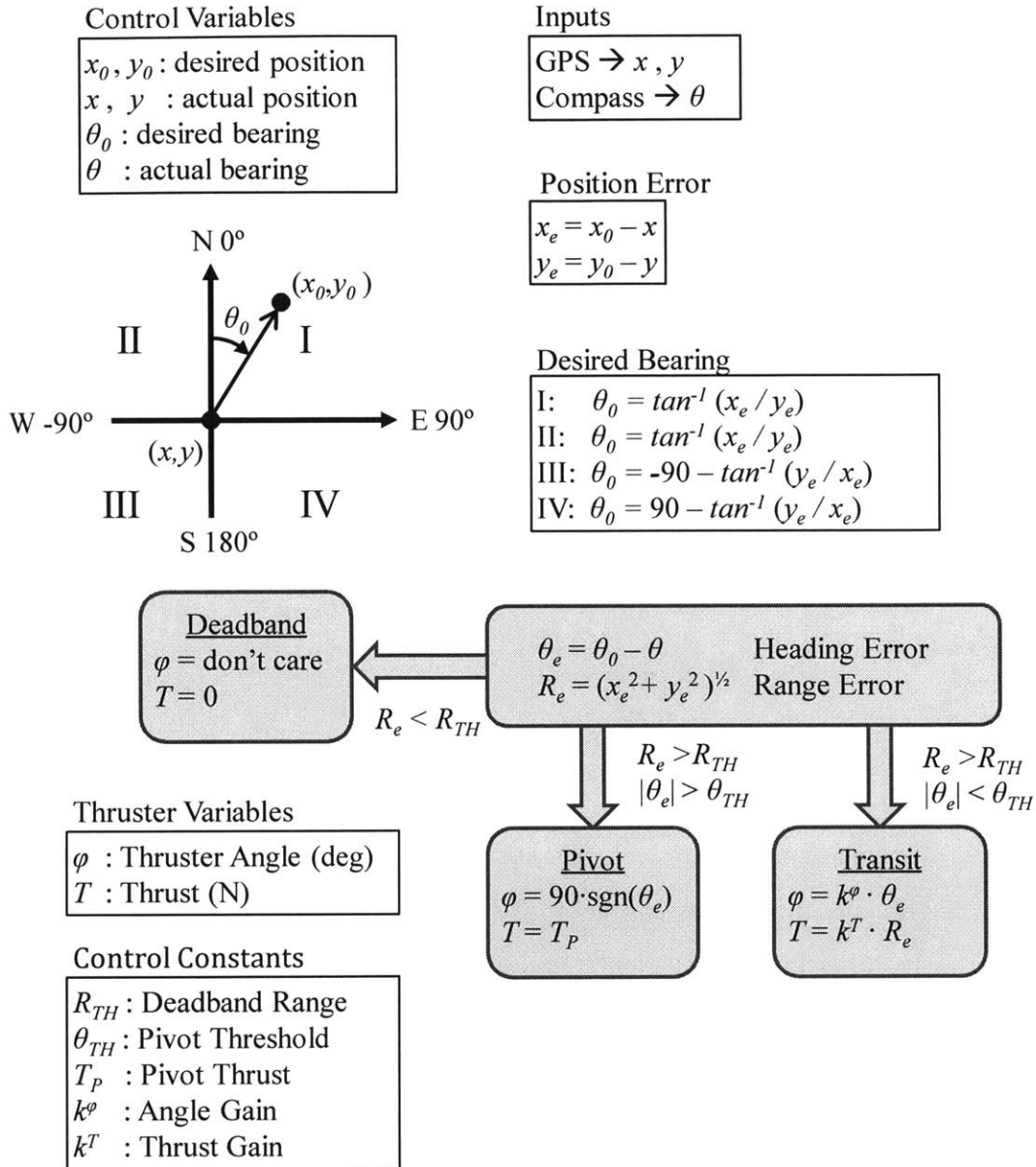
Figure 2-20: Description of kayak position control system. The desired position is set by the user with a set of one or several waypoints. The kayak measures its position with GPS and heading with a MEMS compass. Depending on the range and heading error, the controller enters one of three modes. If range error is minimal, the vehicle enters deadband mode and no control actions are performed. Otherwise the vehicle enters either pivot or transit mode. If heading error is large, pivot mode is used to rotate the vehicle until aimed at the target. When heading error is small, the vehicle uses transit mode with proportional control of heading and thrust. The thrust gain in transit mode results in full output power if range error is more than about ten meters, resulting in full-speed transit with proportional heading control.
