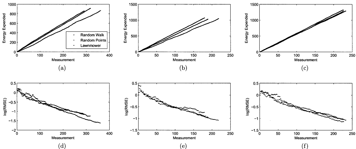
Figure 4-5: Results for Scenario 1 (a) and (d), Scenario 2 (b) and (e), and Scenario 3 (c) and (f). Plots (a)-(c) show energy expenditure as a function of the number of measurements taken. Plots (d)-(f) show the logRMSE as a function of the number of measurements. Scenario 1 - Inexpensive Measurements and Large Domain. Scenario 2 - Inexpensive Measurements and Small Domain. Scenario 3 - Expensive Measurements and Small Domain. In Scenario 1, the random TSP is more efficient, taking more measurements and also achieving a better reconstruction error. In Scenario 2, the random TSP is again more efficient and achieves a better final reconstruction error; however, for a given number of measurements, the random walk performs equally well. In Scenario 3, all strategies are similarly efficient, and here the random TSP is superior given the same number of measurements. The lawnmower performs similarly to the random walk in Scenarios 1 and 3. In Scenario 2 the random walk is superior to the lawnmower. Legend: Blue-random walk; Black-lawnmower ; Red-random TSP
