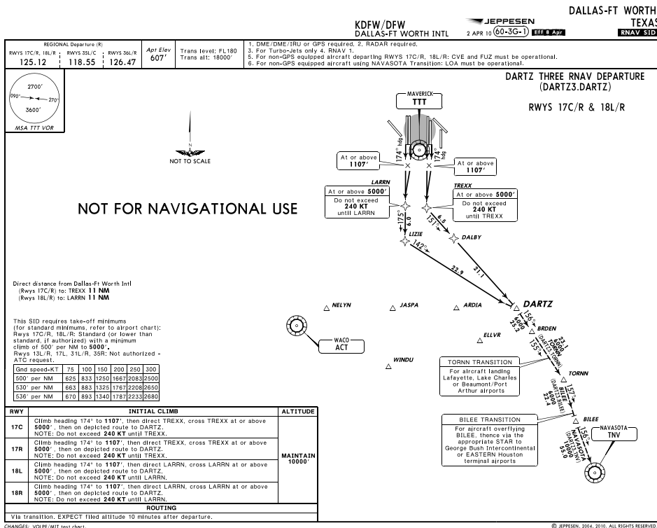
Figure 41. Example Jeppesen departure procedures (a) Current chart (b) Modified chart
