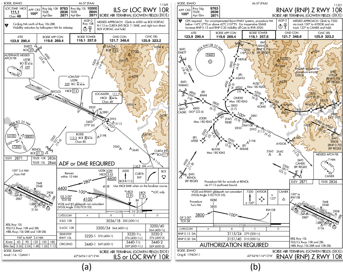
Figure 6. An example of conventional approach procedure (a) and RNP AR approach procedure (b) is shown.
