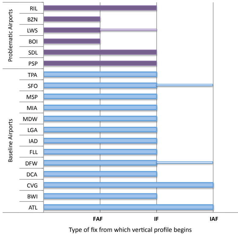
Figure 21. Vertical profile starting fix is shown for individual airport categorized by Problematic Group and Baseline Group. The shaded region shows the range of profile views at the airport
