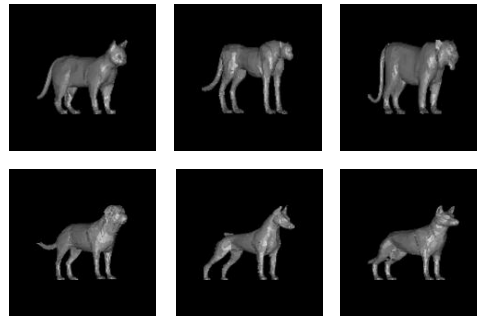
Figure 14: Cat/dog prototypes.
