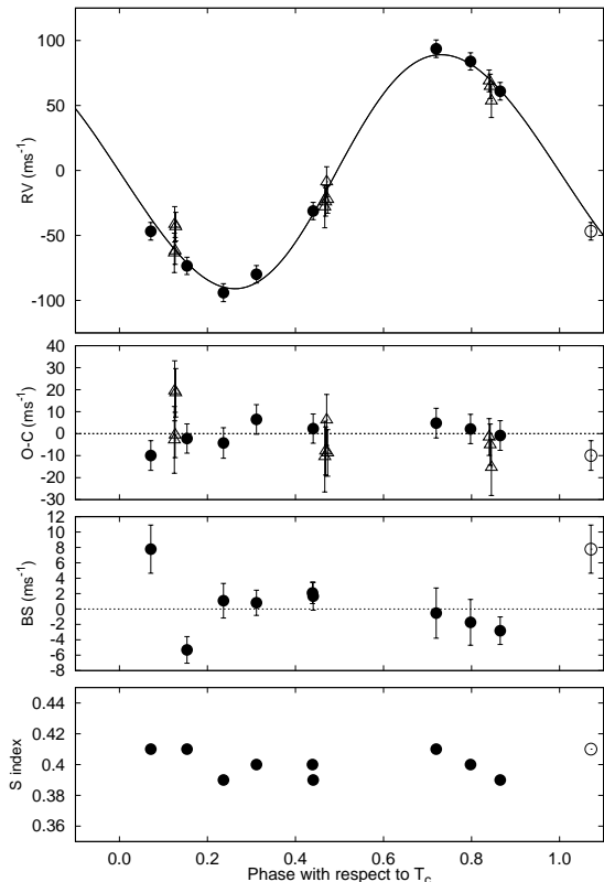
FIG. 2.— Top panel : Keck/HIRES RV measurements (filled circles) and Subaru/HDS RV measurements (open triangles) for HAT-P-30 shown as a function of orbital phase, along with our best-fit model (see Table 4). Zero phase corresponds to the time of mid-transit. The center-of-mass velocity has been subtracted. Second panel : Velocity O-C residuals from the best fit. The error bars include a component from astrophysical/instrumental jitter ( 6.3 \text{ m s}^{-1} for HIRES and 2.1 \text{ m s}^{-1} for HDS) added in quadrature to the formal errors such that \chi_p^2 = 1 (see Section 3.2). Third panel : Bisector spans (BS) for the HIRES spectra, with the mean value subtracted, and the measurement from the template spectrum is included. Bottom panel : Chromospheric activity index S measured from the Keck spectra. Note the different vertical scales of the panels. Observations shown twice are represented with open circles.
