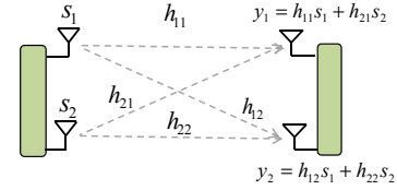
Figure 4—Decoding in a standard 2-by-2 MIMO system.
