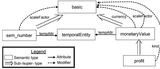
Fig. 4. A graphical representation of the example ontology
