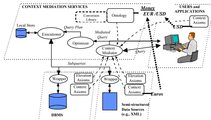
Fig. 3. Architecture of the COIN system
