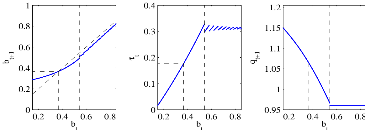
Figure 10: Decision Rules
