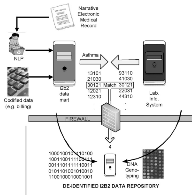
Figure 1. Matching anonymously identified populations to anonymous samples. An i2b2 datamart is generated from codified data (e.g., billing codes, laboratory test values) and concepts codified by running the narrative text in electronic medical records through a NLP tool, the HITex package described in the Methods section. Patients included within the i2b2 datamart meeting study criteria are selected and their corresponding set of identifiers are generated. Those identifiers are forwarded to the Crimson application, which scans recent transactions forwarded from one or more local clinical laboratory or pathology information systems to identify newly accessioned materials matching the cohort identifiers and desired sample types. Upon completion of diagnostic testing (1–3 d after collection in most cases), Crimson manages reaccession of the sample to a study’s IRB protocol and assigns the i2b2-forwarded subject ID to a uniquely generated sample ID. These actions remove all identifiers (accession no., medical record no., etc.) from the original sample. The sample may then be released to the investigator where it can be measured (for genome-wide genotyping in this instance), and these measurement data are merged with the phenotypic data set in the i2b2 datamart. Because of the electronic and regulatory firewalls, only research personnel approved by the IRB can view the limited data set (in the HIPAA sense), and they cannot view the identified clinical data visible to those who access the laboratory information system.
