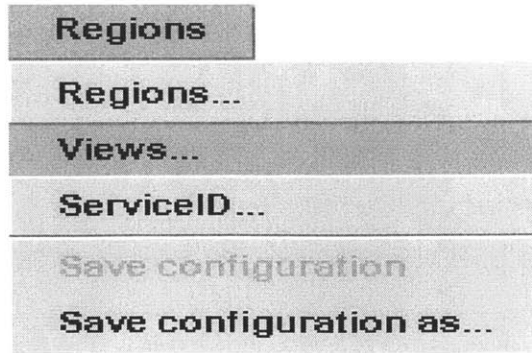
Figure 5-2: Region menu.
