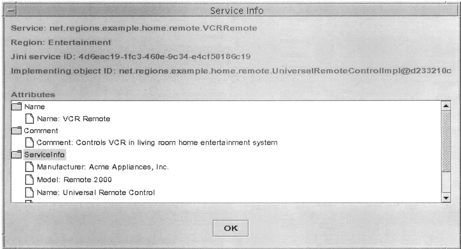
Figure 5-9: Service information for VCRRemote.
