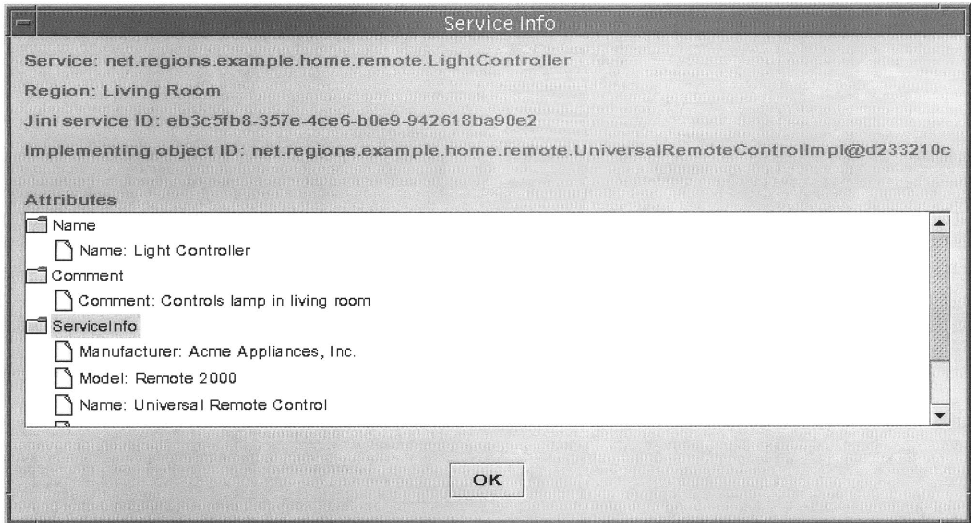
Figure 5-8: Service information for LightController.
