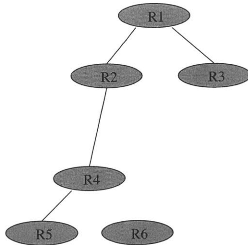
Figure 4-3: Top: Region R6 leaving region R4. Bottom: Region graph after R6 leaves.
