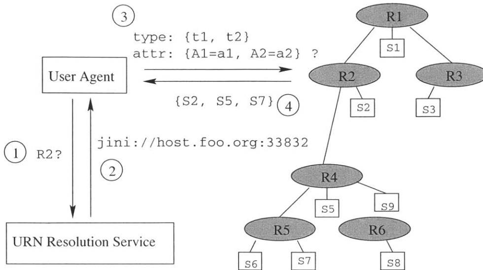
Figure 4-7: User agent querying region R2.
