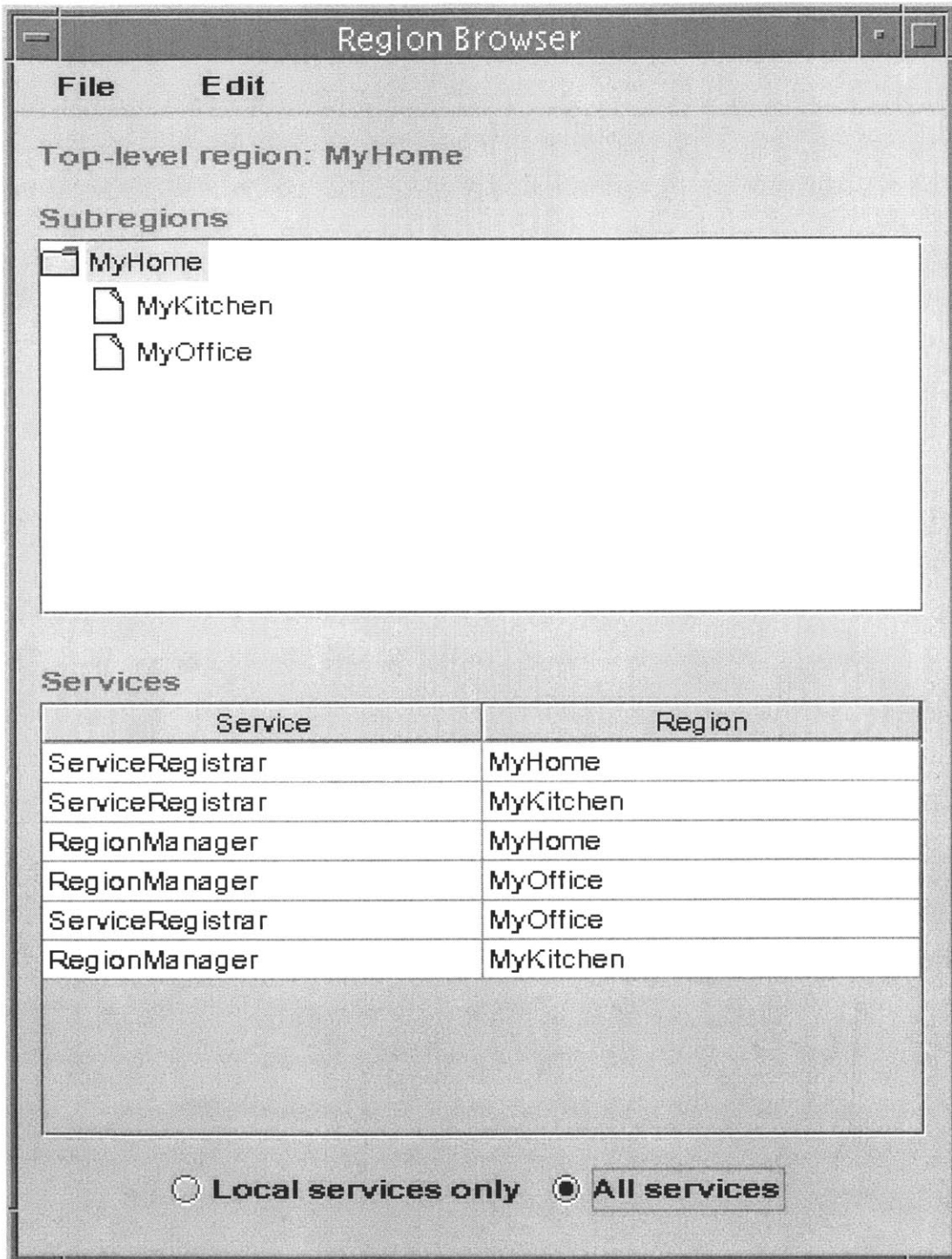
Figure 5-4: Region Browser.
