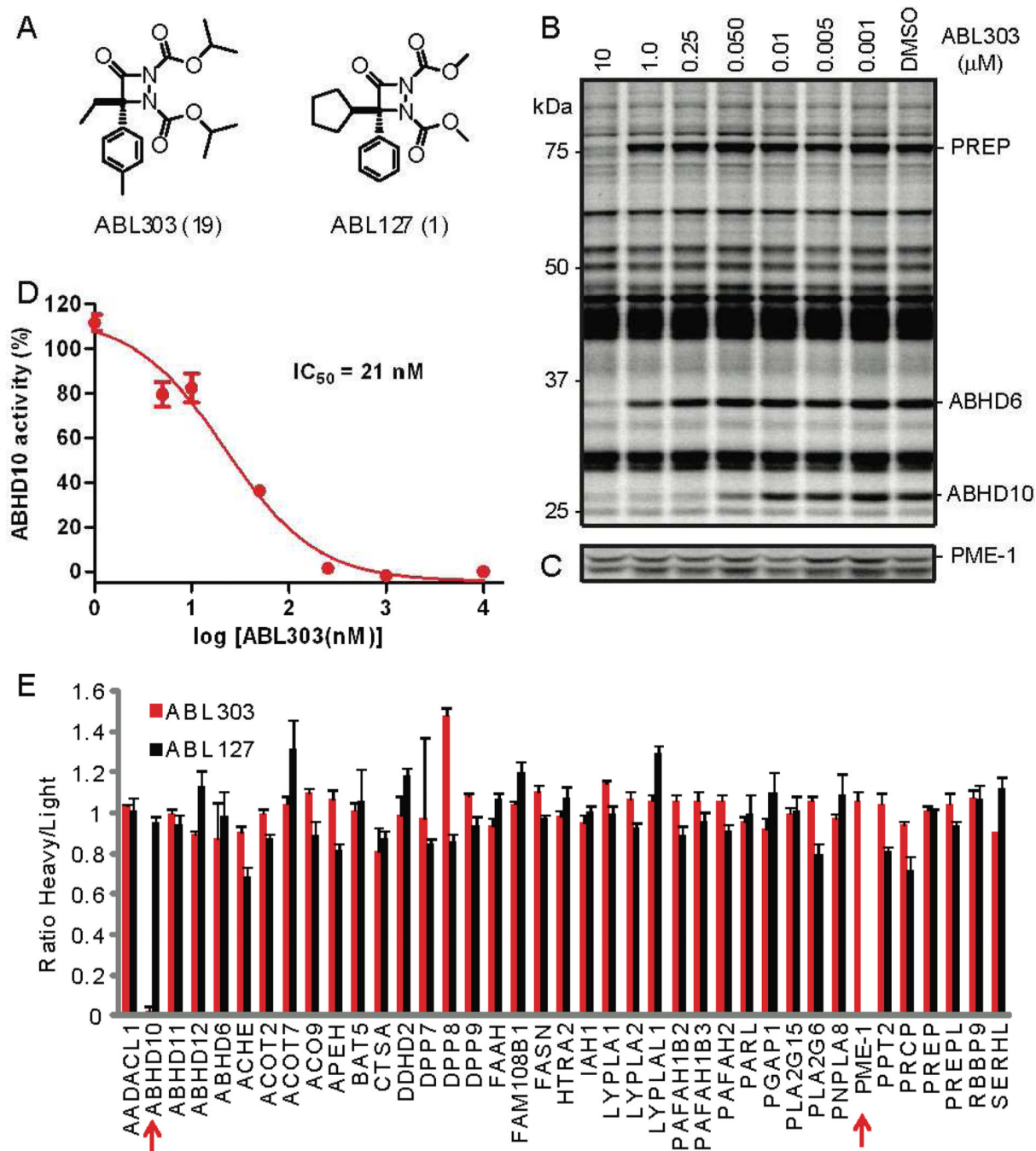
Figure 2. Competitive ABPP of ABL303 in situ. (A) Structures of ABL probes. (B and C) Gel-based ABPP of membrane (B) and soluble (C) proteomes from Neuro-2A cells treated with ABL303 (10 - 0.001 \mu\text{M} , 2 h), afforded an (D) IC 50 value of 21 nM for inhibition of ABHD10 and no significant inhibition of PME-1. Data are presented as mean values \pm SEM; n = 3/\text{group} . (E) ABPP-SILAC analysis of Neuro-2A cells treated with ABL303 (red) or ABL127 (black) (100 nM, 2 h; heavy samples) versus DMSO (light samples) revealed selective inhibition of ABHD10 and PME-1, respectively. Data are reported as mean values \pm SEM of all peptides quantified for each serine hydrolase.
